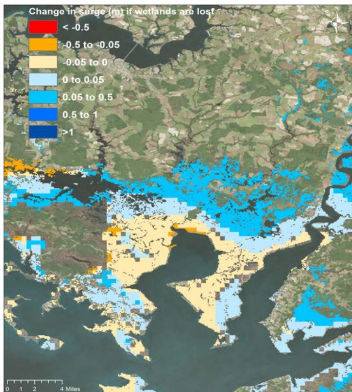
Figure 8: Wetlands can increase surge heights. A comparison of surge heights within wetlands for “Present” and “Wetland Loss” scenarios in Chesapeake Bay. Here, flood waters ‘pile up’ in the wetlands in front and are reduced behind them. Areas in orange experienced higher surge and areas in blue had lower surge heights.
