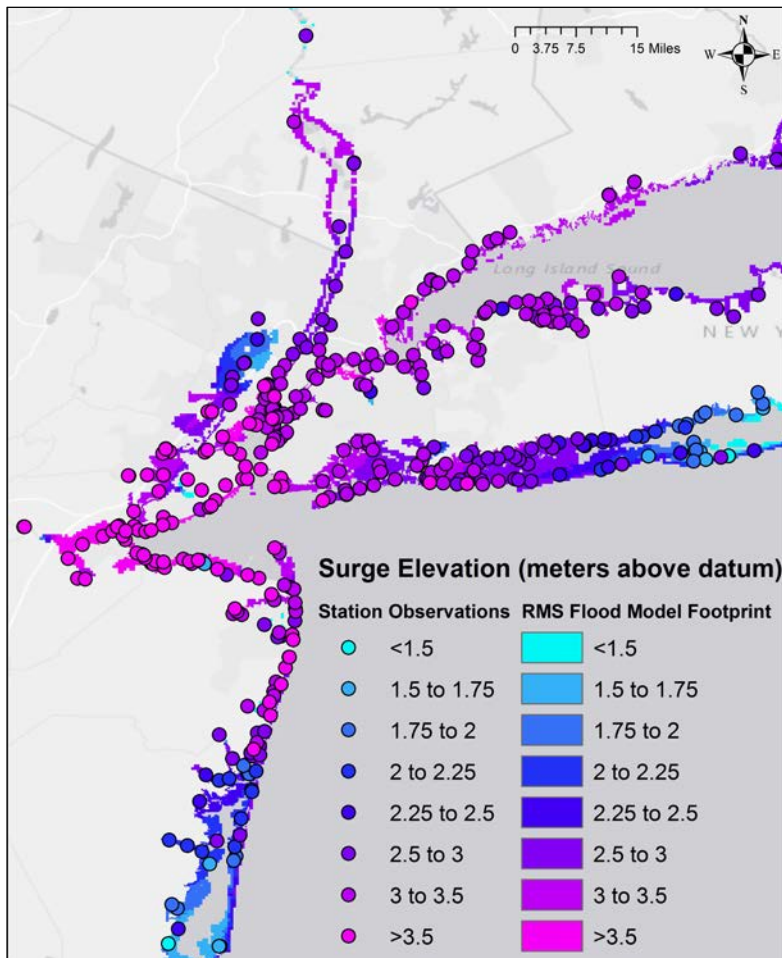
Figure 1: Flood model validation. Observed and predicted flood heights from Hurricane Sandy (here shown for parts of for New York and New Jersey). Station observations for the Sandy surge event were obtained from multiple sources (National Oceanic and Atmospheric Administration, 2012; US Geological Survey, 2012a, 2012b) and compared to the outputs from the RMS flood model.
