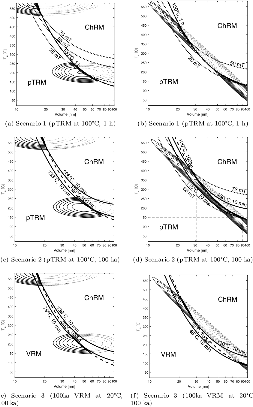
Fig. 7. Plots showing the magnetic moment m_r carried by each set of grains (given by their volume V and titanium content / Curie temperature T_c ) for a bimodal distribution. The dashed lines indicate the blocking condition for the acquisition time and temperature of the respective scenarios; the black lines indicate the blocking condition for the timescale of the demagnetization experiment; the dotted lines indicate the peak AF fields \tilde{H} needed to remove the magnetization.
