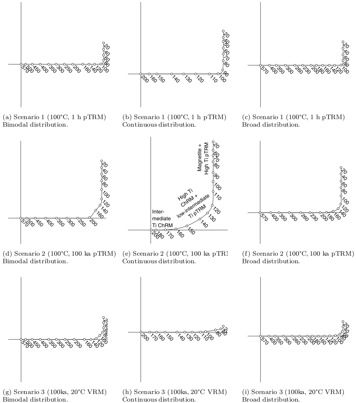
Fig. 3. Vector demagnetization (Zijderveld, 1967) plots for stepwise thermal demagnetization. Temperatures are given in °C. Fig. 3e is annotated to highlight behaviors occurring in all scenario 2 simulations.
