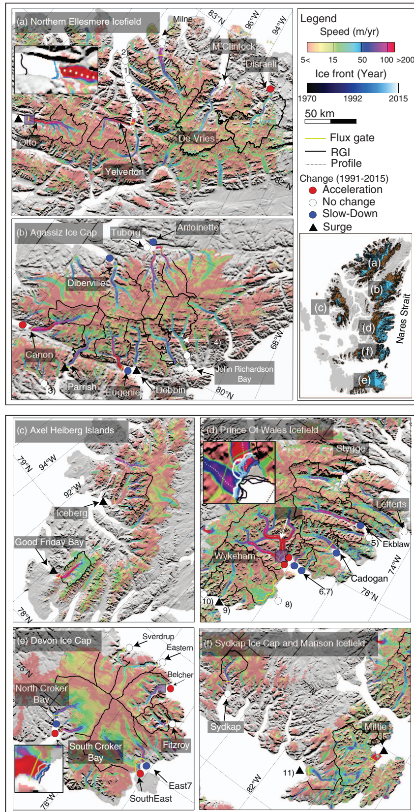
Figure 1. Flow speed of the QEI glaciers averaged between 1991 and 2015, color coded on a logarithmic scale, and overlaid on the CDED DEM in shaded relief. The survey domain is divided into 6 regions: (a) Northern Ellesmere Icefield, (b) Agassiz Ice Cap, (c) Axel Heiberg Islands, (d) Prince of Wales Icefield, (e) Devon Ice Cap, and (f) Sydkap Ice Cap and Manson Icefield. A full map of the QEI with CDED DEM in shaded relief is shown with the position of Nares Strait. Blue basins represent the drainage basins of marine-terminating glaciers and brown basins represent the drainage basins of land-terminating glaciers. Operation IceBridge (OIB) flight tracks are yellow, center flow lines are dash white, flux gates are yellow, and Randolph Glacier Inventory basin boundaries are black. Insets in (a), (d) and (e) show ice front positions of marine-terminating glaciers color coded from black, to blue and white from 1970 to 2015 for (a) Otto Glacier, (d) Trinity and Wykeham glaciers, and (e) Belcher Glacier. Glacier names are provided for major outlet glaciers. Red circles denote glacier acceleration. White circles denote no change in speed. Blue circles denote a slow down in speed during the period 1991 to 2015. Surging glaciers during the 1991–2015 time period are denoted with a black triangle.
