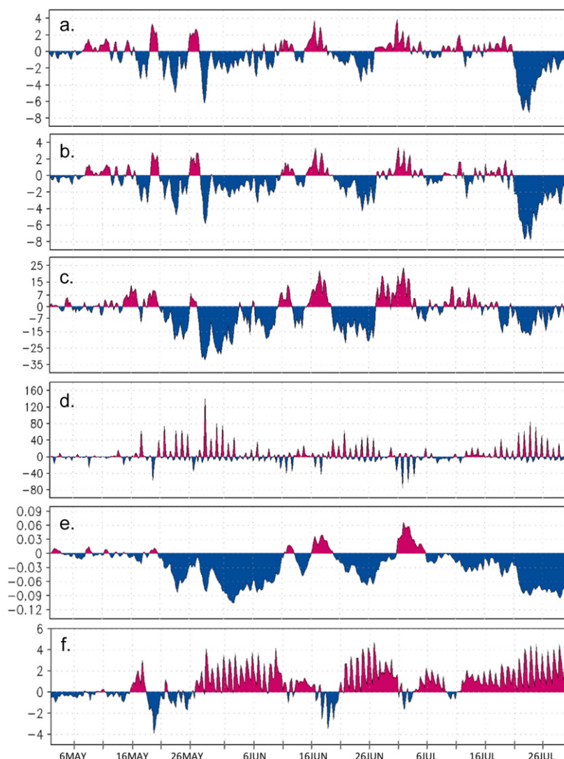
Figure 7. Time series of difference between Case 2011 and Case SUBT averaged over the SGP for (a) vertical integrated moisture flux divergence [ \text{mm day}^{-1} ], (b) precipitation [ \text{mm day}^{-1} ], (c) cloud cover [%], (d) net radiation [ \text{W m}^{-2} ], (e) soil wetness, and (f) surface temperature [ ^{\circ}\text{C} ].
