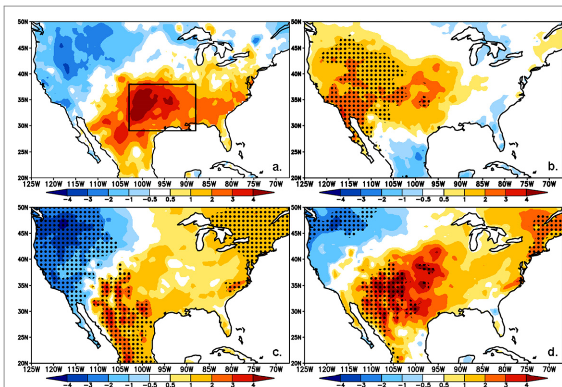
Figure 4. Observed/WRF simulated anomaly/difference of surface temperature ( ^{\circ}\text{C} ) for June. (a) Observed, (b) SUBT effect, (c) SST effect, and (d) SST effect plus SUBT effect. The dotted areas denote statistical significance at the \alpha = 0.01 level of t-test values.
