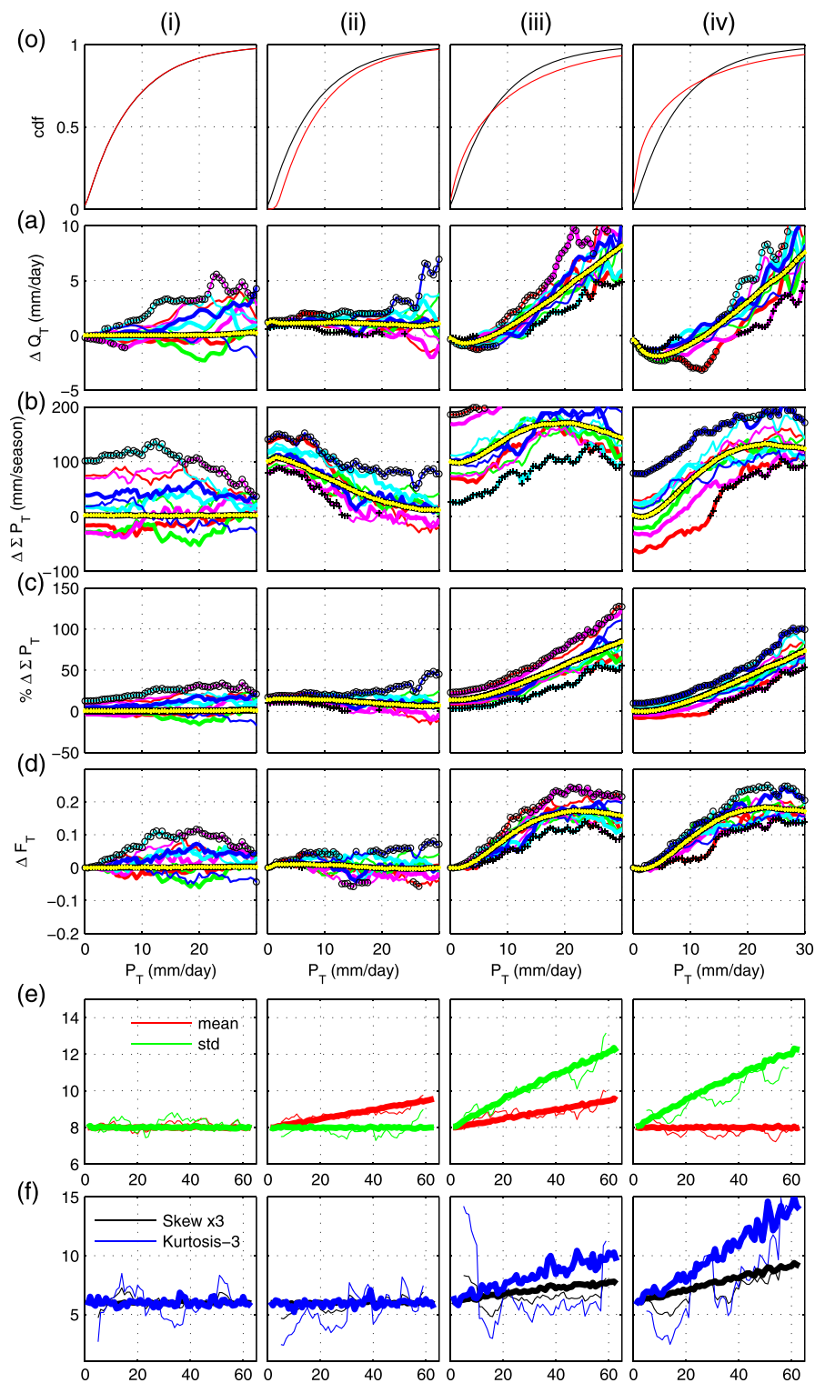
Figure 1. Idealized climate change with limited data and with almost perfect knowledge. (o) Cumulative distribution functions at the beginning (black) and end (red) of the illustrative 63 year period for (i) a constant distribution, (ii) increasing mean only, (iii) increasing mean, variance, skew and kurtosis, and (iv) increasing variance, skew and kurtosis. (a) Solid lines coloured blue through magenta plot ten samples of change in quantile, \Delta Q_T , over moving 45 year periods (from the middle of season within year 5 to the middle of the same season within year 50, 6 to 51, ..., 14 to 59) within the 63 year timeseries, where each year's distribution is represented by 9 years of data (for year t this includes years t - 4 to t + 4 —see appendix) and each year contains 90 samples from its underlying distribution. This is analogous to looking at a real-world timeseries built from one season/year. The bold yellow line shows the change between years 9 and 54 (a central sample) but taking each year's distribution as represented by 100 000 samples from its underlying distribution—also see SI figure 1. Rows (b), (c), and (d), are as (a) but for the climate change descriptors: (b) \Delta \Sigma P_T , (c) relative \Delta \Sigma P_T , and (d) \Delta F_T . Plots (o)–(d) are functions of daily precipitation threshold ( P_T ). Largest and smallest changes of consistent sign (see appendix) are marked with circles and crosses respectively. Rows (e) and (f) show the time-dependence of the mean (red), standard deviation (green), skew (black) and kurtosis (blue) for the well-sampled case (bold lines) and the realistically sampled case (standard lines).
