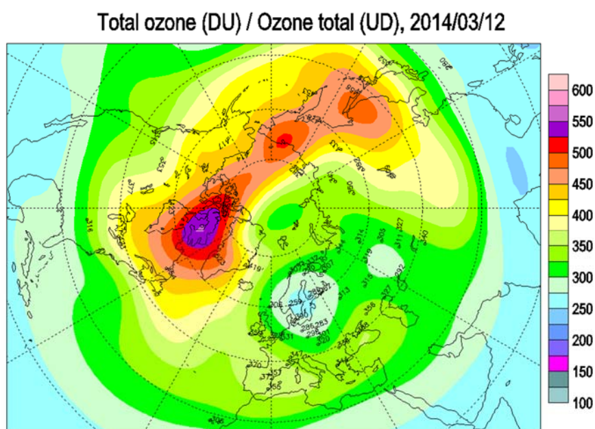
Figure 8: Total ozone from WOUDC and Environment Canada 12. March 2014. The map is based on ground based measurements and satellite observations ( http://exp-studies.tor.ec.gc.ca/e/ozone/Curr_allmap_g.htm )
