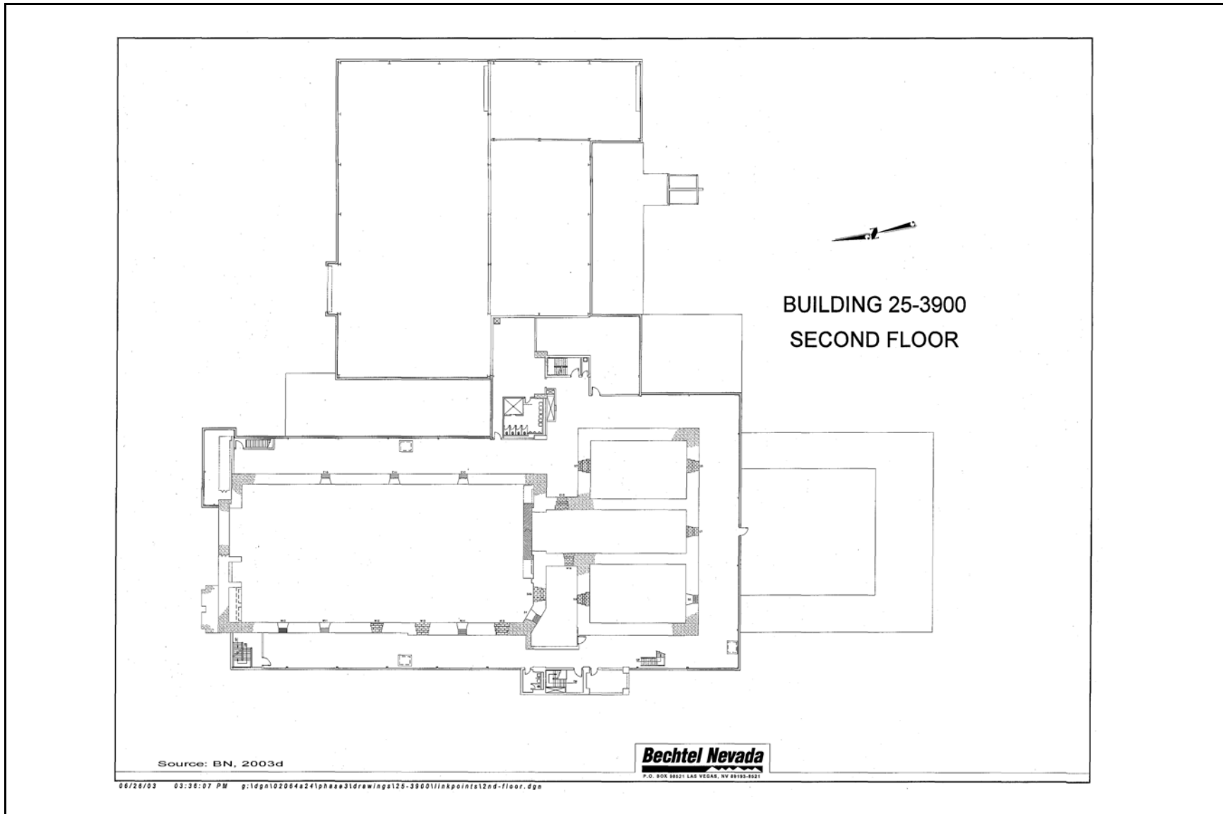
Figure 2-2 E-MAD Facility Second-Floor Layout
