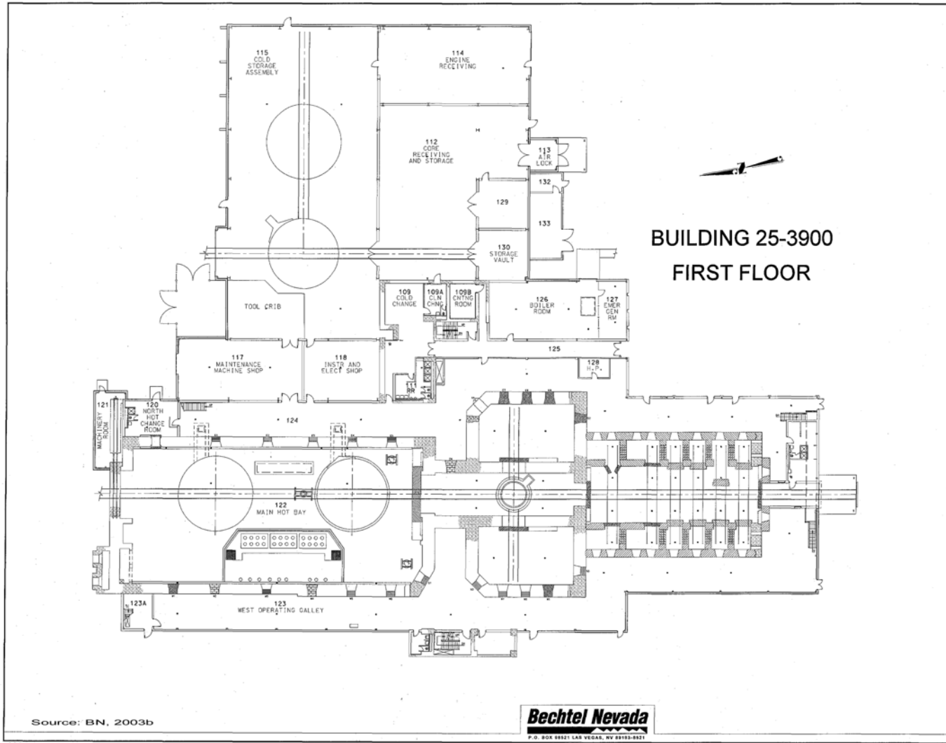
Figure 2-1 E-MAD Facility First-Floor Layout
