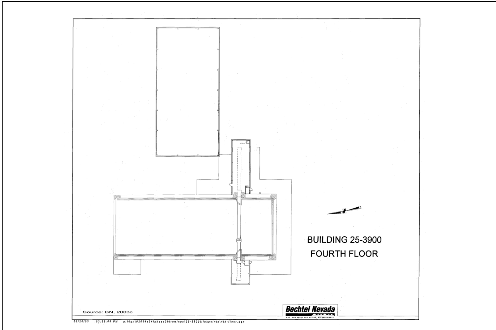
Figure 2-4 E-MAD Facility Fourth-Floor Layout
