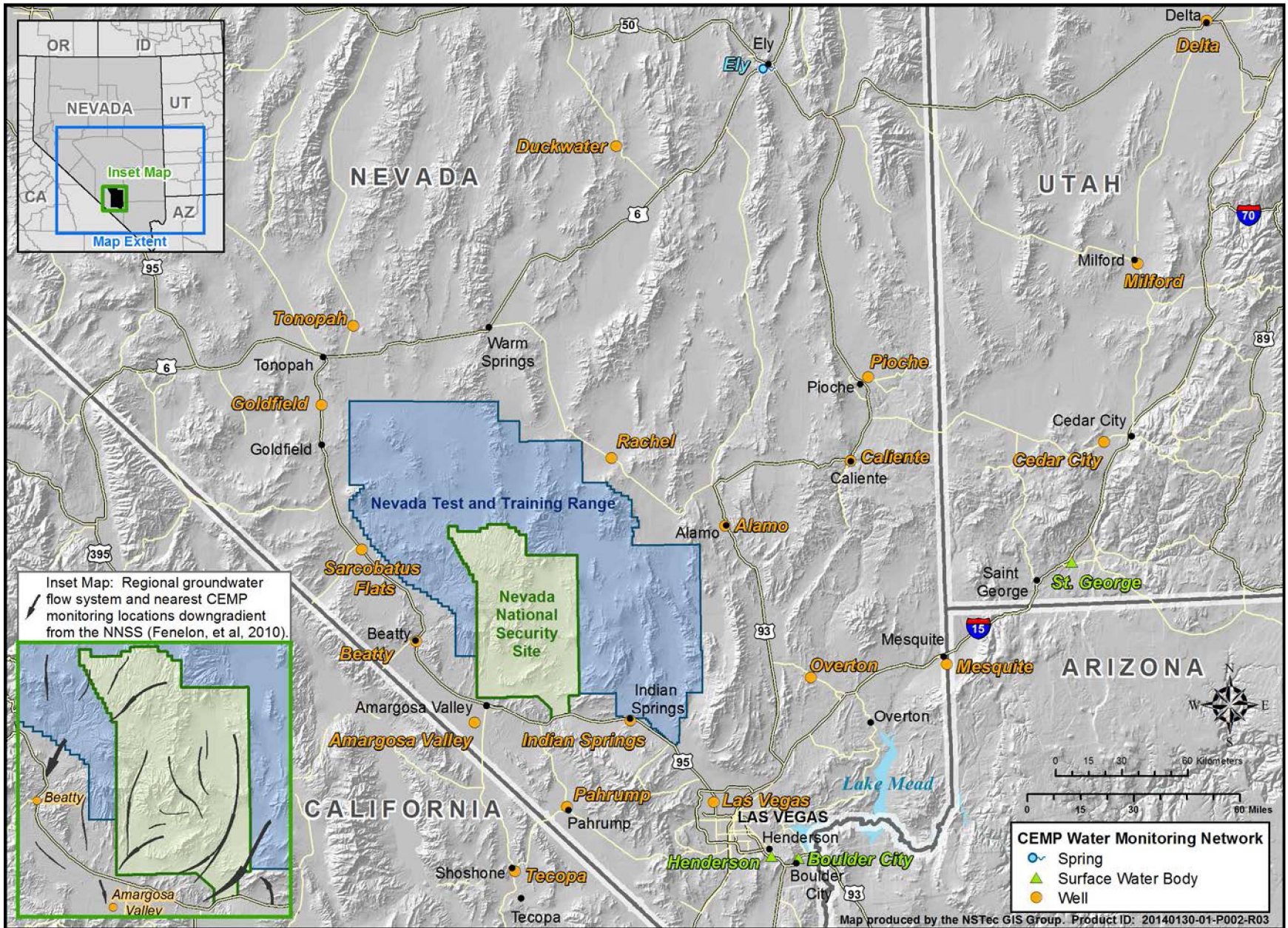
Figure 7-7. 2013 CEMP water monitoring locations
