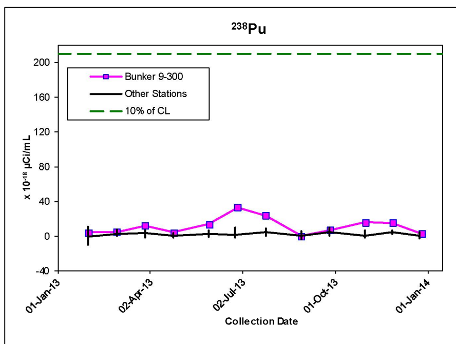
Figure 4-4. Concentrations of ^{238}\text{Pu} in air samples collected in 2013
