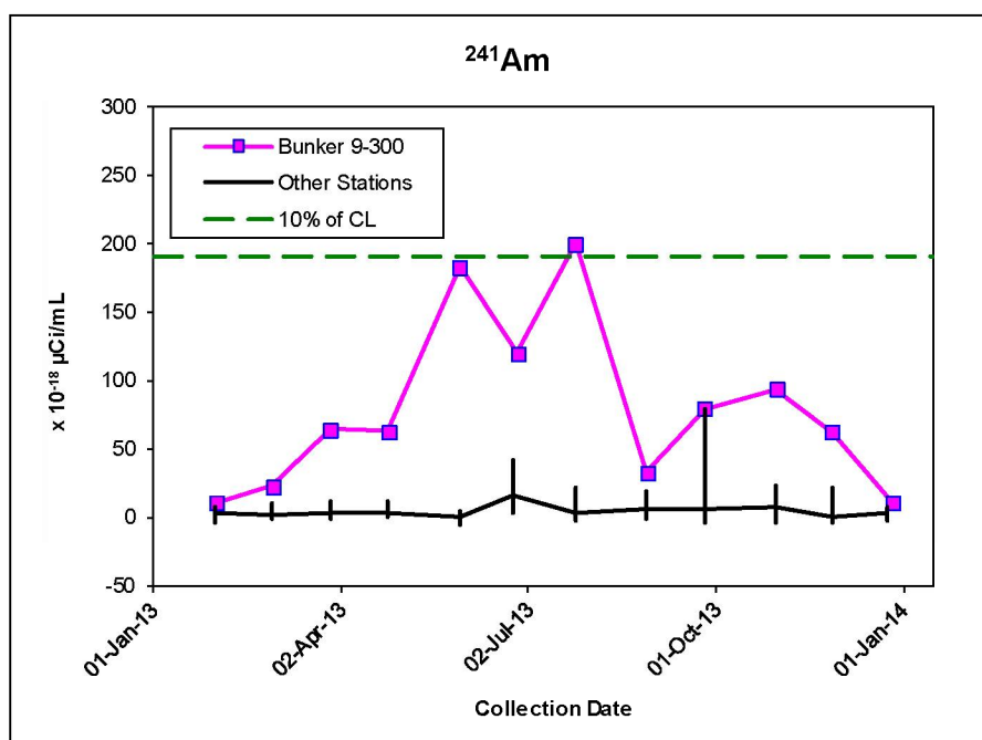
Figure 4-3. Concentrations of ^{241}\text{Am} in air samples collected in 2013
