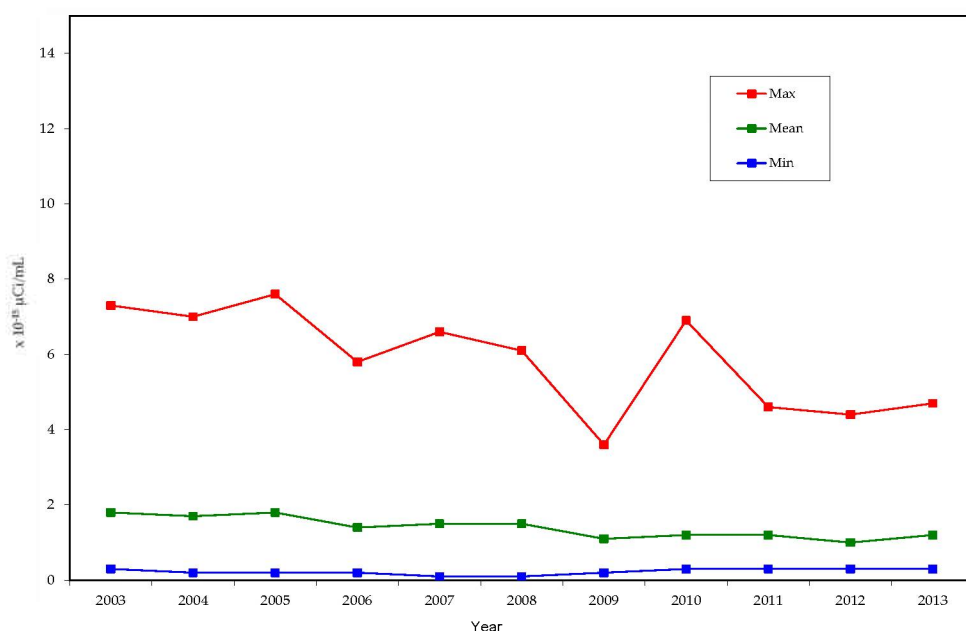
Figure 7-3. Historical trend for gross alpha analysis for all CEMP stations
