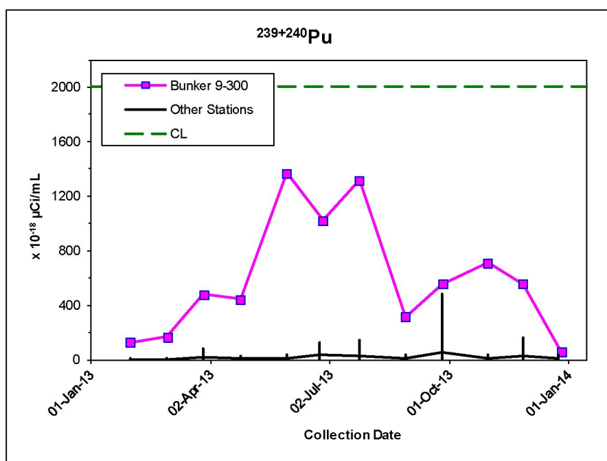
Figure 4-5. Concentrations of ^{239+240}\text{Pu} in air samples collected in 2013
