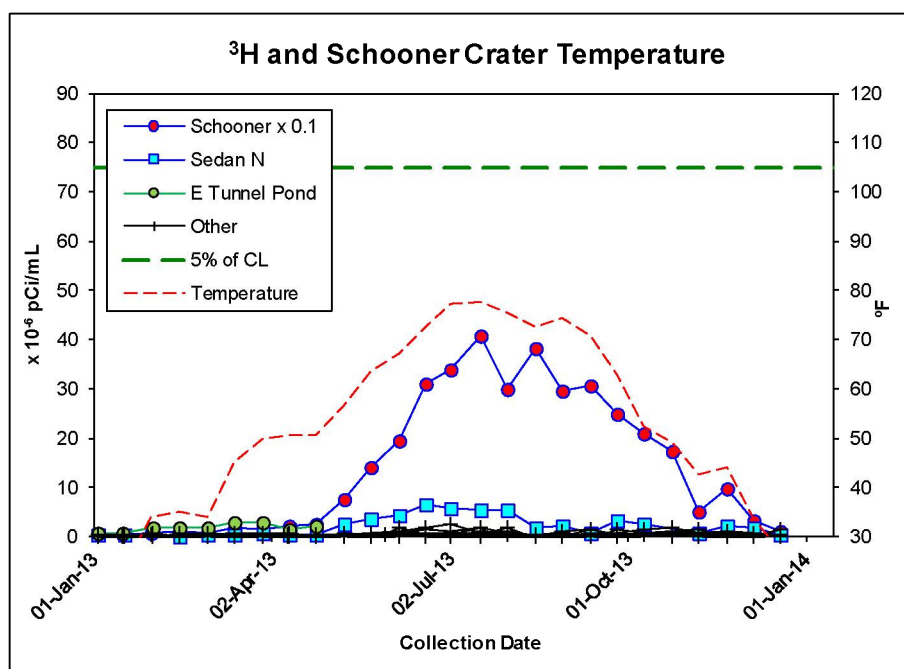
Figure 4-7. Concentrations of ^3\text{H} in air samples collected in 2013 with Schooner Crater average air temperature per collection period
