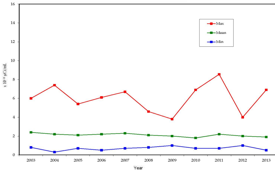
Figure 7-4. Historical trend for gross beta analysis for all CEMP stations
