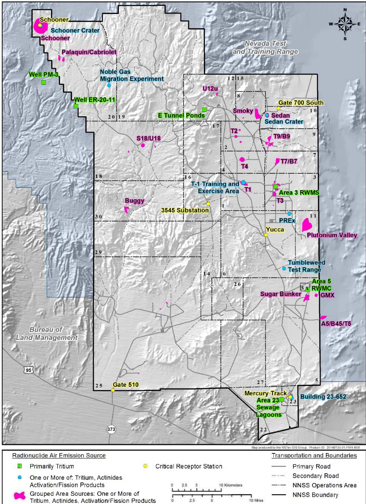
Figure 4-1. Sources of radiological air emissions on the NNS in 2013
