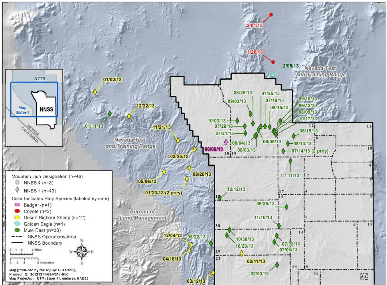
Figure 15-3. Kill sites of two radio-collared mountain lions documented in 2013
