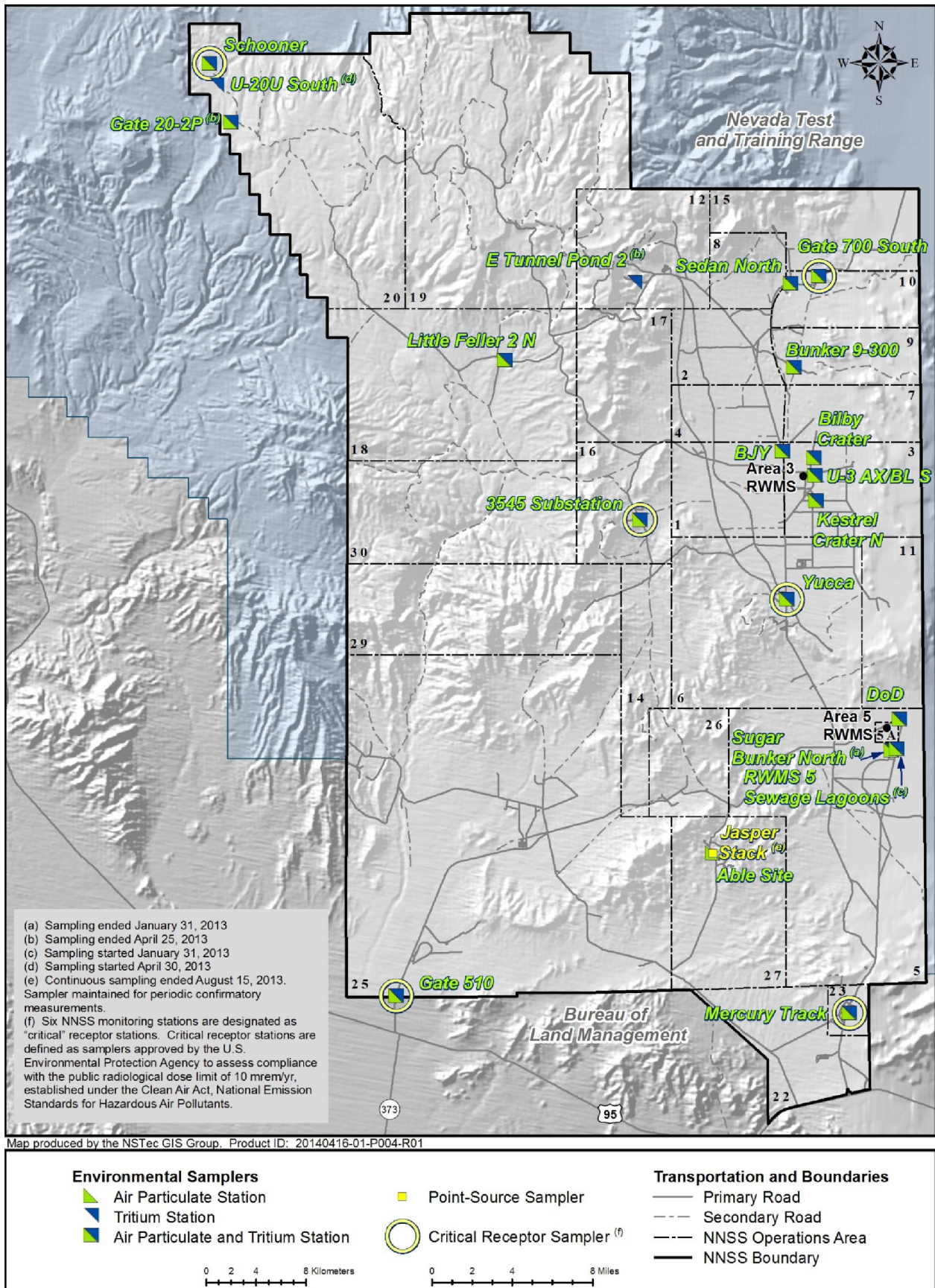
Figure 4-2. Radiological air sampling network on the NNSS in 2013
