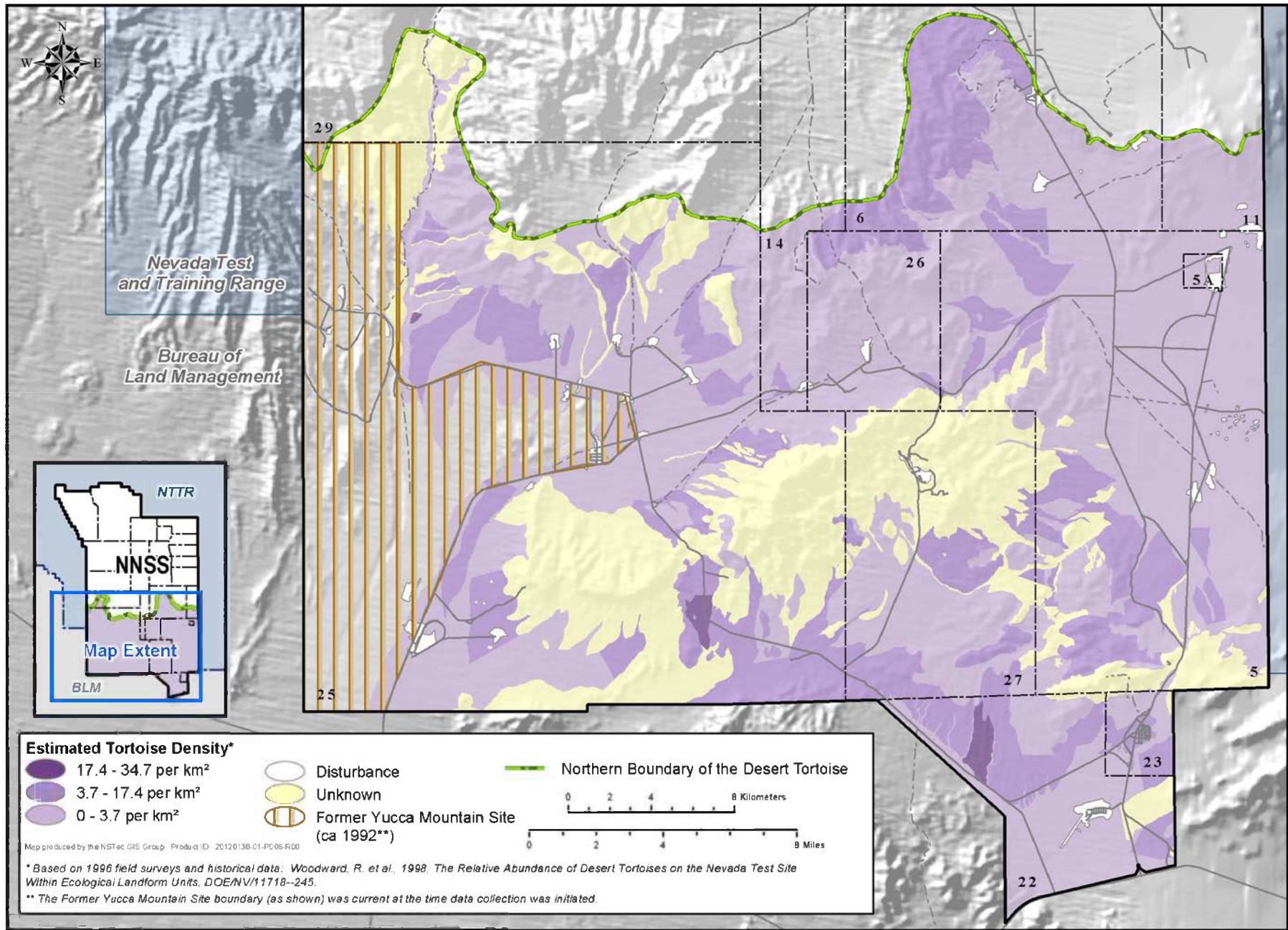
Figure 15-1. Desert tortoise distribution and abundance on the NNSS
