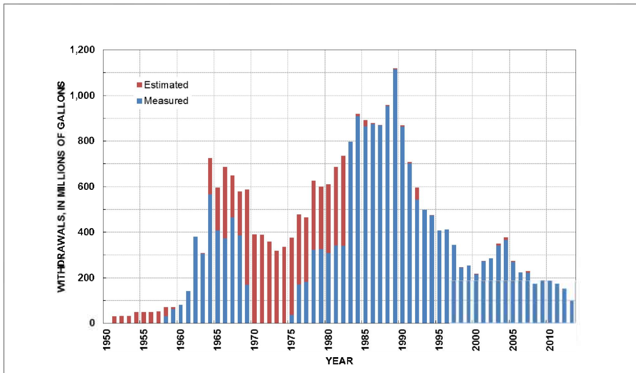
Figure 13-1. Annual withdrawals from the NNSS, 1951 to 2013
