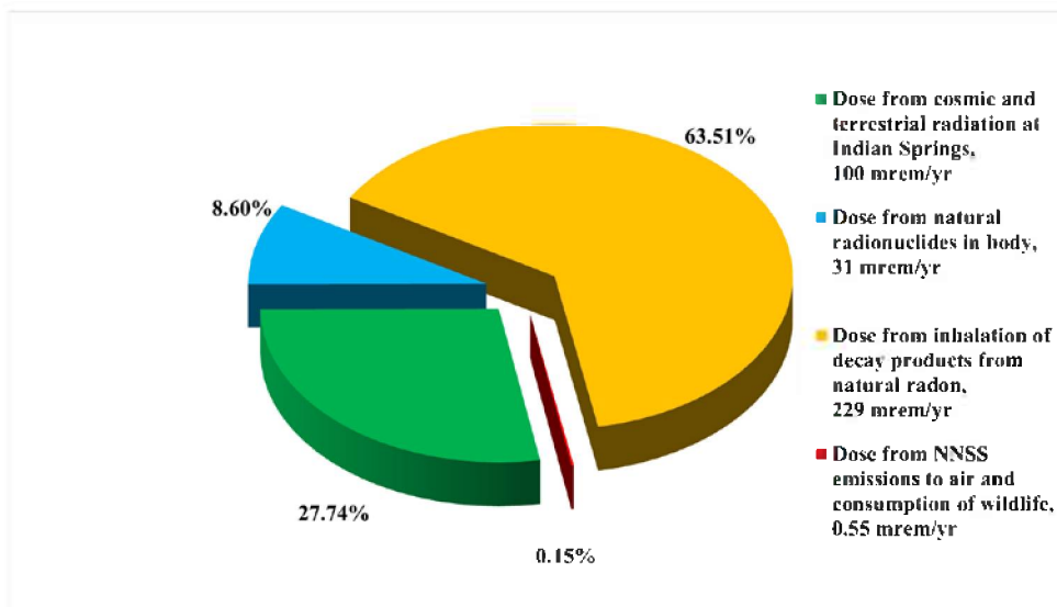
Figure 9-1. Comparison of radiation dose to the MEI from the NNSS and natural background (percent of total)
