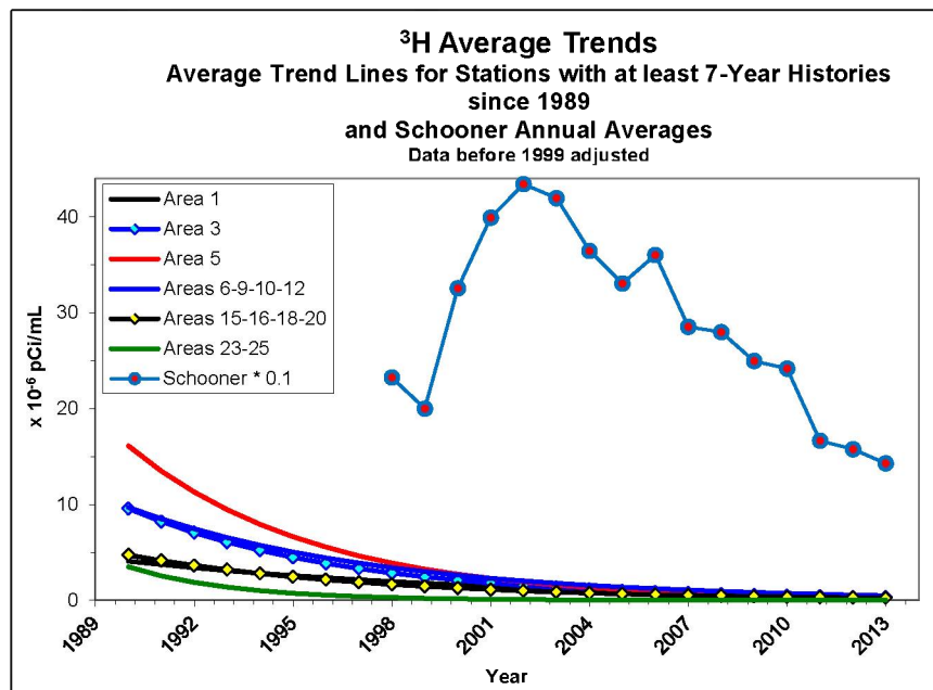
Figure 4-9. Trends in annual mean 3 H air concentrations for Area groups and Schooner Crater annual means, 1990–2013
