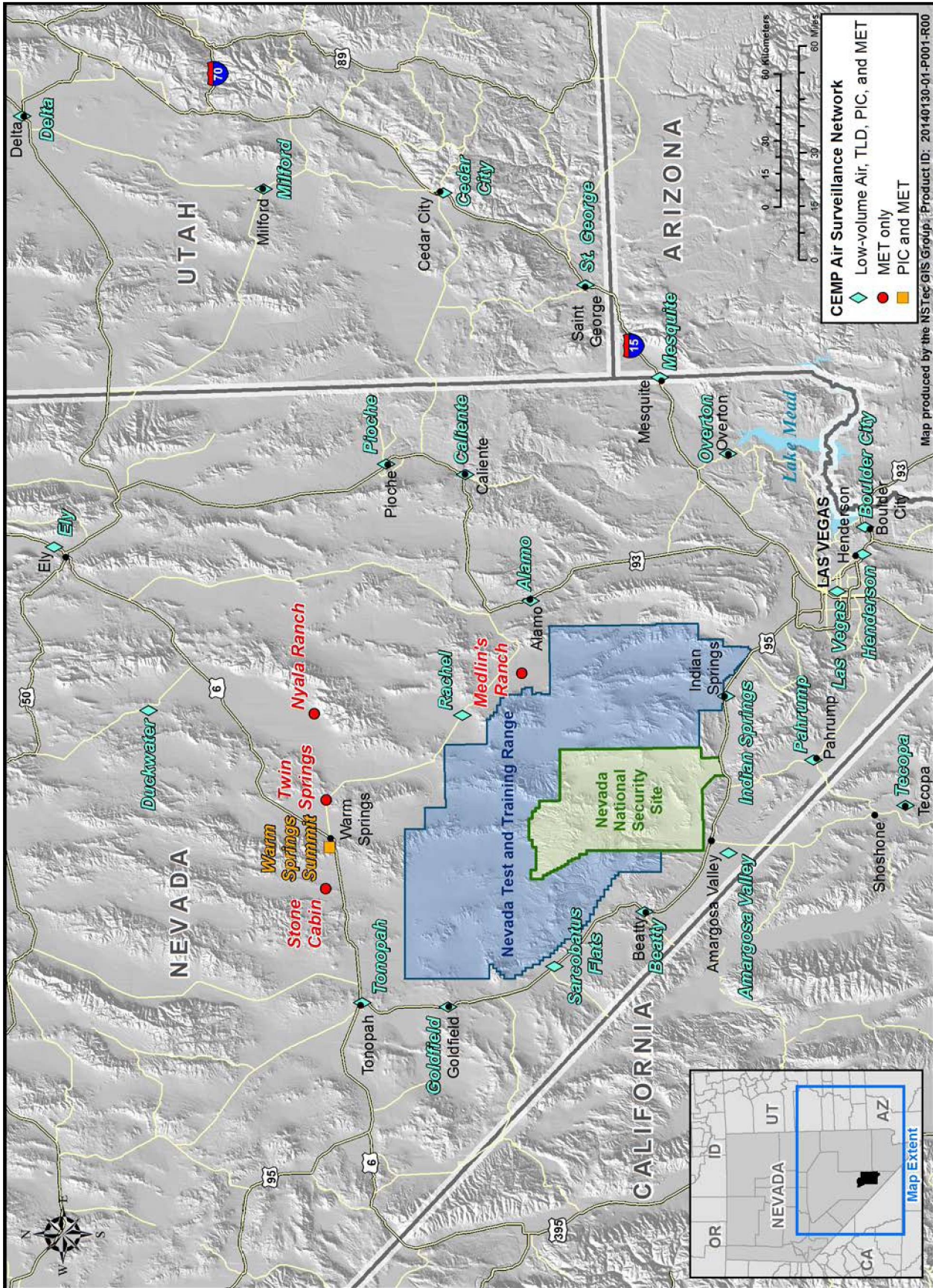
Figure 7-1. 2012 CEMP Air Surveillance Network
