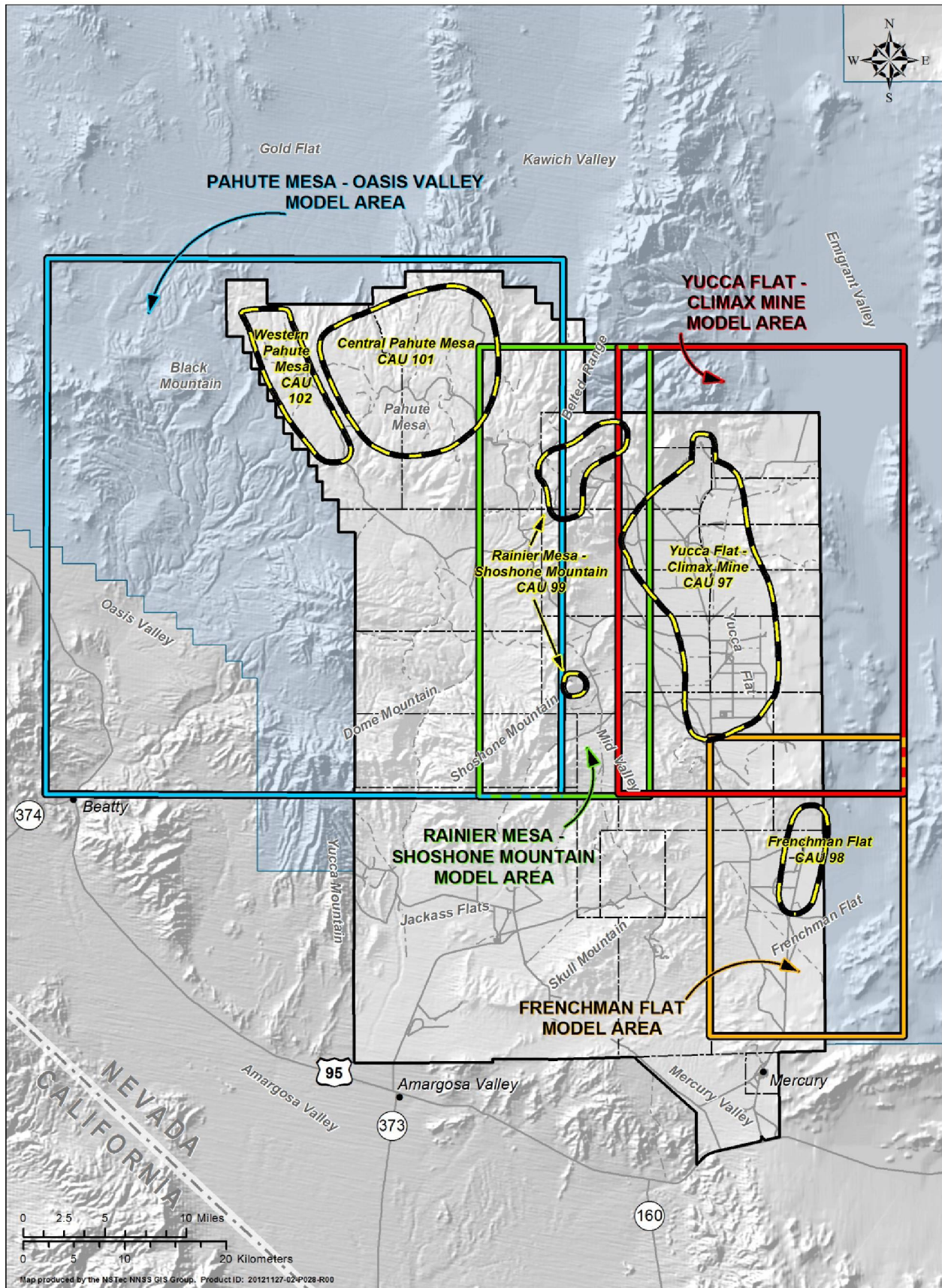
Figure 11-2. Location of UGTA model areas
