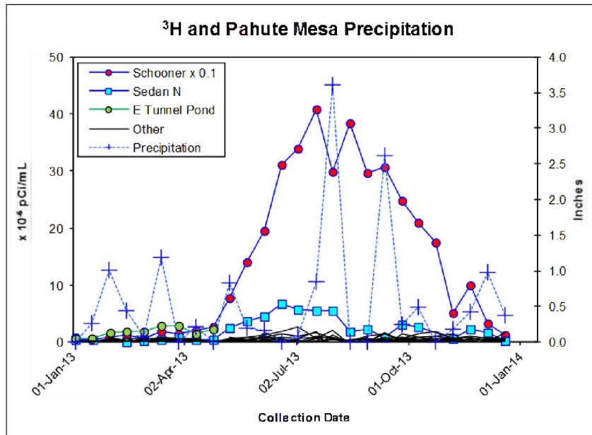
Figure 4-8. Concentrations of 3 H in air samples collected in 2013 with Pahute Mesa precipitation
