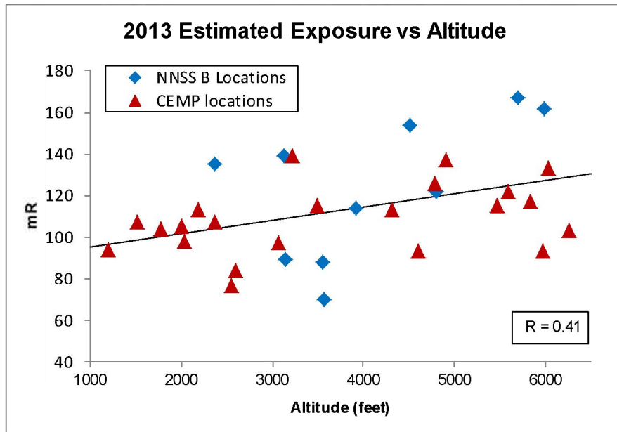
Figure 6-3. Correlation between 2013 annual exposures at NNSS Background and CEMP TLD locations and altitude
