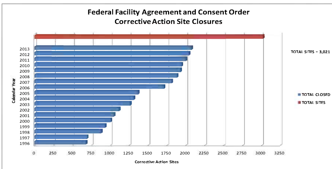
Figure 11-5. Annual cumulative totals of FFAO CAS closures
