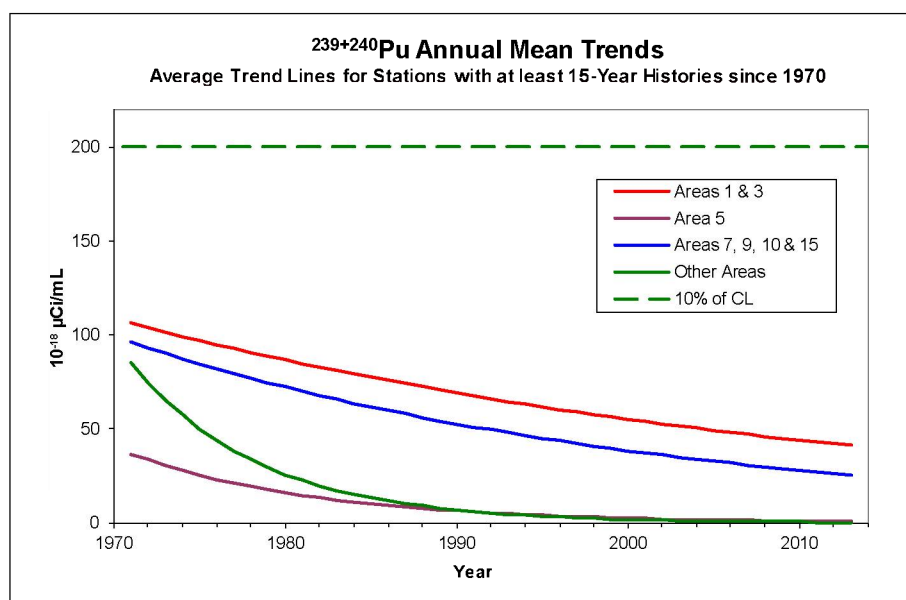
Figure 4-6. Average trends in ^{239+240}\text{Pu} in air annual means, 1971–2013
