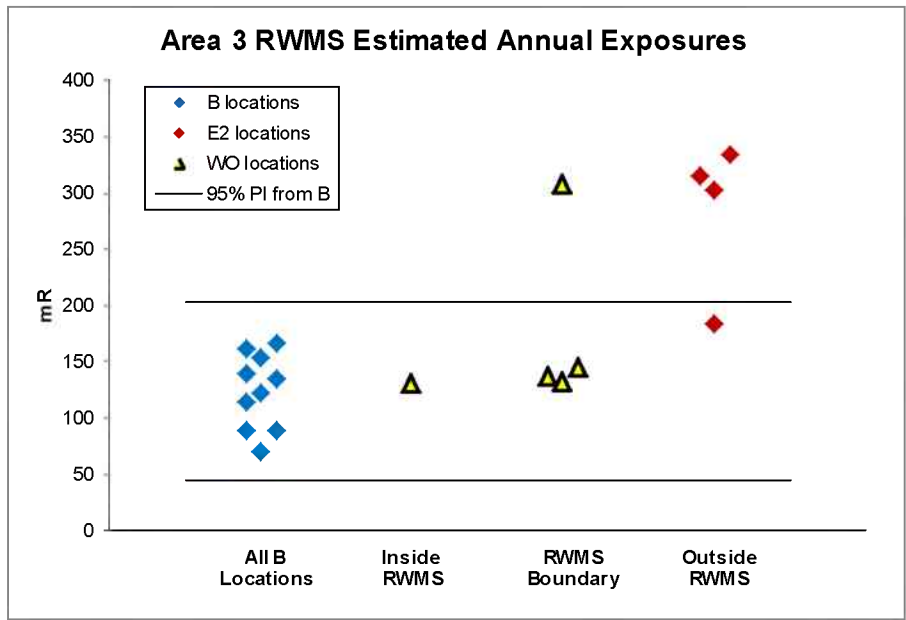
Figure 6-4. 2013 annual exposures in and around the Area 3 RWMS and at background locations
