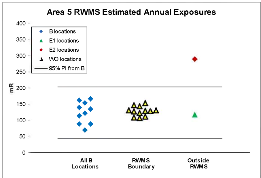
Figure 6-5. 2013 annual exposures around the Area 5 RWMS and at background locations
