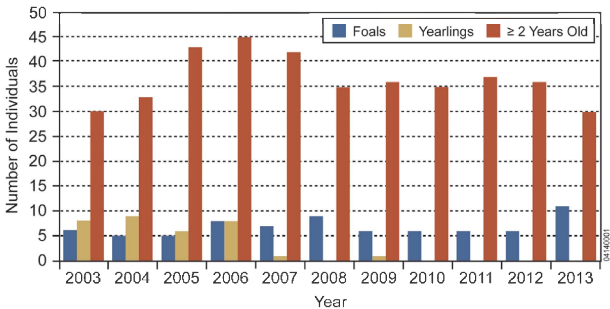
Figure 15-4. Trends in age structure of the NNSS horse population from 2003 to 2013
