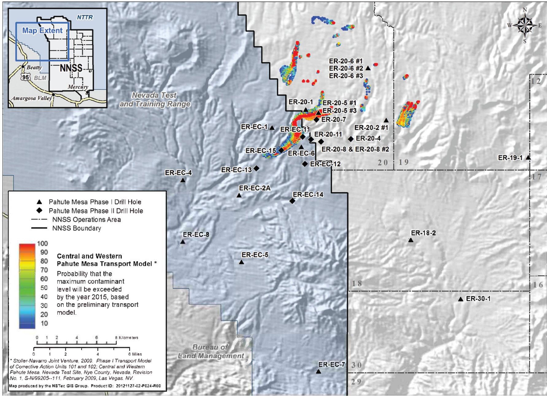
Figure 11-4. Results of Phase I Central and Western Pahute Mesa Transport Modeling
