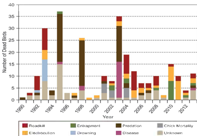
Figure 15-2. Number of bird deaths recorded on the NNSS by year and cause
