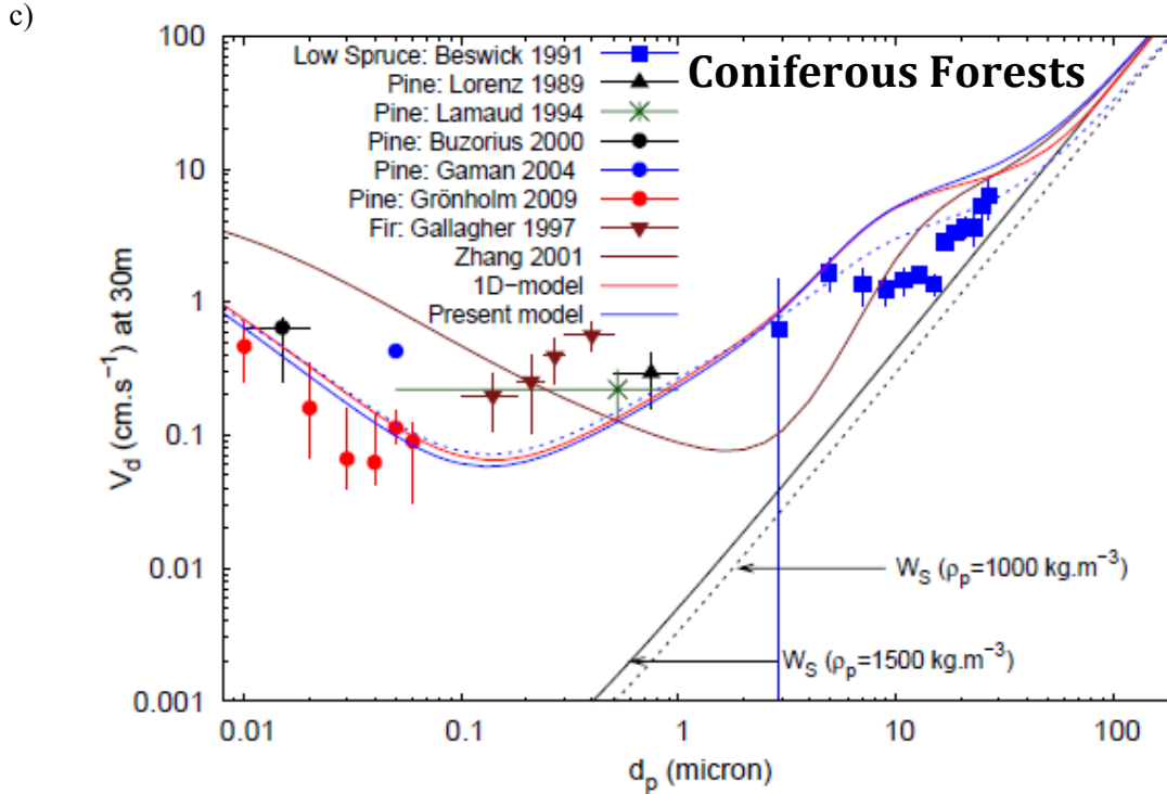
Figure 3-2. Dependence of deposition velocity on particle diameter for smooth soil (a), grass (b) and coniferous forests (c). Gravitational settling is shown by the w_s curve. Petroff and Zhang (2010) model results are labeled with solid lines labeled (a) “Present model leaf” (b) and “Present model” (c). Symbols show measured values with uncertainty ranges shown as line segments. Graphics reproduced from Figures 3, 4, and 5 (Petroff and Zhang, 2010).
