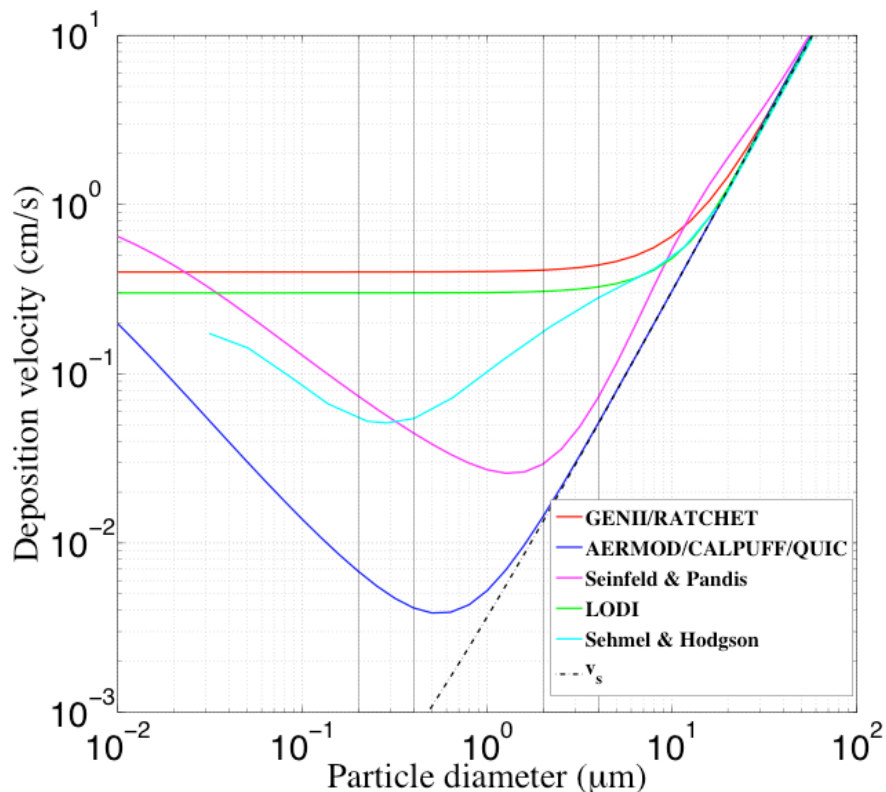
Figure 4-1. Deposition velocity (cm/s) as a function of particle diameter ( \mu\text{m} ) and choice of deposition (resistance) model formulations for several representative models and 1 m/s winds, stability class F, and a surface roughness length of 1 cm.
