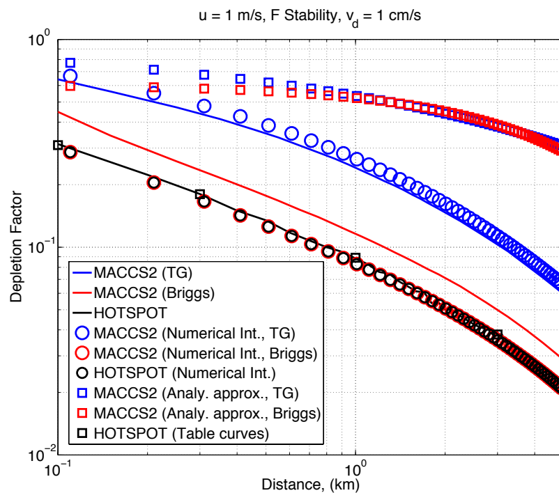
Figure 5-1. Depletion factors for Hotspot and MACCS 2 ( u= 1\text{ m/s} , v_d= 1\text{ cm/s} . F stability)
