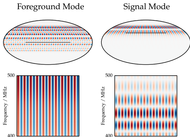
FIG. 6. Here we plot two KL-modes (with m = 20 ) as they would look on the sky: one of the most foreground like modes ( S/F = 4 \times 10^{-13} ); and one of the most signal like modes ( S/F = 170 ). Though they are derived in visibility space, when projected back to the sky, they appear as we would expect with the foreground mode having a smooth frequency spectrum, and the signal mode oscillating. Modes at either end of the spectrum, like the ones plotted are easy to interpret, this is not generally true of the intermediate modes.
