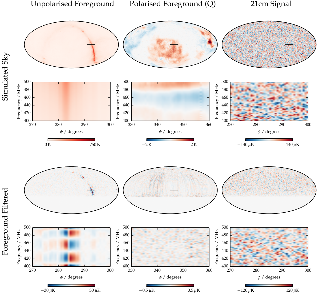
FIG. 8. This plot illustrates the process of foreground removal on simulations of the radio sky. The top row of plots show skymaps of the individual components: unpolarised foregrounds, polarised foregrounds (showing Stokes Q only), and the 21 cm signal. On the bottom row we show the maps we would make after foreground cleaning visibilities from our example telescope. Both the polarised and unpolarised foregrounds become substantially suppressed, whereas the 21 cm signal is largely unaffected. In this example we have discarded modes with S/F < 10 . This leaves a clear correspondence between the original signal simulation and the foreground subtracted signal, whilst leaving the foreground residuals over 10 times smaller in amplitude.
