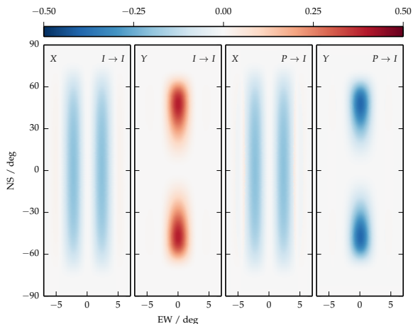
FIG. 11. The response of the primary beam to fractional changes in the X and Y dipoles E-plane widths. Similar to Figure 2 we illustrate the transfer from the total intensity and polarised sky, into an instrumental Stokes I combination, however, here we show the derivative with respect to changes in the E-plane width of the X and Y feeds. The first two plots show the change of the total intensity response with changes in the E-plane of the X and Y dipoles; the second two plots show the changes in the polarisation response, again corresponding to changes in the X and Y feeds. For instance a 1% change in each dipoles width changes each response by 1% of the corresponding plot (to first order).
