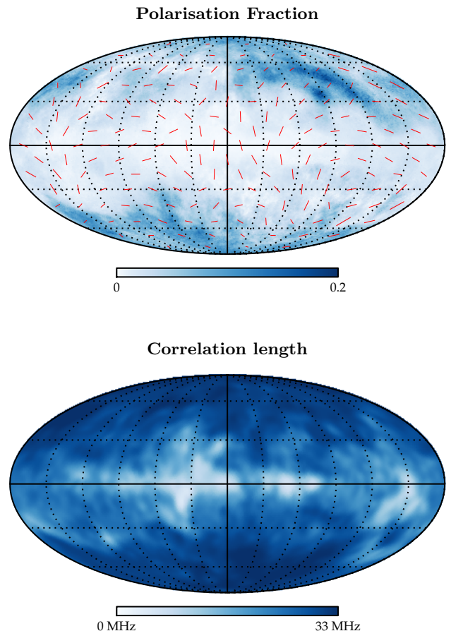
FIG. 16. The top figure shows the polarisation direction and fraction of the 600 MHz slice of a polarised simulation of the galaxy. This clearly demonstrates the effect of Faraday depolarisation towards the galactic centre. The lower plot shows the effective correlation length as measured across the sky, smoothed on 10^\circ scales.
