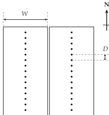
FIG. 1. A schematic of a cylinder telescope, consisting of two cylinders aligned North-South on the ground. Each cylinder is of width W , and has N_{\text{feeds}} regularly spaced a distance D apart. In this paper we will only consider cylinders which are touching, making the total width of the array 2W . The cylinders are assumed to be long enough that there are no optical differences between feeds at the edge and in the centre of the array.
