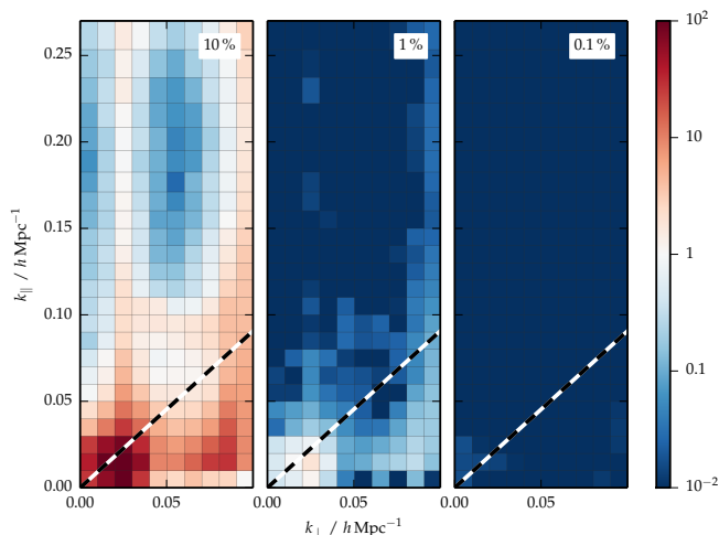
FIG. 10. Biasing of the power spectrum from complex gain perturbations with amplitude \sigma_g = 10\% , 1\% and 0.1\% , again for observations of 400–500 MHz. The bias is given as a fraction of the statistical error. Regions where this ratio is less than one (shown in blue) indicate where the systematic errors are sub-dominant compared to the statistical errors. Again we indicate the foreground wedge with a dashed line, however in this case we note that most of the bias lies within this region.
