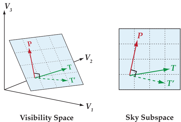
FIG. 4. The information about the sky does not spread throughout the space of visibilities but is contained in a subspace, a linear combination of the measured signals which does not span the whole visibility space. Directions orthogonal to this subspace are excited only by the instrumental noise, and contain no information about the sky. The left panel illustrates the geometry of the full visibility space, showing the sky subspace as a plane. In the right panel we show only the sky plane. Within this sky subspace, there are yet lower dimensional subspaces that the total intensity (labelled T ) and polarised ( P ) signals get mapped to. However, they need not be orthogonal, an effect we must take into account. One way of treating this is to project onto the space orthogonal to polarisation (labelled T' ), this eliminates polarised contamination at the expense of some sensitivity to total intensity. This is discussed in detail in the text.
