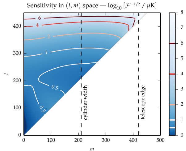
FIG. 3. Sensitivity of the array to temperature, derived from the inverse of the diagonal elements of the Fisher matrix (\mathcal{F}_{(lm)(lm)})^{-1} . The plot above shows the \log_{10} of the sensitivity in units of \mu\text{K} . The sensitivity to the three remaining Stokes parameters are largely identical. The dashed black lines mark the m corresponding to the separation between the cylinders, and the total width of the cylinders. As we would expect the sensitivity peaks in m at the zero separation, and the single cylinder separation. It then falls off rapidly at the edge of the telescope.
