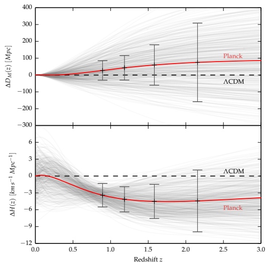
FIG. 14. Constraints on the expansion history as a function of redshift, shown relative to a fiducial \Lambda CDM cosmology. The redline shows the mean expansion history predicted from the Planck constraints on w_0, w_a [60] (combined with Union 2 supernovae data [61]), and the grey lines show a selection of histories randomly drawn from the posterior distribution. For a medium sized cylinder experiment, the best discrimination comes at low redshift from the 600–800 MHz bands.
