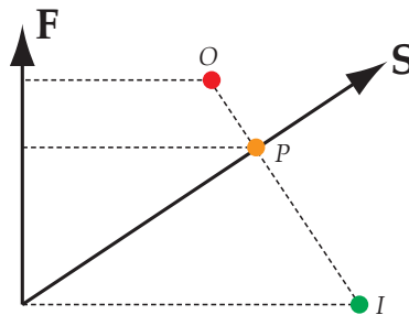
FIG. 7. To remove foregrounds from our data (point O ), we separate our space into two subspaces of foreground contaminated modes, and signal modes (denoted by \mathbf{F} and \mathbf{S} ). These spaces are not guaranteed to be orthogonal. Inverting with the pseudo-inverse, gives the linear combination of signal vectors with the same amplitude, however, the resulting vector P is clearly contaminated by foregrounds (as the projection onto \mathbf{F} is non-zero). The full-inverse gives point I , which has the same projection onto \mathbf{S} , but contains no foregrounds, however, it is necessarily a combination of both \mathbf{S} and \mathbf{F} .
