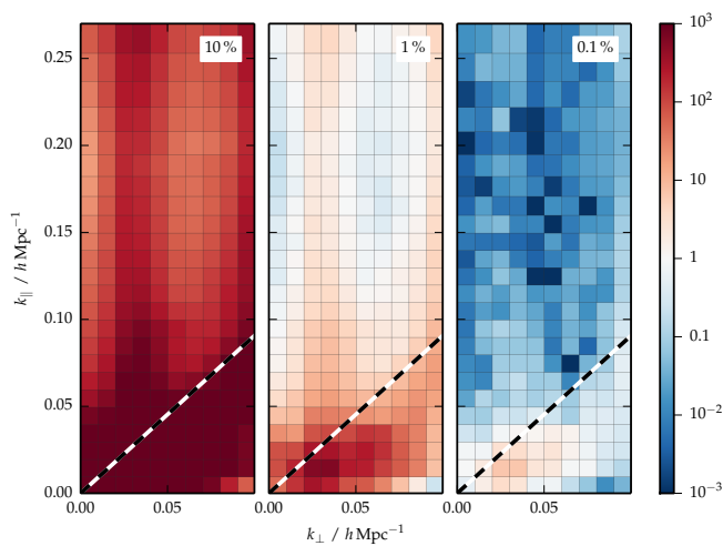
FIG. 12. Power spectrum biasing for 10%, 1% and 0.1% shifts from the fiducial E-plane width. These biases are given in units of \sigma for each band, values greater than one indicate where this systematic error dominates the statistical error. These are the biases of the Minimum Variance estimator (so as to avoid issues with the power spectrum deconvolution). Here we can see that unknown fluctuations in the beam width of more than 0.1% give rise to significant power spectrum biases.
