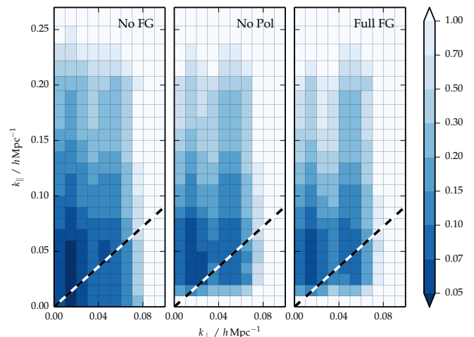
FIG. 9. Forecast errors on the power spectrum as a fraction of its fiducial value for the 400–500 MHz band. The three panels show the predicted errors without foregrounds (left), with unpolarised foregrounds (centre), and with fully polarised foregrounds (right). The dashed line indicated the predicted bound of the ‘foreground wedge’, showing that with perfect knowledge of our instrument foregrounds can be successfully cleaned well into this region.
