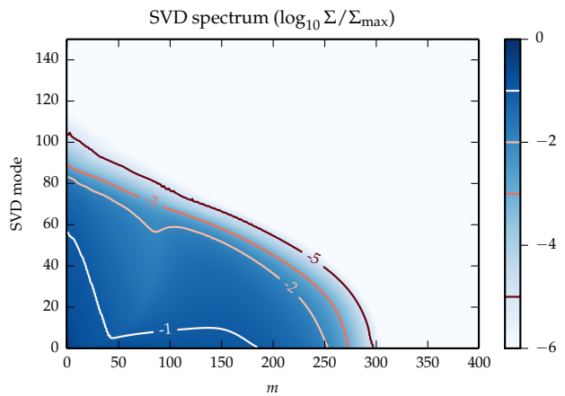
FIG. 5. The singular values of \bar{\mathbf{B}} for the 400 MHz channel after removal of the polarised modes. Large singular values represent modes on the sky that are well measured. We see that at each m there are less than 100 measured degrees of freedom from the sky, with the spectrum dropping off very steeply beyond this. This is a significant saving, before compression there are twice as many modes as there are unique baselines, including positive and negative m . In our example there are 762 unique baselines (without auto-correlations), so there would be \sim 1500 modes.
