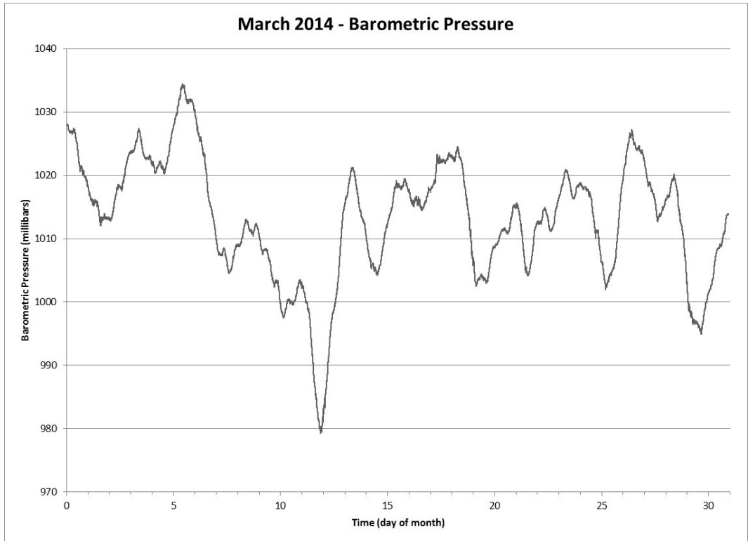
Figure 19 Barometric Pressure for the Month of March 2014
