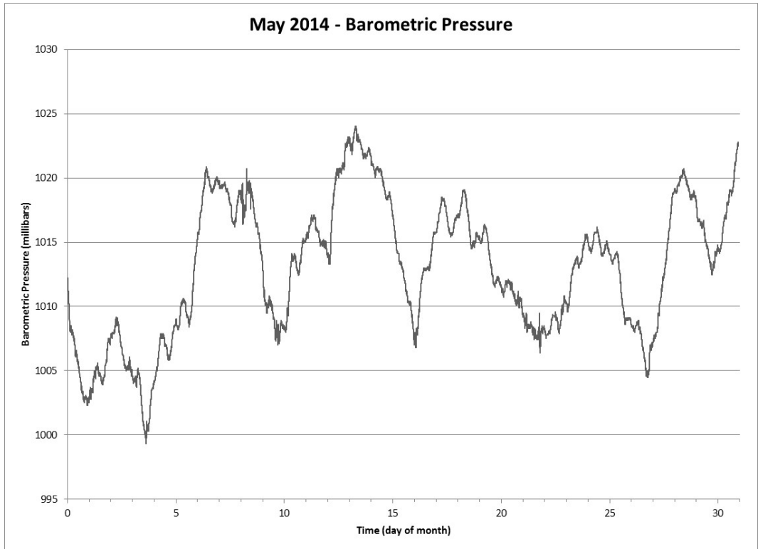
Figure 21 Barometric Pressure for the Month of May 2014
