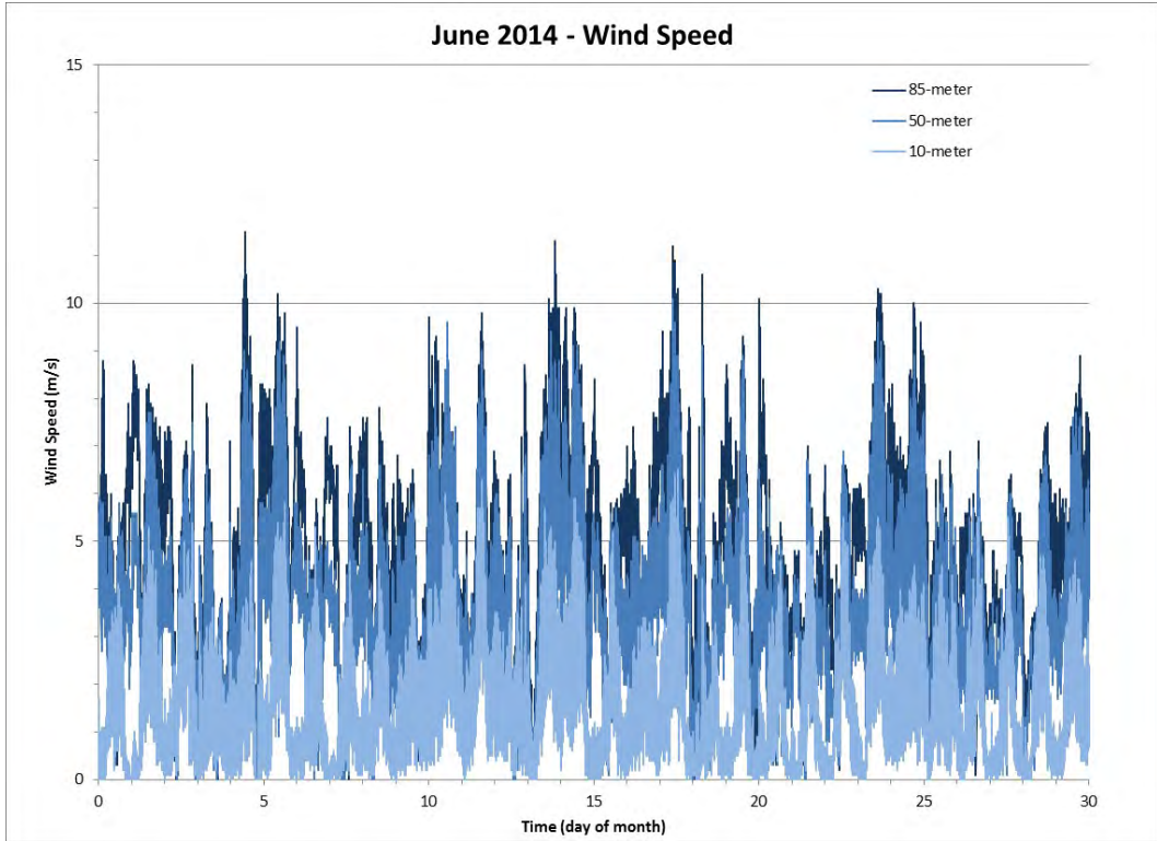
Figure 96 Wind Speed for the Month of June 2014
