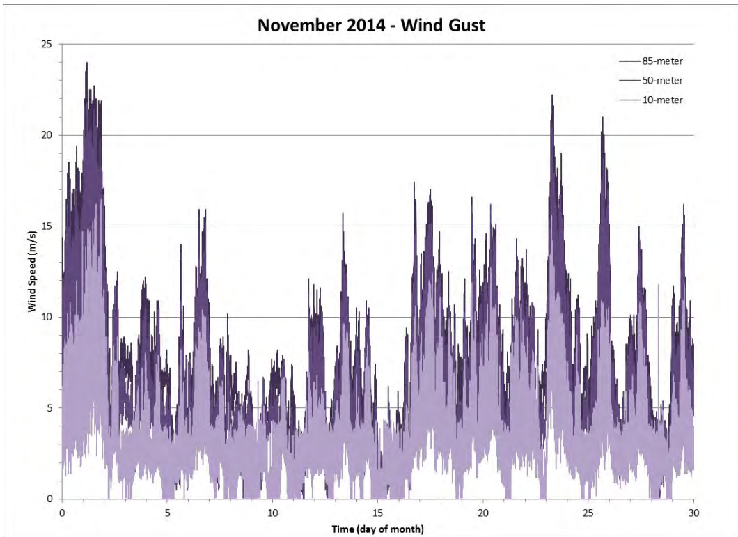
Figure 107 Wind Gust data for the Month of November 2014
