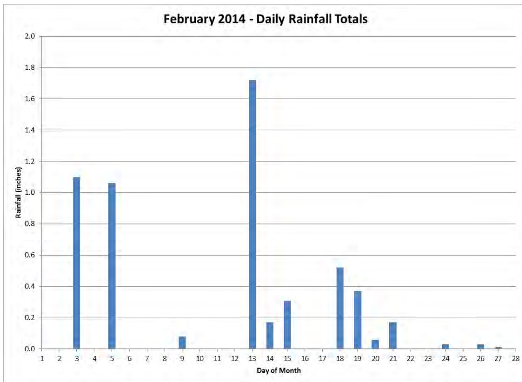
Figure 46 Daily Rainfall for the Month of February 2014
