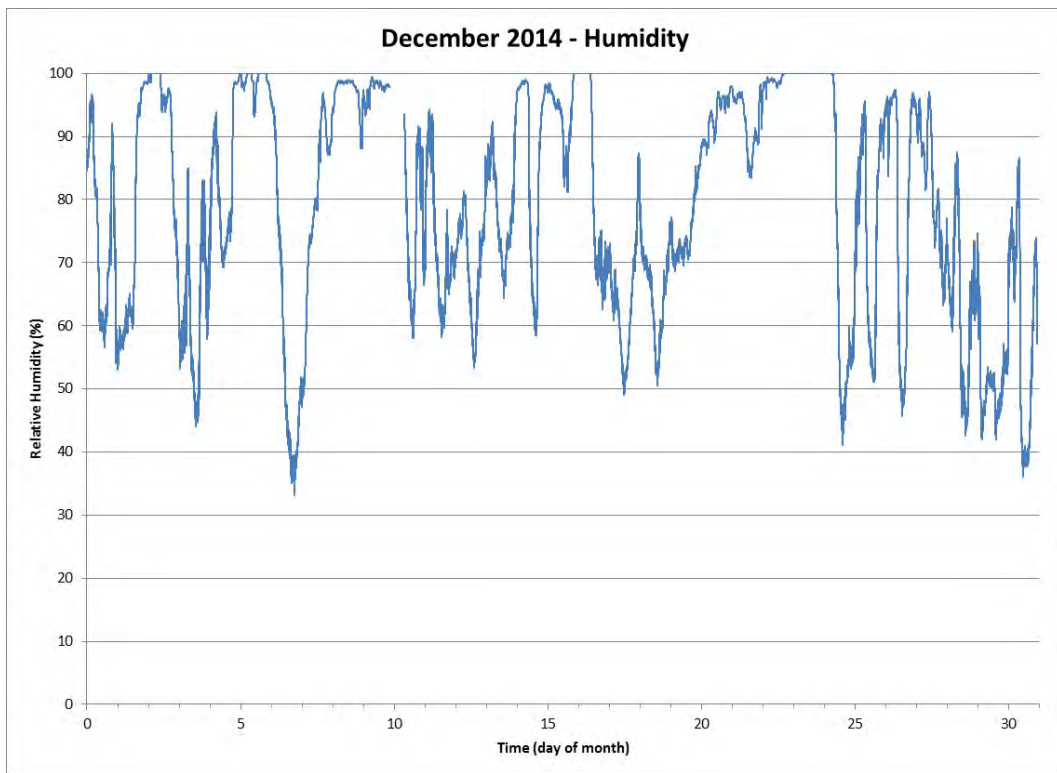
Figure 43 Relative Humidity for the Month of December 2014
