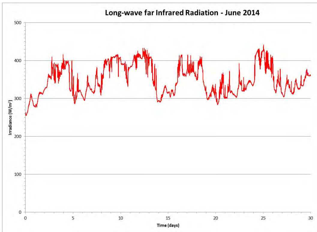
Figure 154 Long-wave Far Infrared Radiation for the Month of June 2014
