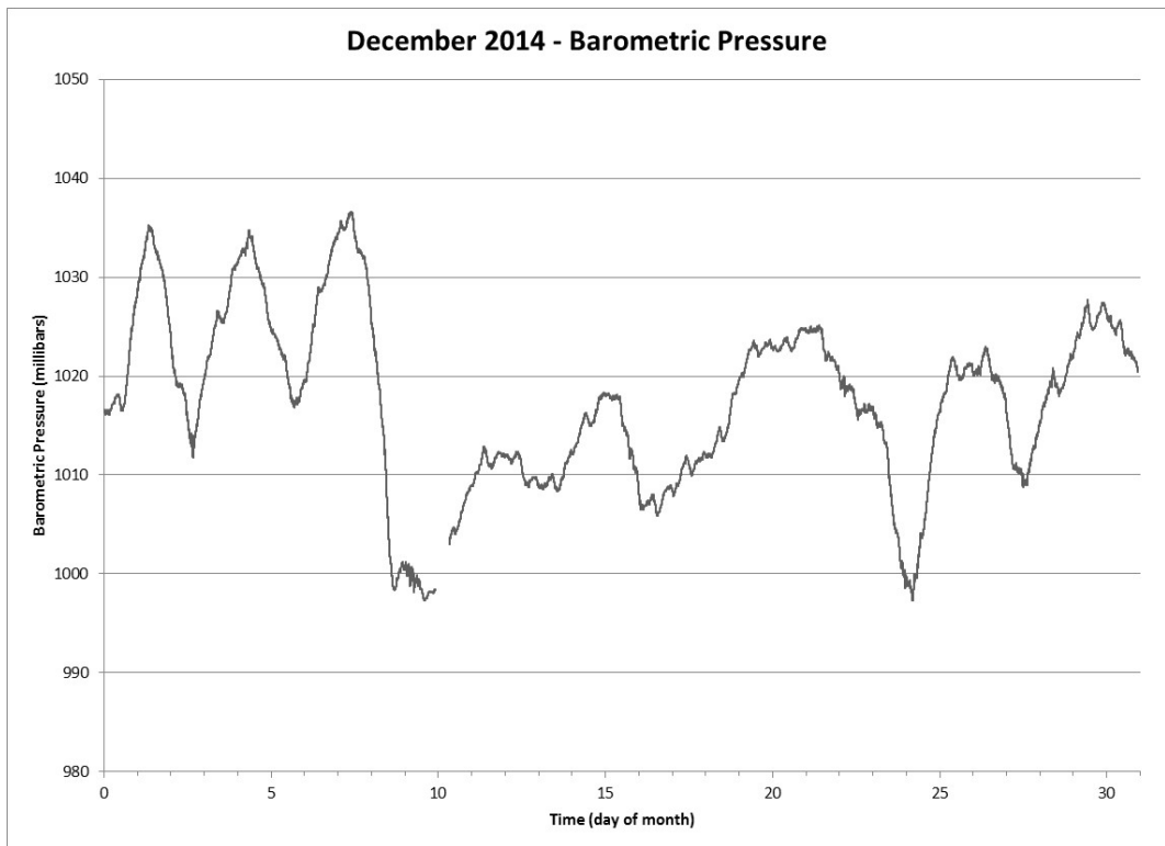
Figure 28 Barometric Pressure for the Month of December 2014
