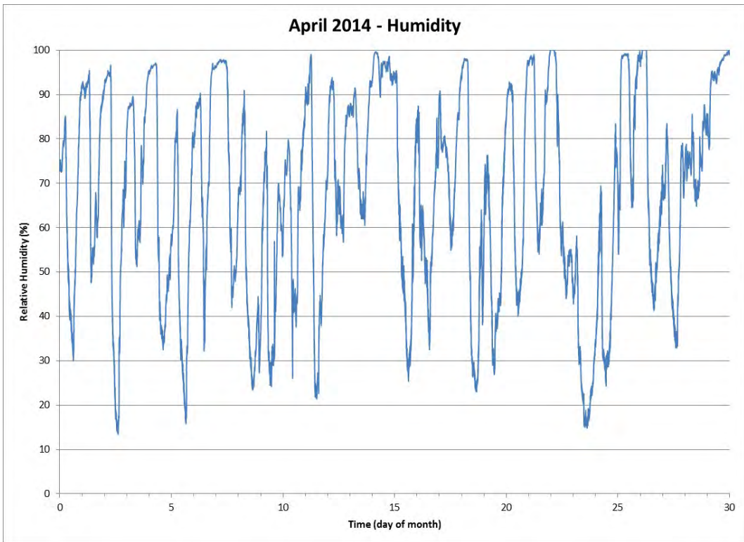
Figure 35 Relative Humidity for the Month of April 2014
