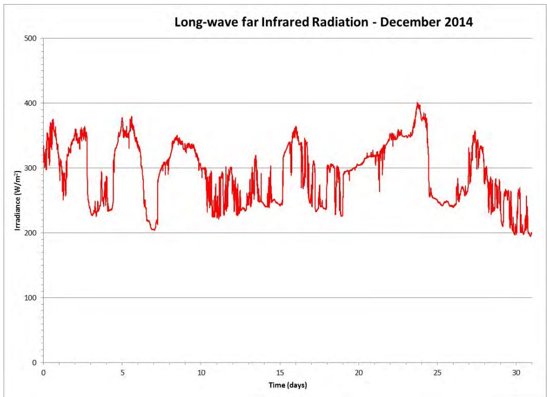
Figure 160 Long-wave Far Infrared Radiation for the Month of December 2014
