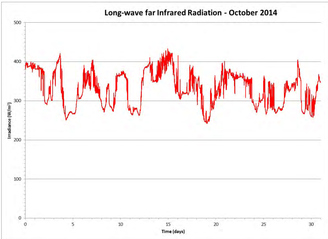
Figure 158 Long-wave Far Infrared Radiation for the Month of October 2014
