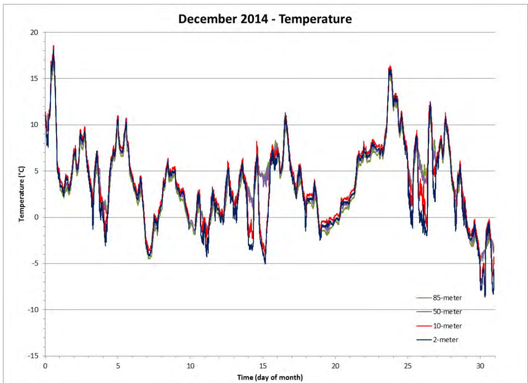
Figure 15 Air Temperature for the Month of December 2014
