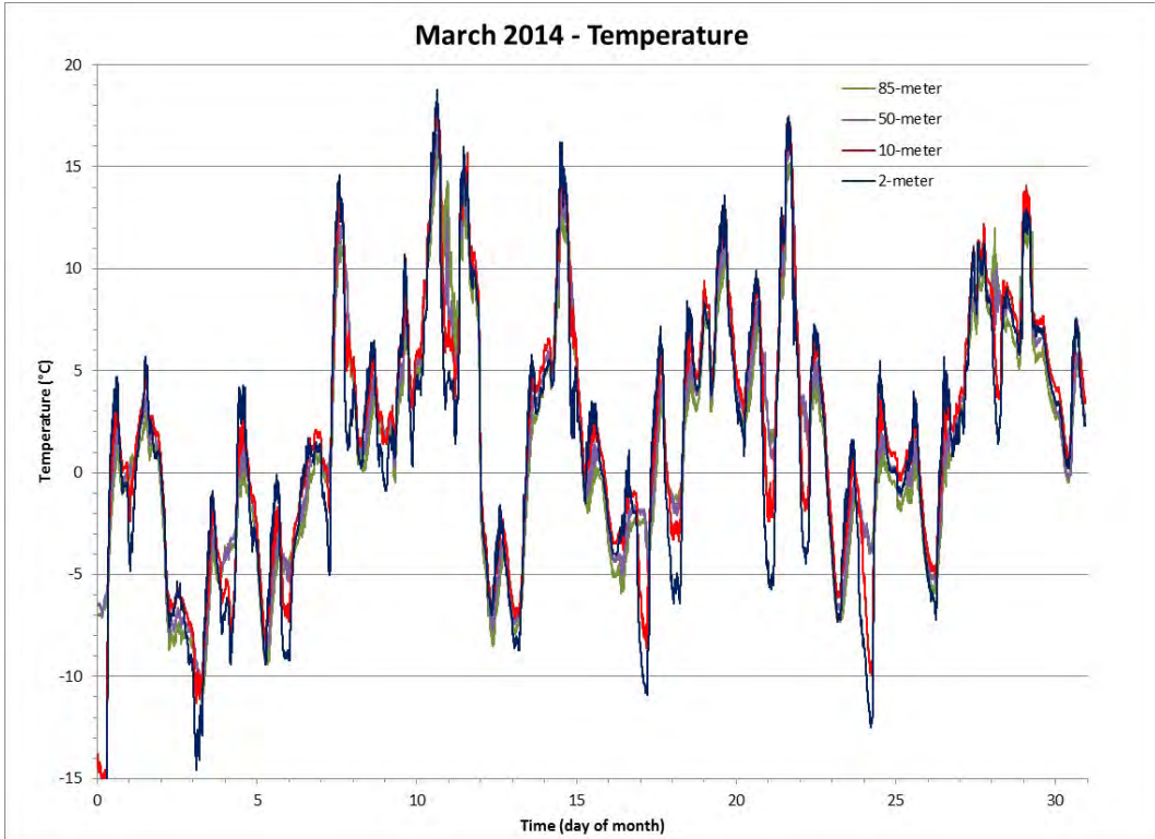
Figure 6 Air Temperature for the Month of March 2014
