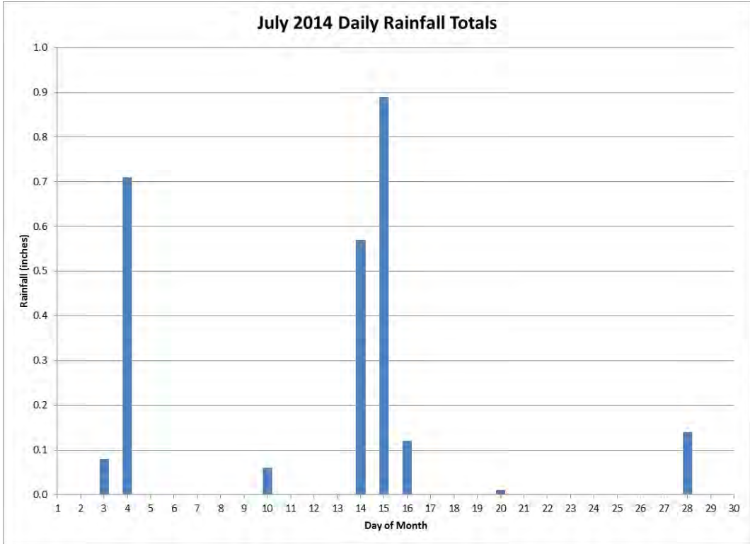
Figure 51 Daily Rainfall for the Month of July 2014
