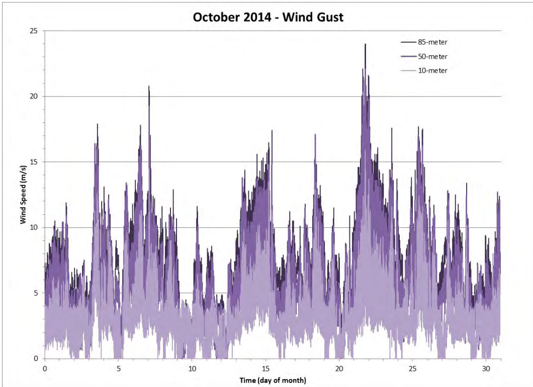
Figure 105 Wind Gust data for the Month of October 2014
