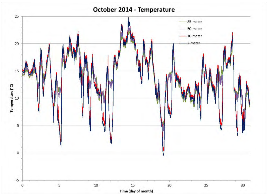
Figure 13 Air Temperature for the Month of October 2014
