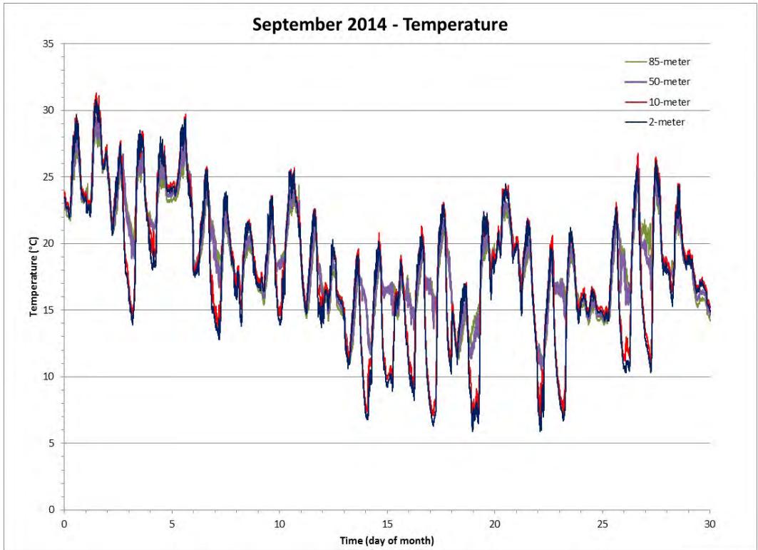
Figure 12 Air Temperature for the Month of September 2014
