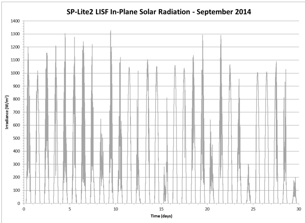
Figure 182 Tilted ( 27^\circ ) Global Solar Radiation from an SP-Lite2 Pyranometer for September 2014
