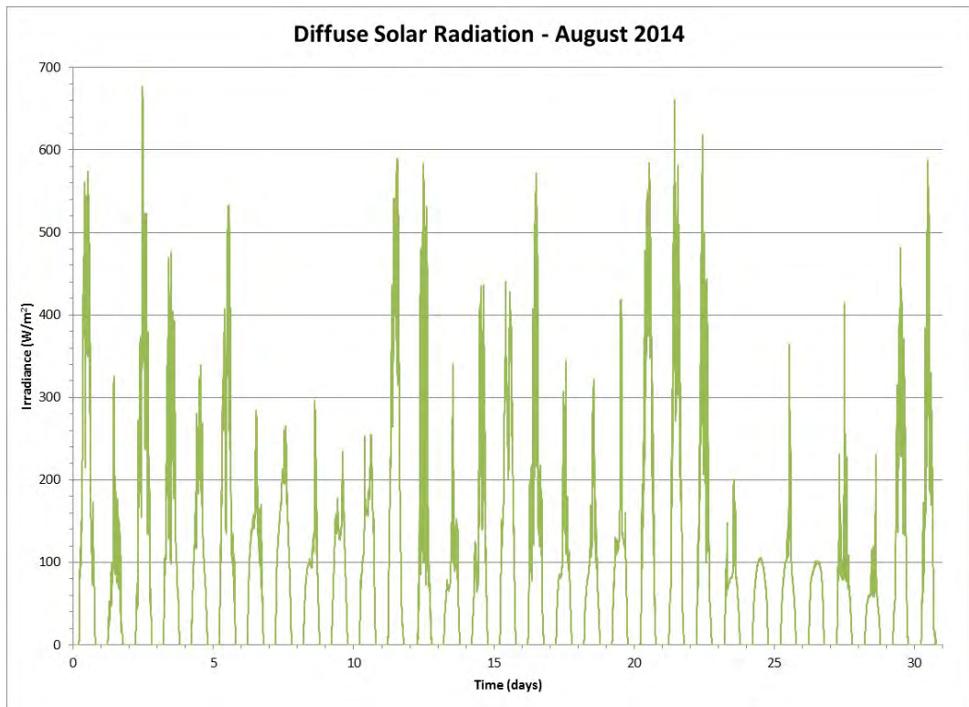
Figure 132 Diffuse Solar Radiation for the Month of August 2014
