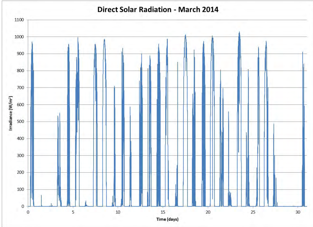
Figure 139 Direct Solar Radiation for the Month of March 2014
