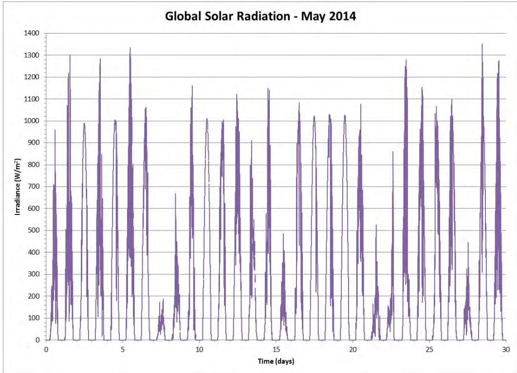
Figure 117 Global Solar Radiation for the Month of May 2014
