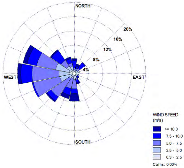
Figure 62 One-hour Wind Roses for the Month of January 2014 from the 85m level
