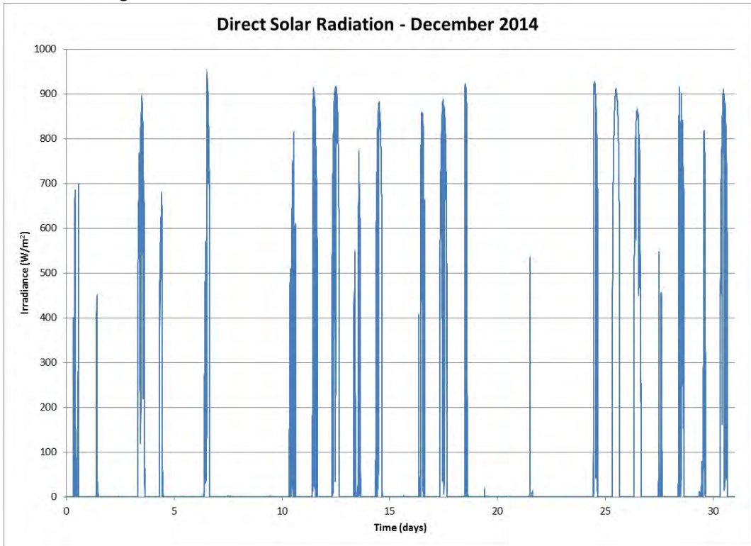
Figure 148 Direct Solar Radiation for the Month December 2014
