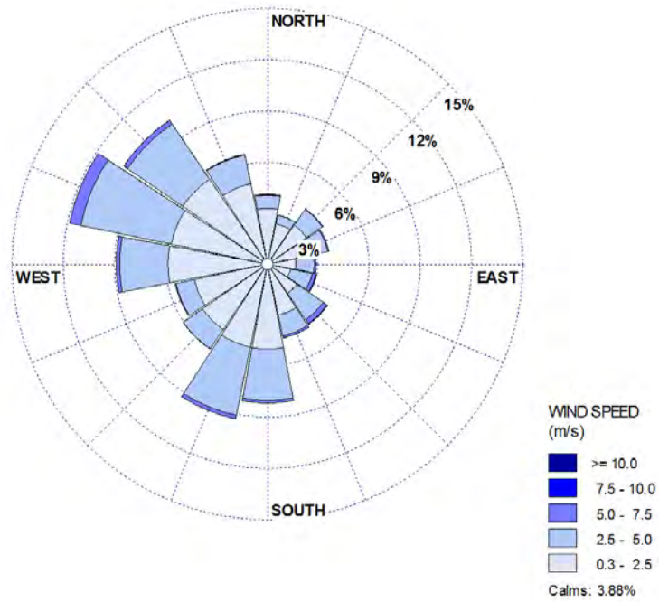
Figure 58 Historic Annual One-hour Wind Roses for the Years 1994 to 2014 from the 85m level
