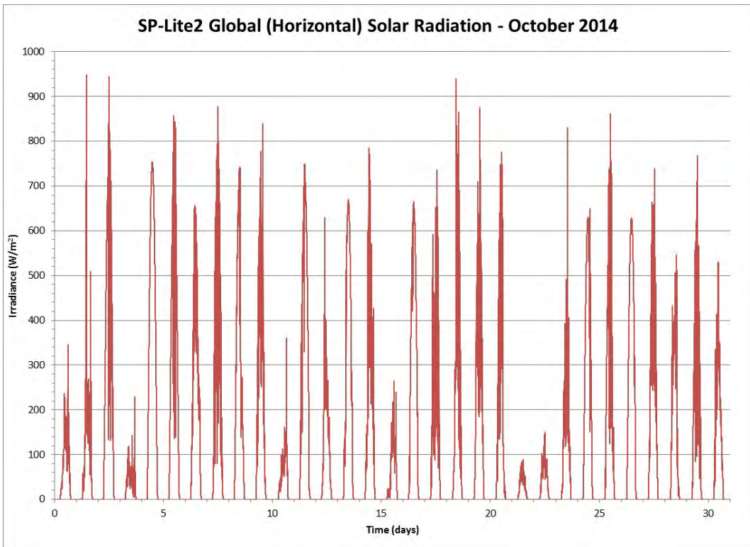
Figure 170 Global Solar Radiation from an SP-Lite2 Pyranometer for the Month of October 2014
