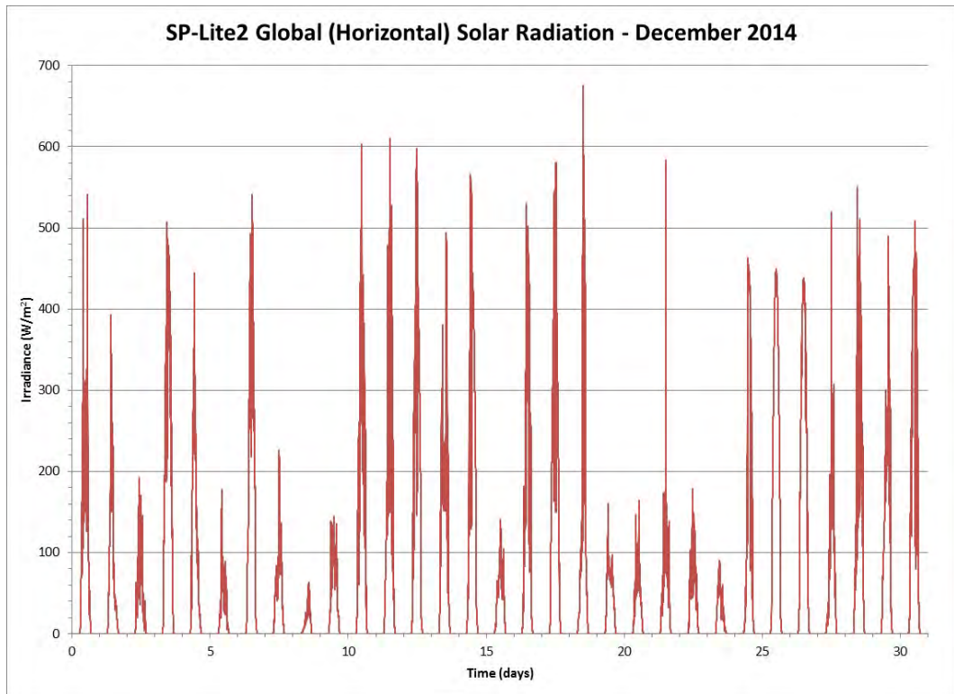
Figure 172 Global Solar Radiation from an SP-Lite2 Pyranometer for the Month of December 2014
