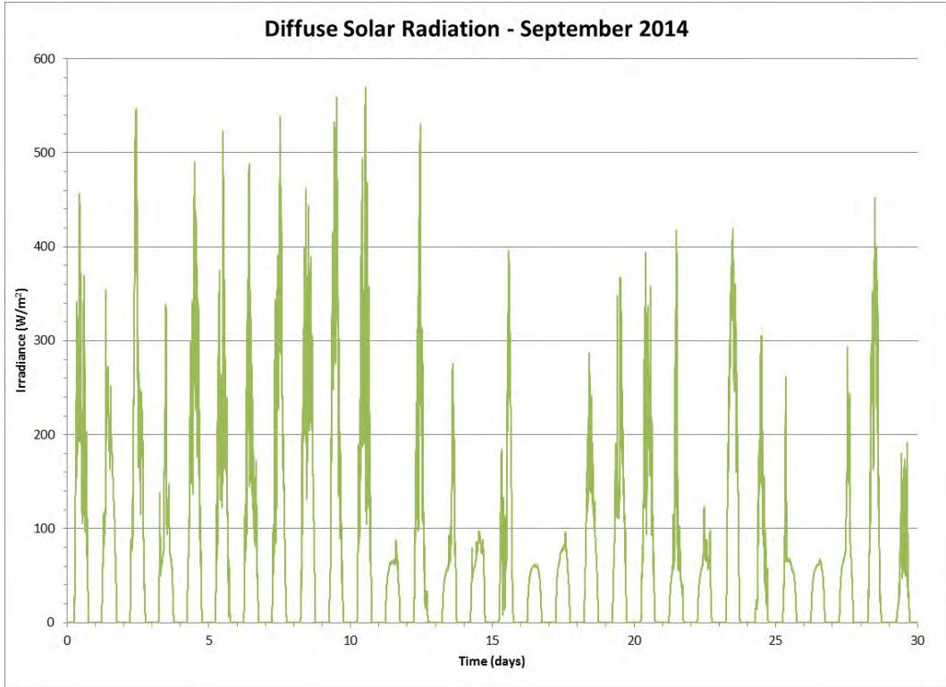
Figure 133 Diffuse Solar Radiation for the Month of September 2014
