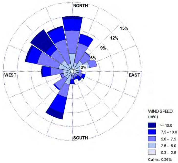
Figure 66 One-hour Wind Roses for the Month of March 2014 from the 85m level
