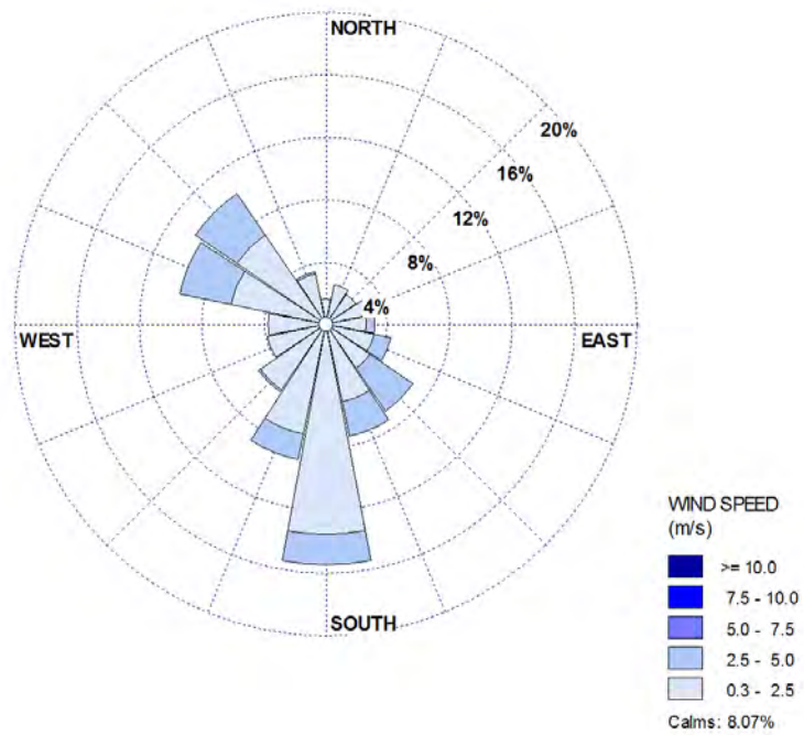
Figure 72 One-hour Wind Roses for the Month of June 2014 from the 85m level
