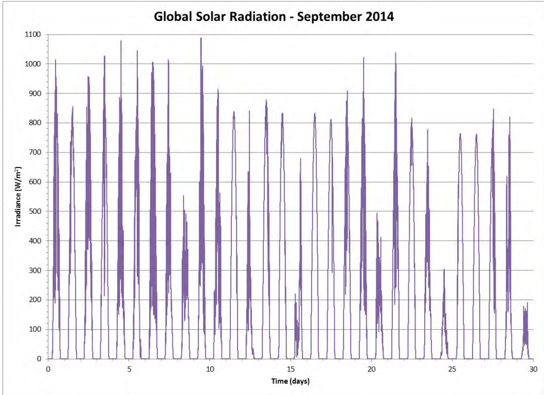
Figure 121 Global Solar Radiation for the Month of September 2014
