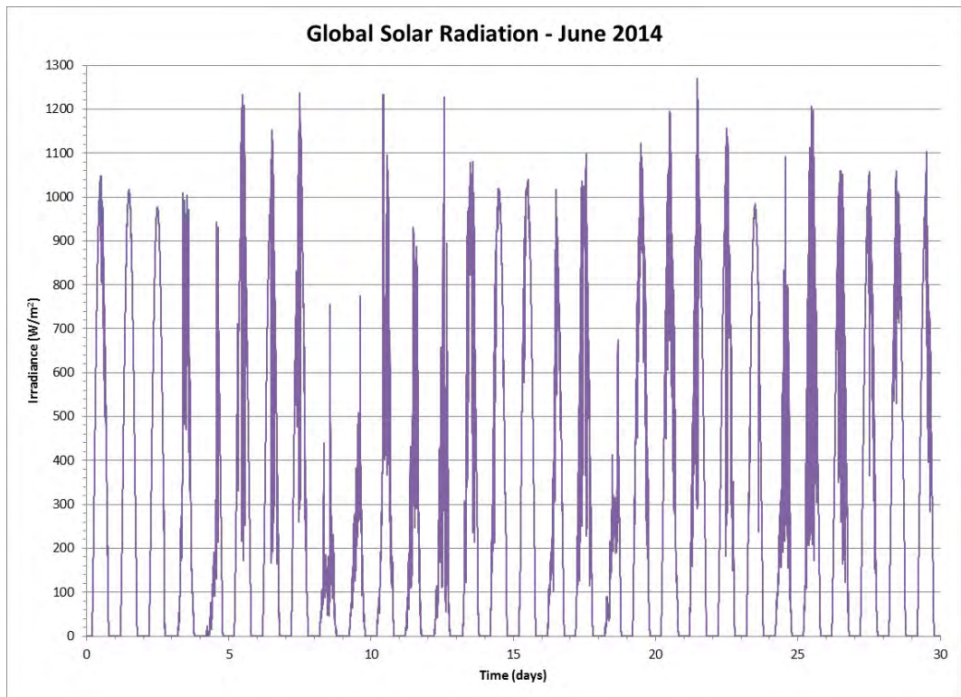
Figure 118 Global Solar Radiation for the Month of June 2014
