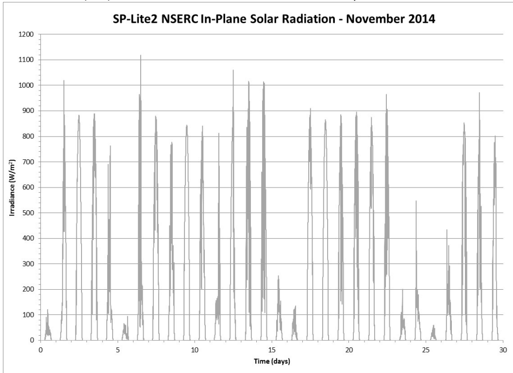
Figure 187 Tilted ( 23^\circ ) Global Solar Radiation from an SP-Lite2 Pyranometer for November 2014
