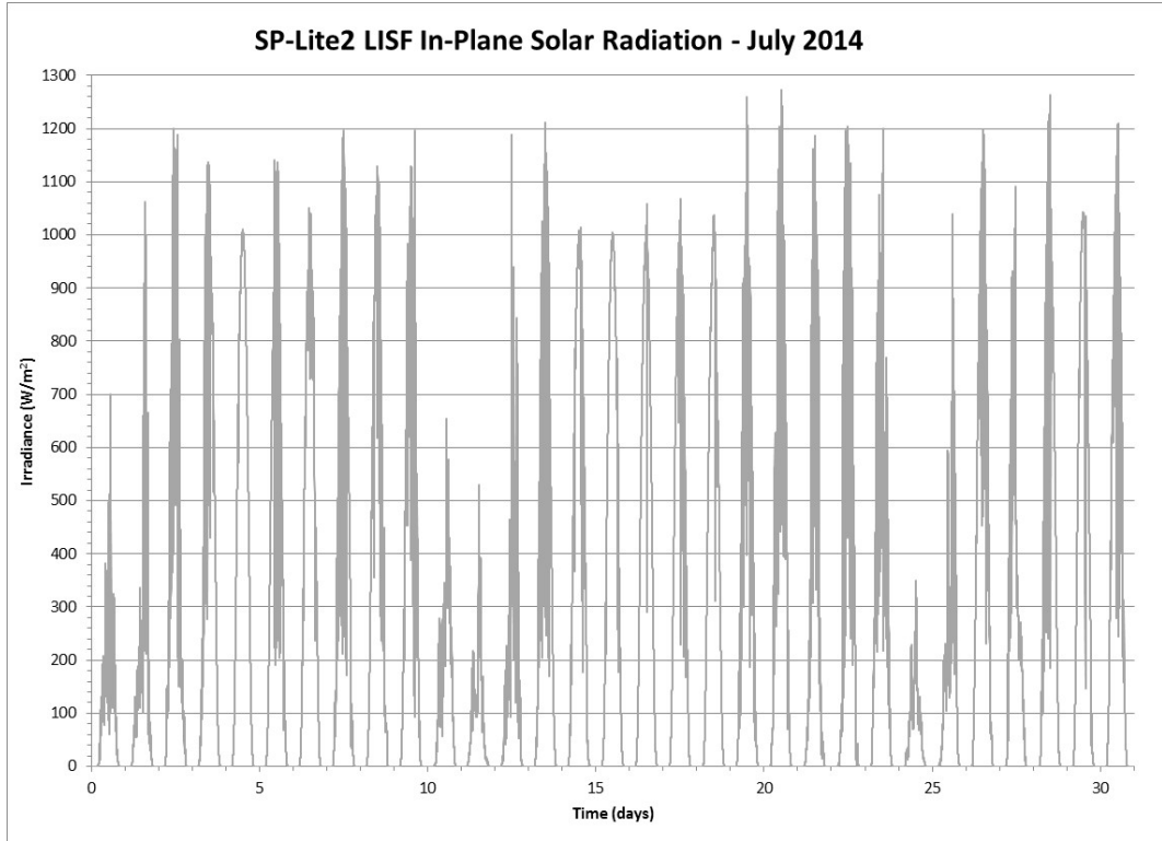
Figure 179 Tilted (27°) Global Solar Radiation from an SP-Lite2 Pyranometer for July 2014
