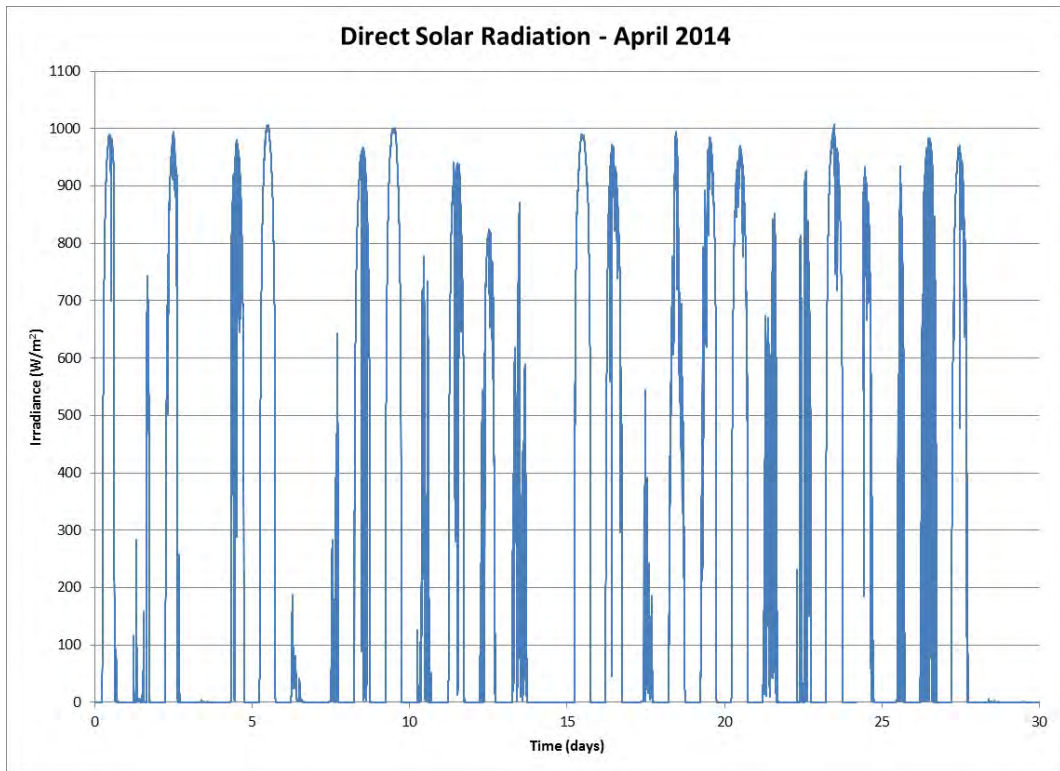
Figure 140 Direct Solar Radiation for the Month April 2014
