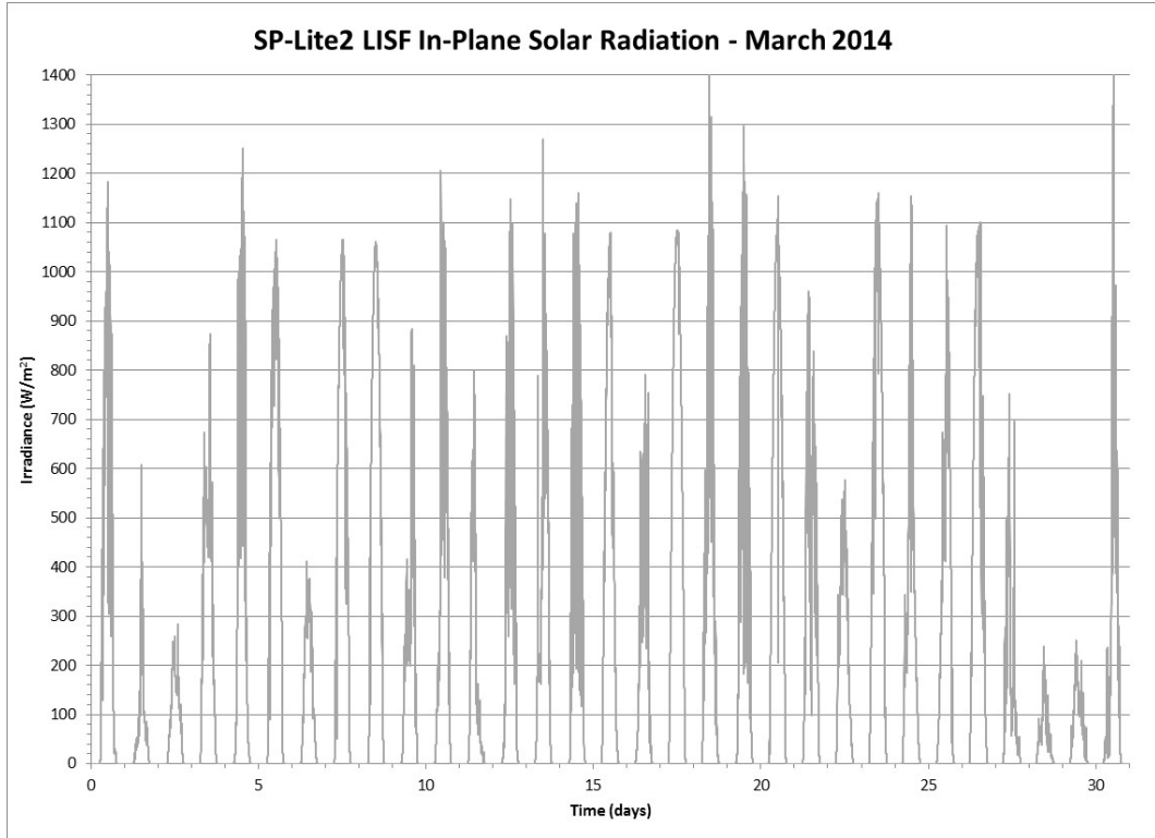
Figure 175 Tilted (27°) Global Solar Radiation from an SP-Lite2 Pyranometer for March 2014
