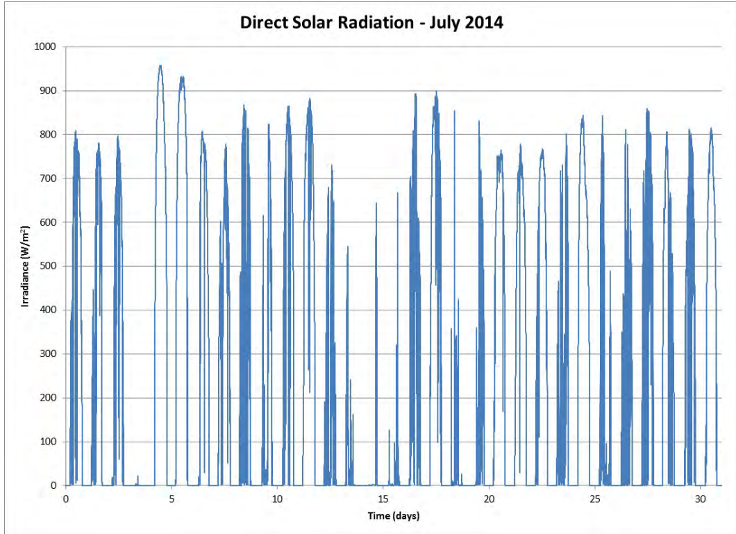
Figure 143 Direct Solar Radiation for the Month July 2014
