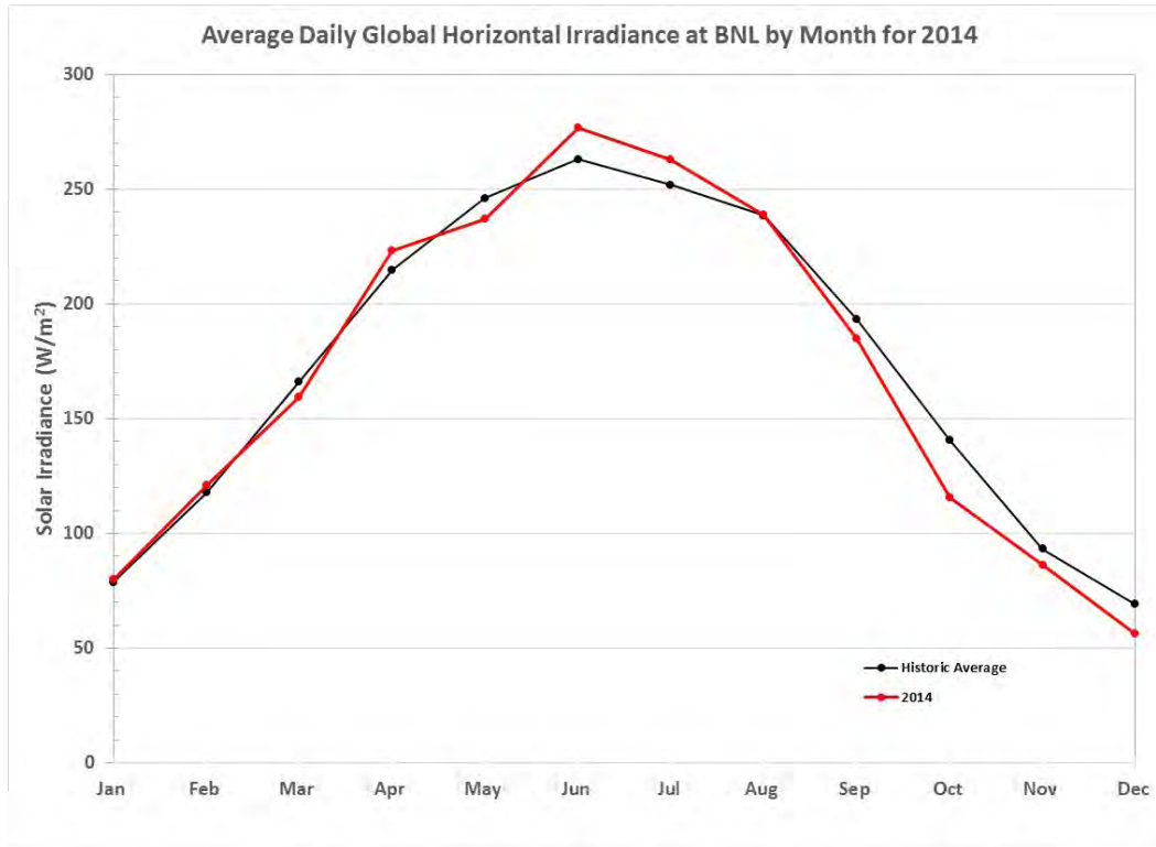
Figure 112 Global Horizontal Irradiance – 2014 Monthly Daily-Average
