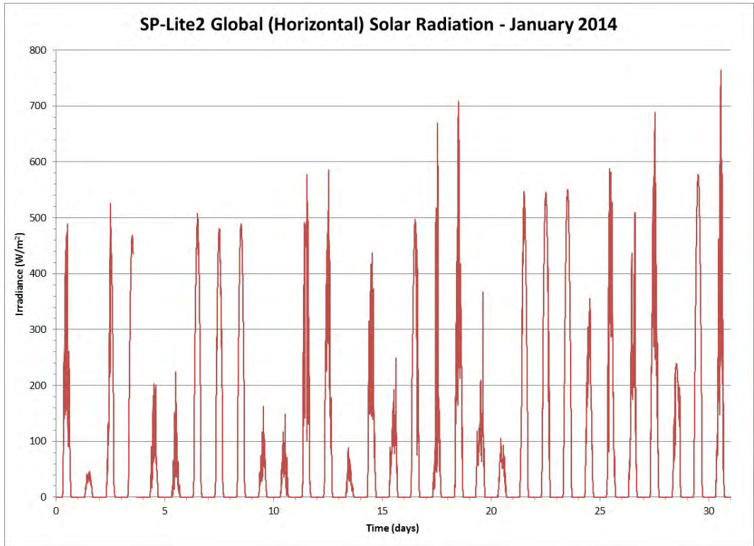
Figure 161 Global Solar Radiation from an SP-Lite2 Pyranometer for the Month of January 2014
