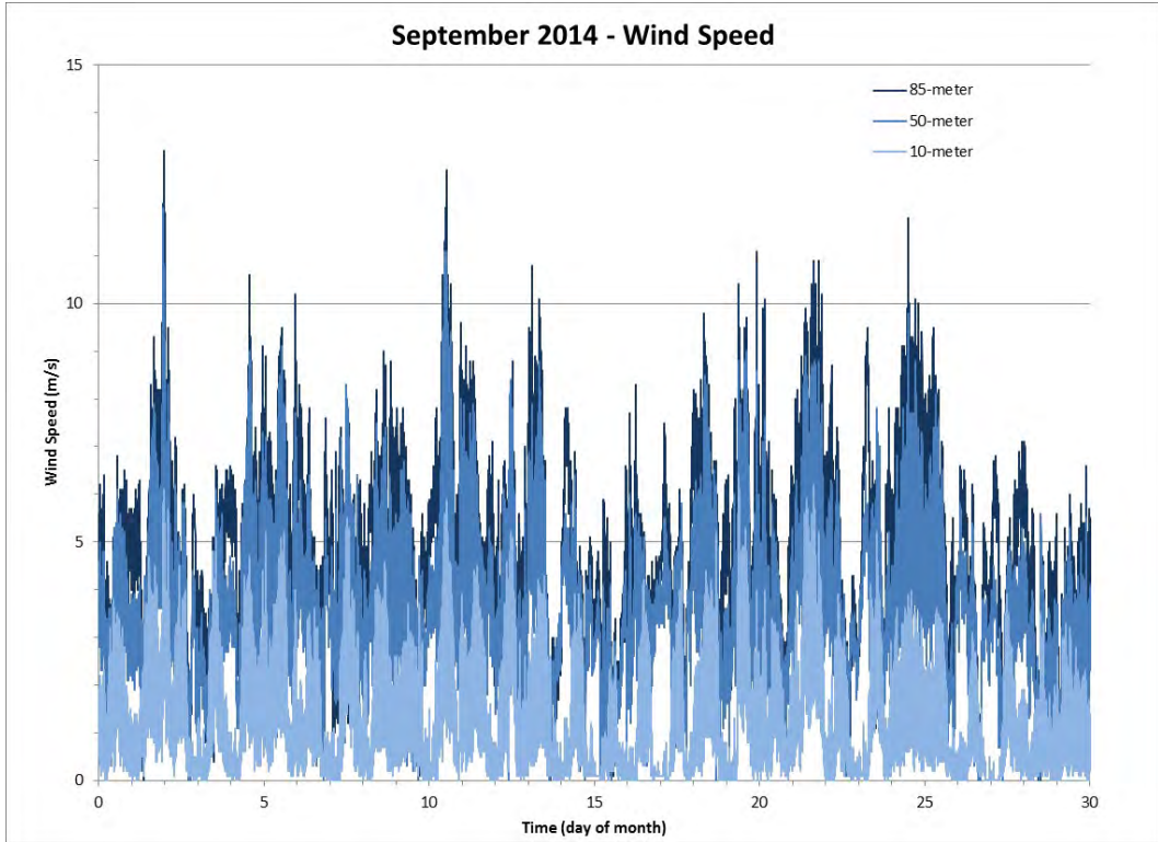
Figure 102 Wind Speed for the Month of September 2014
