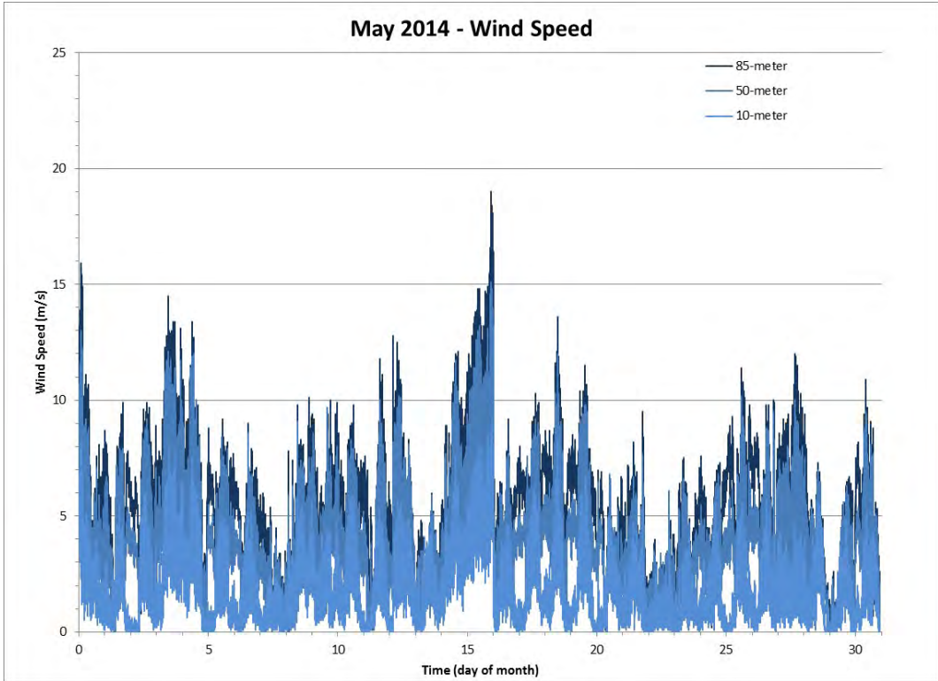
Figure 94 Wind Speed for the Month of May 2014
