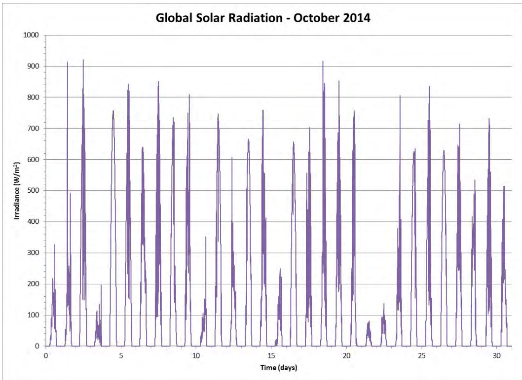
Figure 122 Global Solar Radiation for the Month of October 2014
