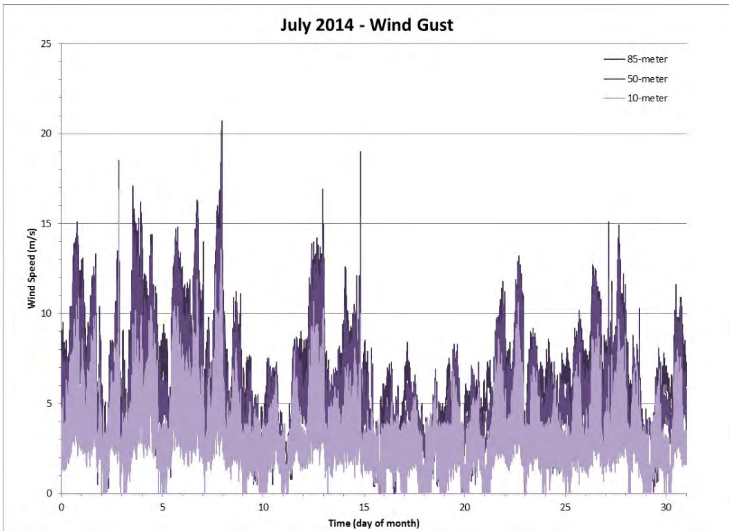
Figure 99 Wind Gust data for the Month of July 2014
