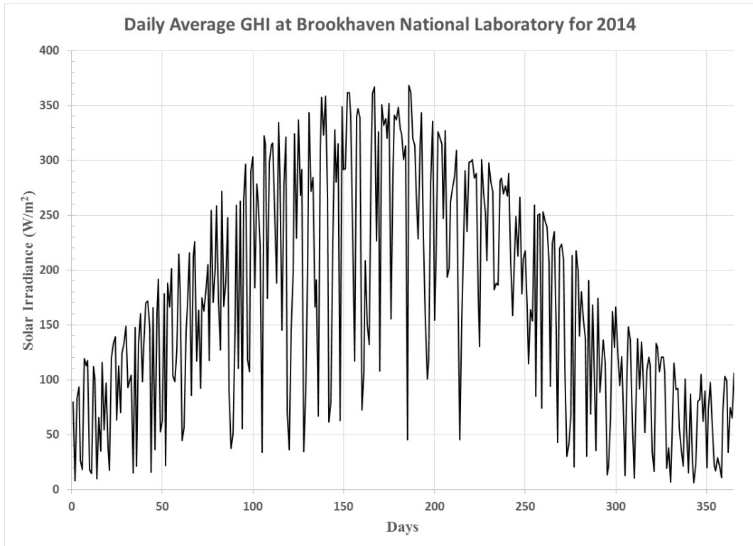
Figure 111 Average Daily Solar Irradiance at Brookhaven National Laboratory for 2014
