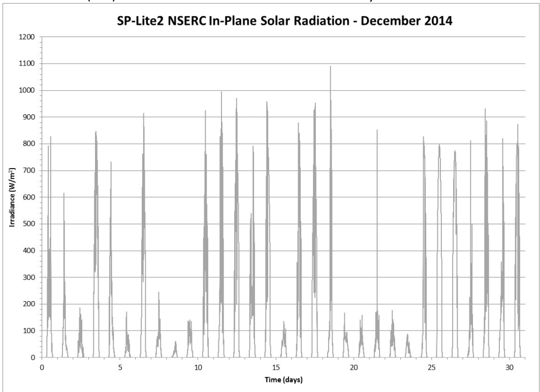
Figure 189 Tilted ( 23^\circ ) Global Solar Radiation from an SP-Lite2 Pyranometer for December 2014
