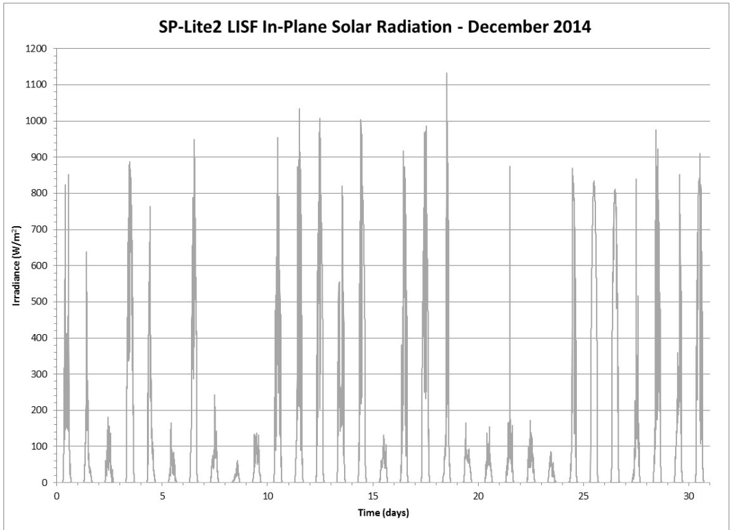
Figure 188 Tilted ( 27^\circ ) Global Solar Radiation from an SP-Lite2 Pyranometer for December 2014
