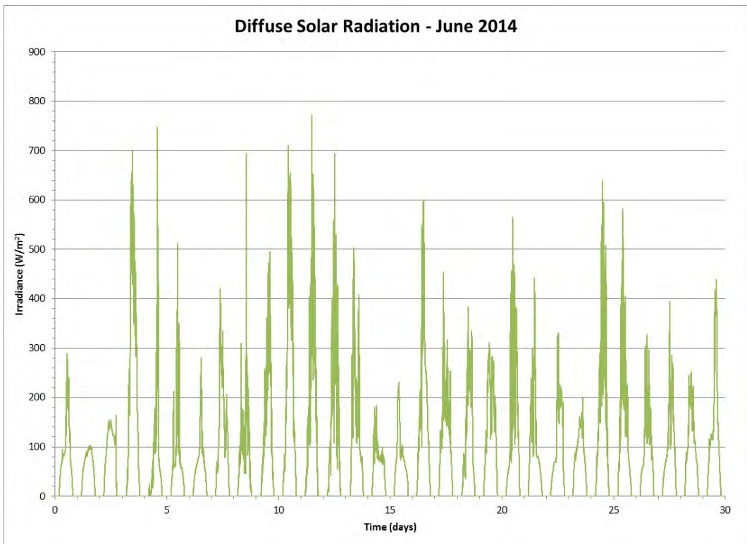
Figure 130 Diffuse Solar Radiation for the Month of June 2014
