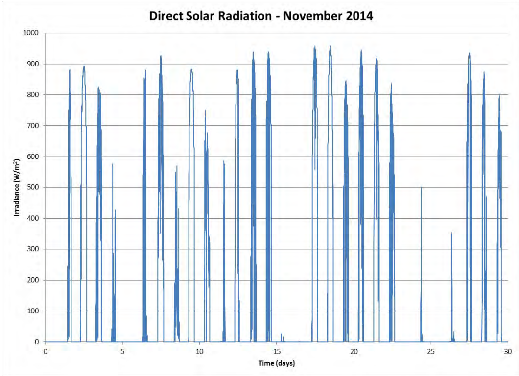
Figure 147 Direct Solar Radiation for the Month November 2014
