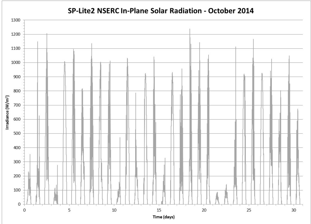
Figure 185 Tilted ( 23^\circ ) Global Solar Radiation from an SP-Lite2 Pyranometer for October 2014
