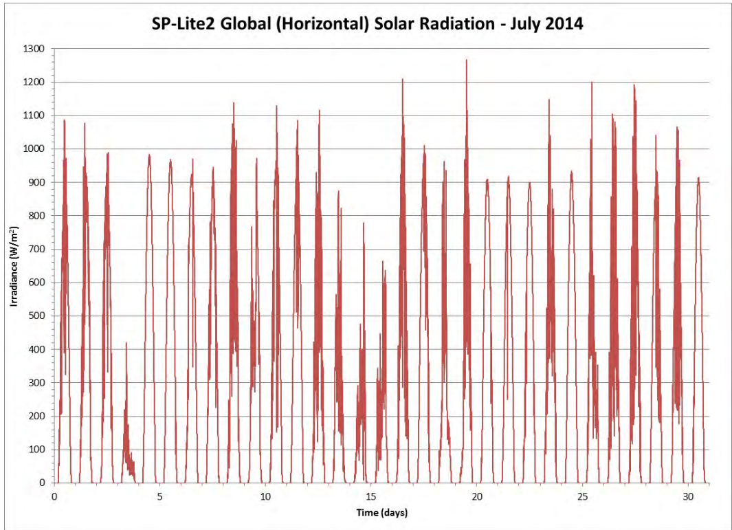
Figure 16751 Global Solar Radiation from an SP-Lite2 Pyranometer for the Month of July 2014
