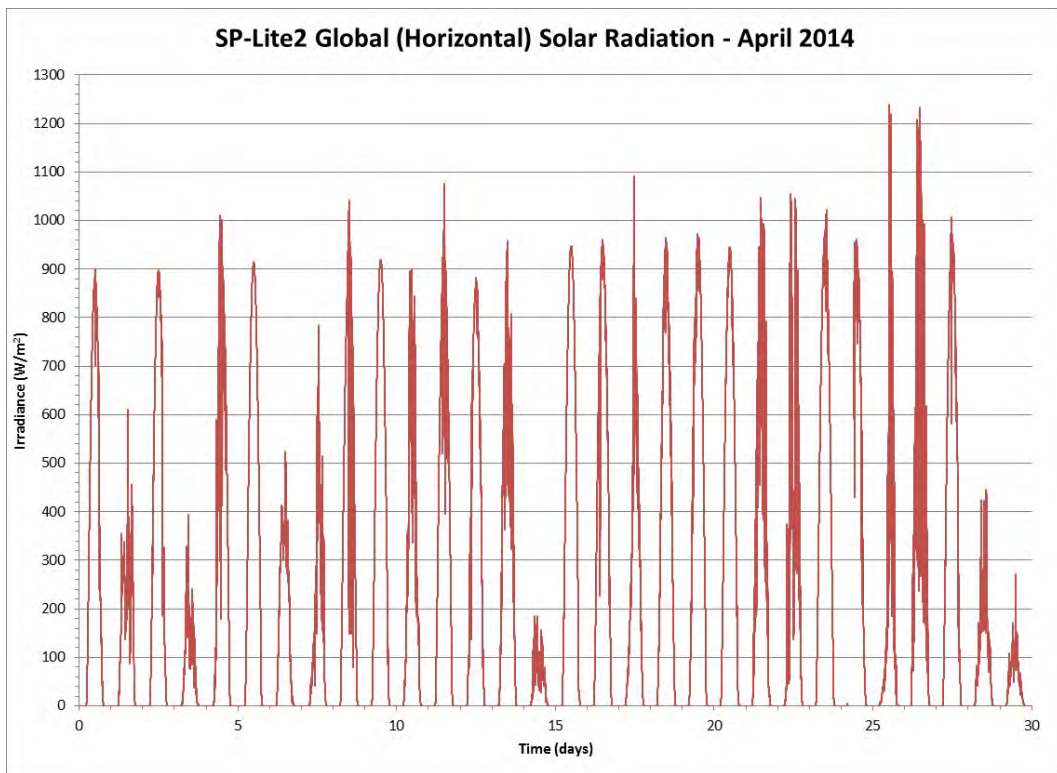
Figure 164 Global Solar Radiation from an SP-Lite2 Pyranometer for the Month of April 2014
