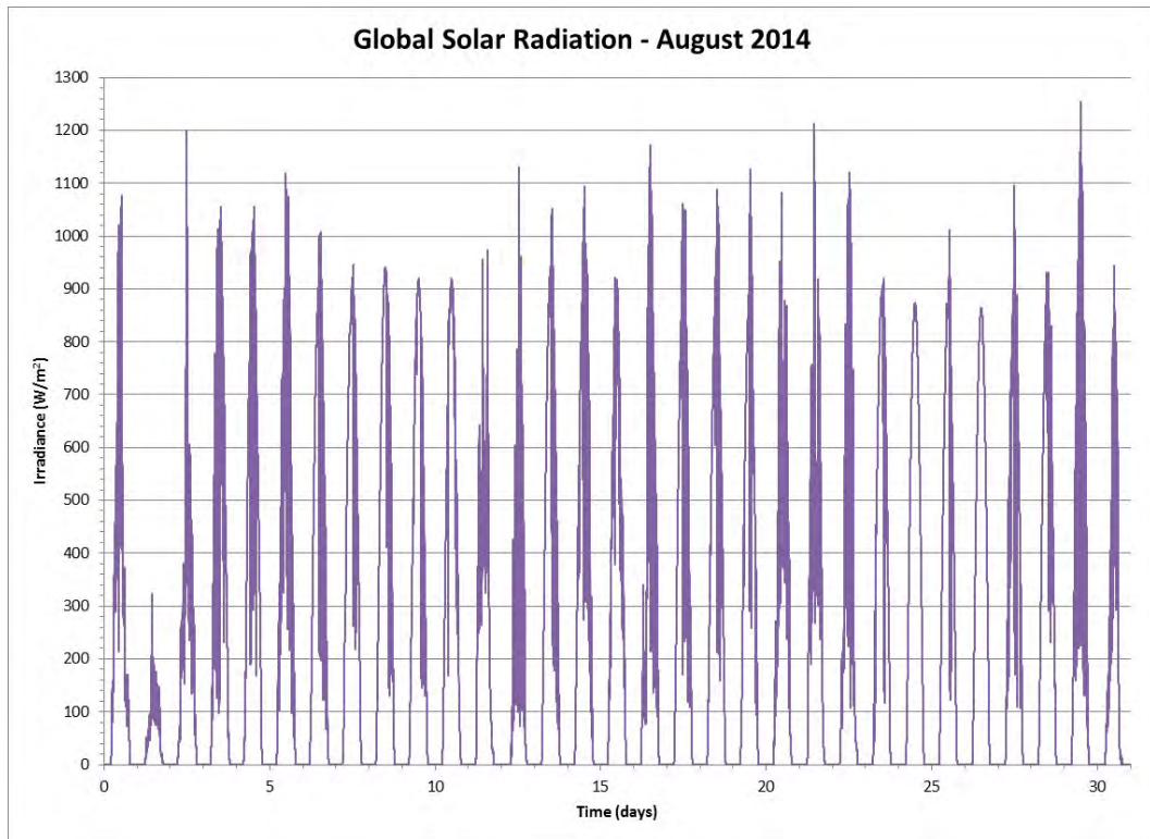
Figure 120 Global Solar Radiation for the Month of August 2014
