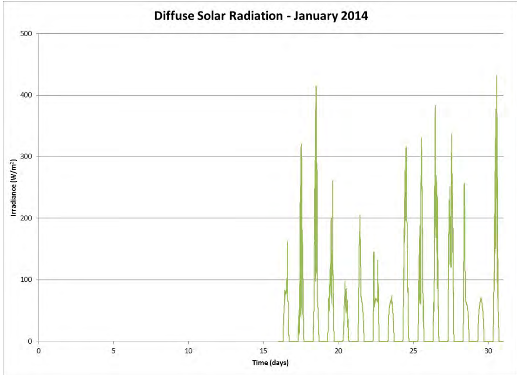
Figure 125 Diffuse Solar Radiation for the Month of January 2014
