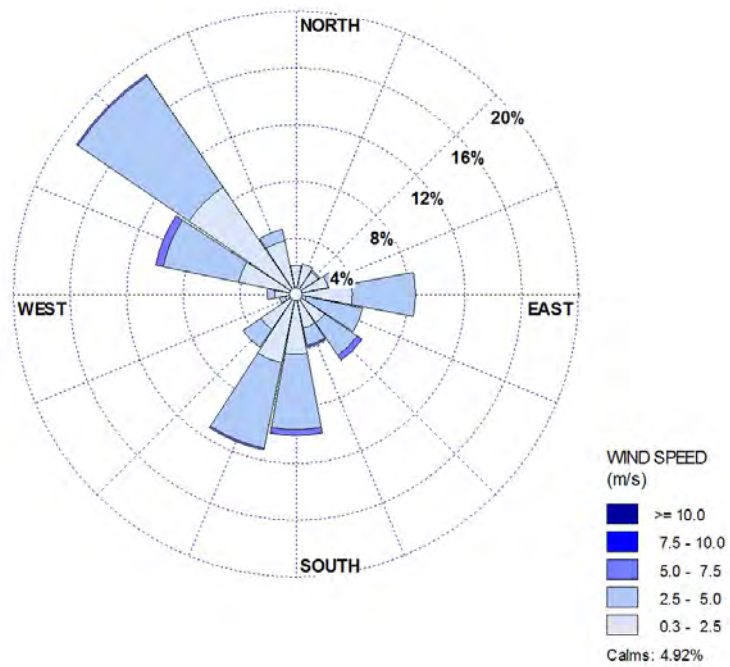
Figure 68 One-hour Wind Roses for the Month of April 2014 from the 85m level
