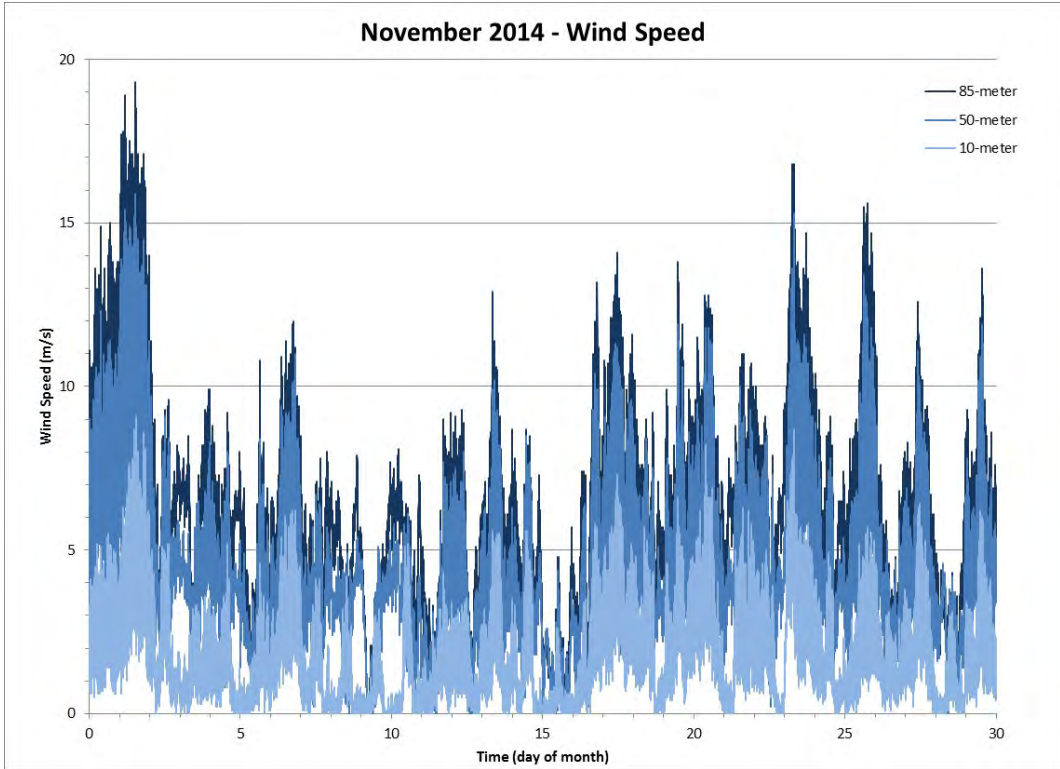
Figure 106 Wind Speed for the Month of November 2014
