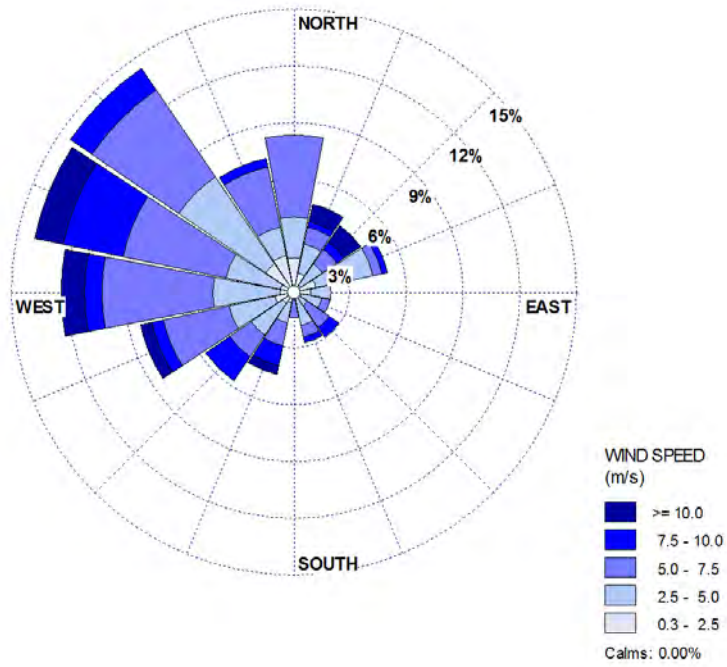
Figure 64 One-hour Wind Roses for the Month of February 2014 from the 85m level
