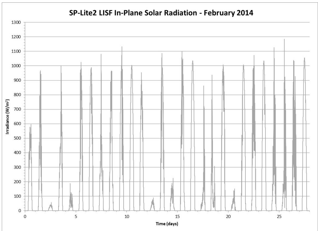
Figure 174 Tilted ( 27^\circ ) Global Solar Radiation from an SP-Lite2 Pyranometer for February 2014
