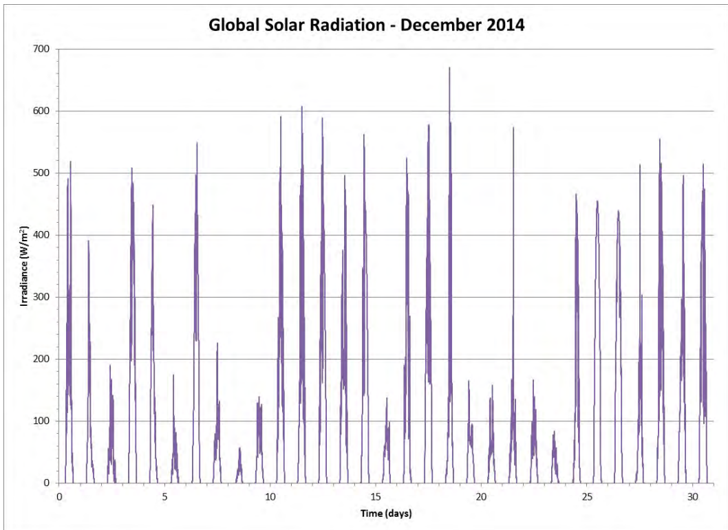
Figure 124 Global Solar Radiation for the Month of December 2014
