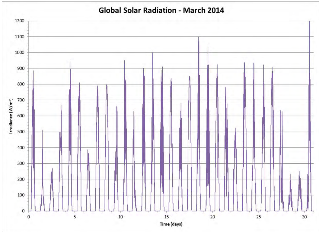
Figure 115 Global Solar Radiation for the Month of March 2014
