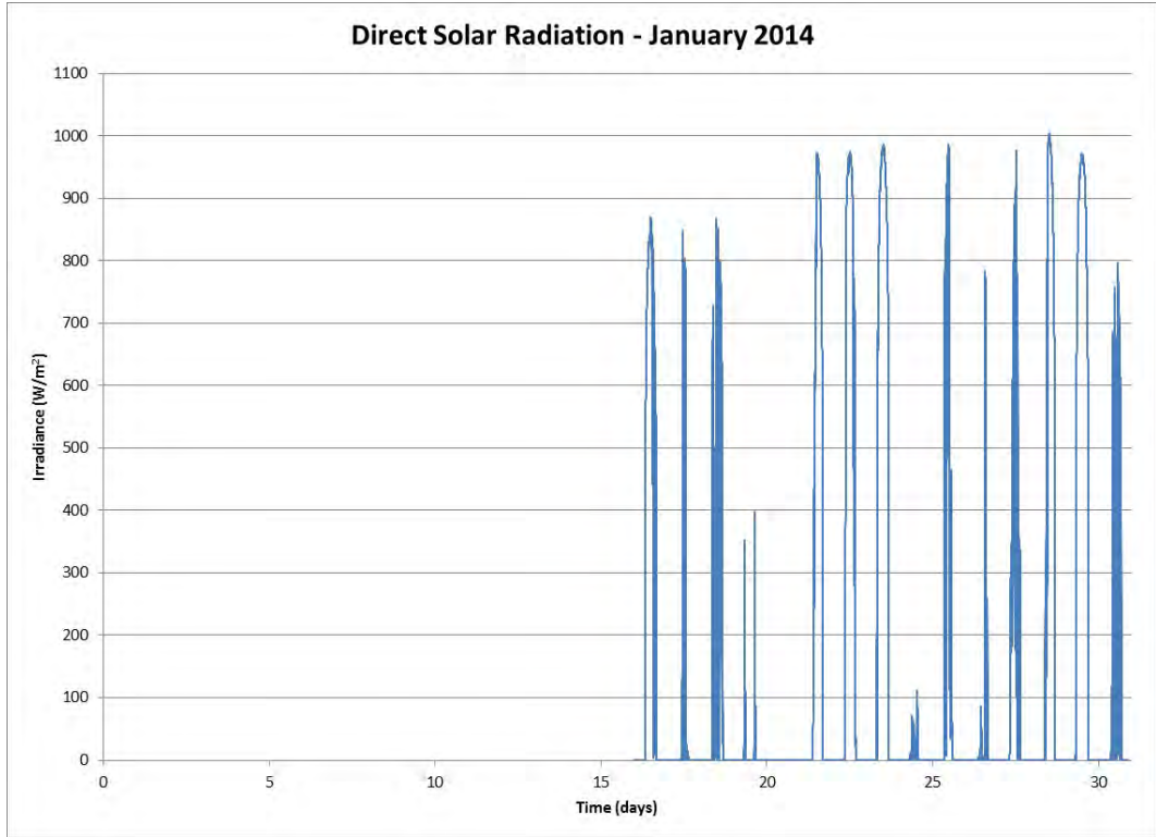
Figure 137 Direct Solar Radiation for the Month of January 2014
