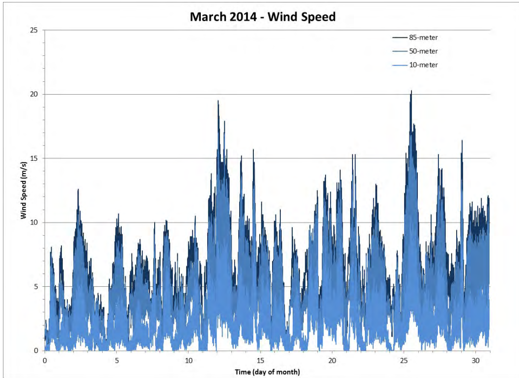
Figure 90 Wind Speed for the Month of March 2014
