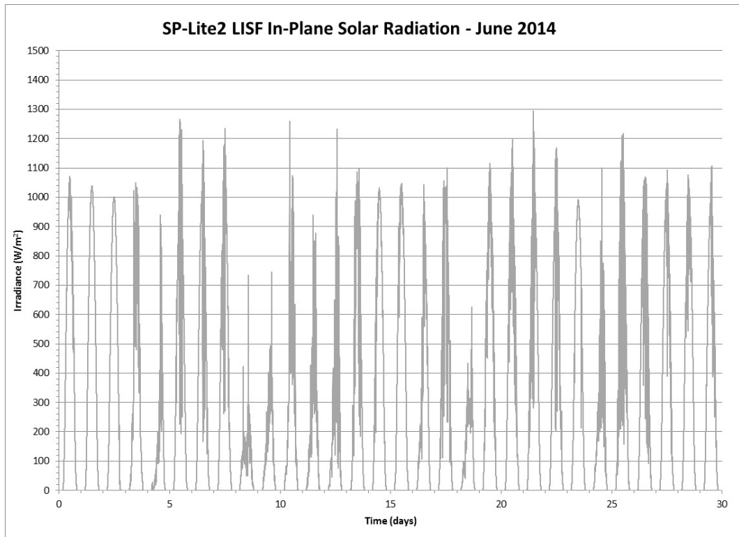
Figure 178 Tilted (27°) Global Solar Radiation from an SP-Lite2 Pyranometer for June 2014
