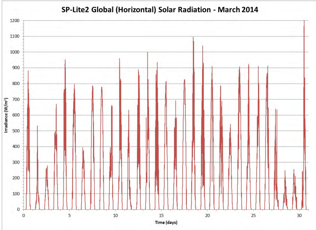
Figure 163 Global Solar Radiation from an SP-Lite2 Pyranometer for the Month of March 2014
