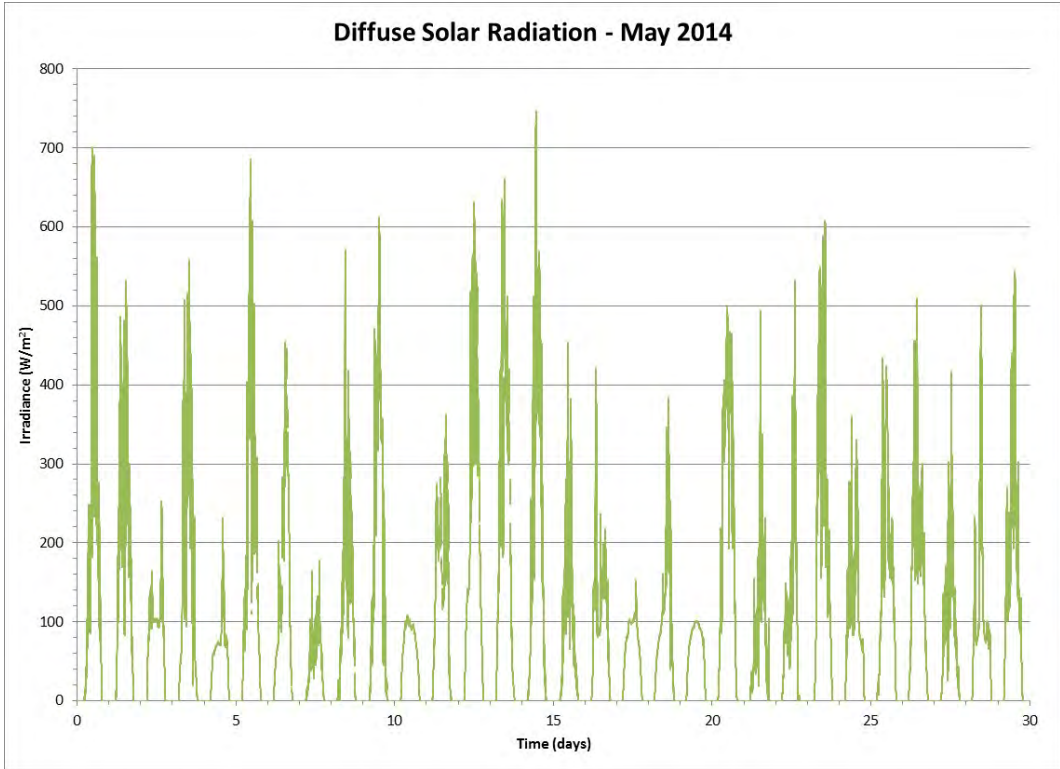
Figure 129 Diffuse Solar Radiation for the Month of May 2014
