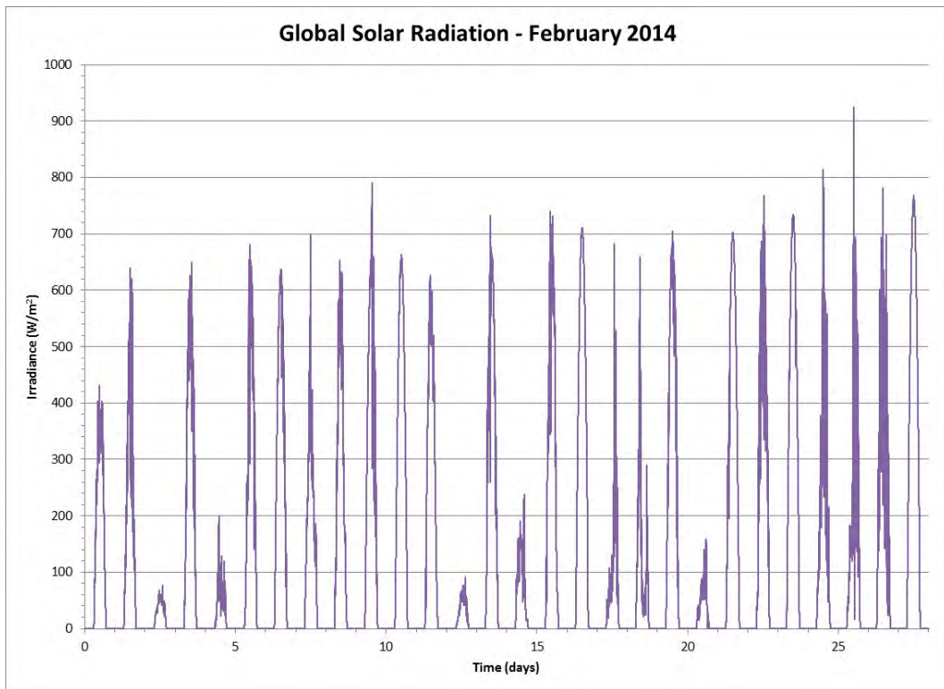
Figure 114 Global Solar Radiation for the Month of February 2014
