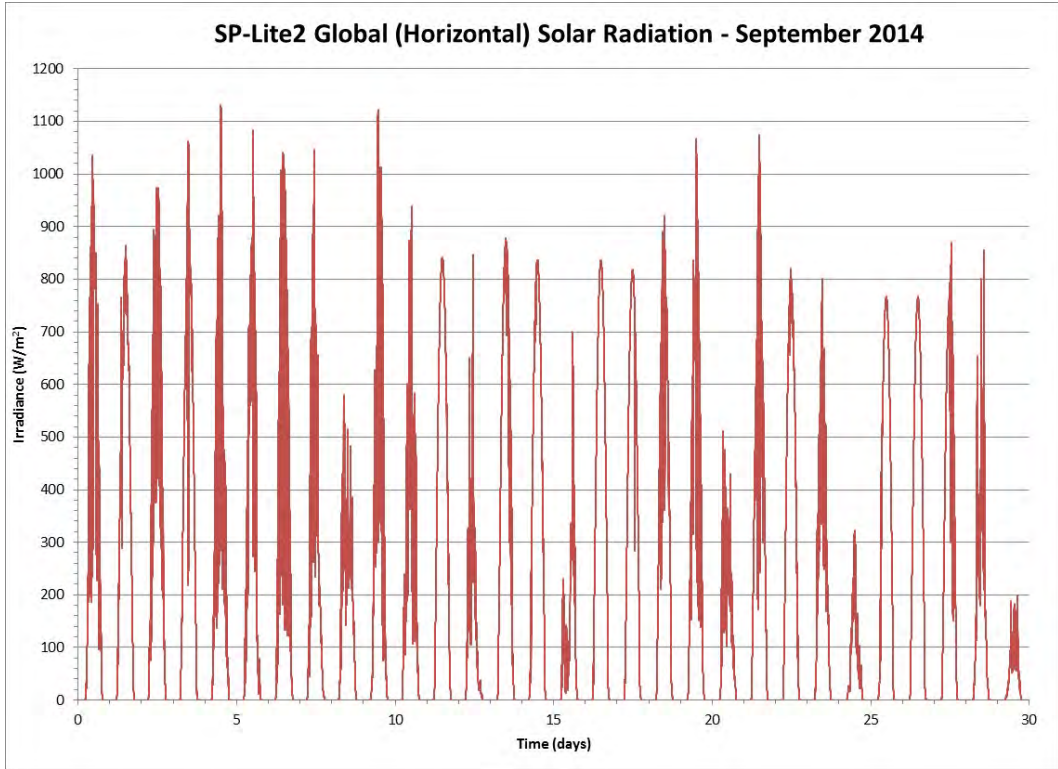
Figure 169 Global Solar Radiation from an SP-Lite2 Pyranometer for the Month of September 2014
