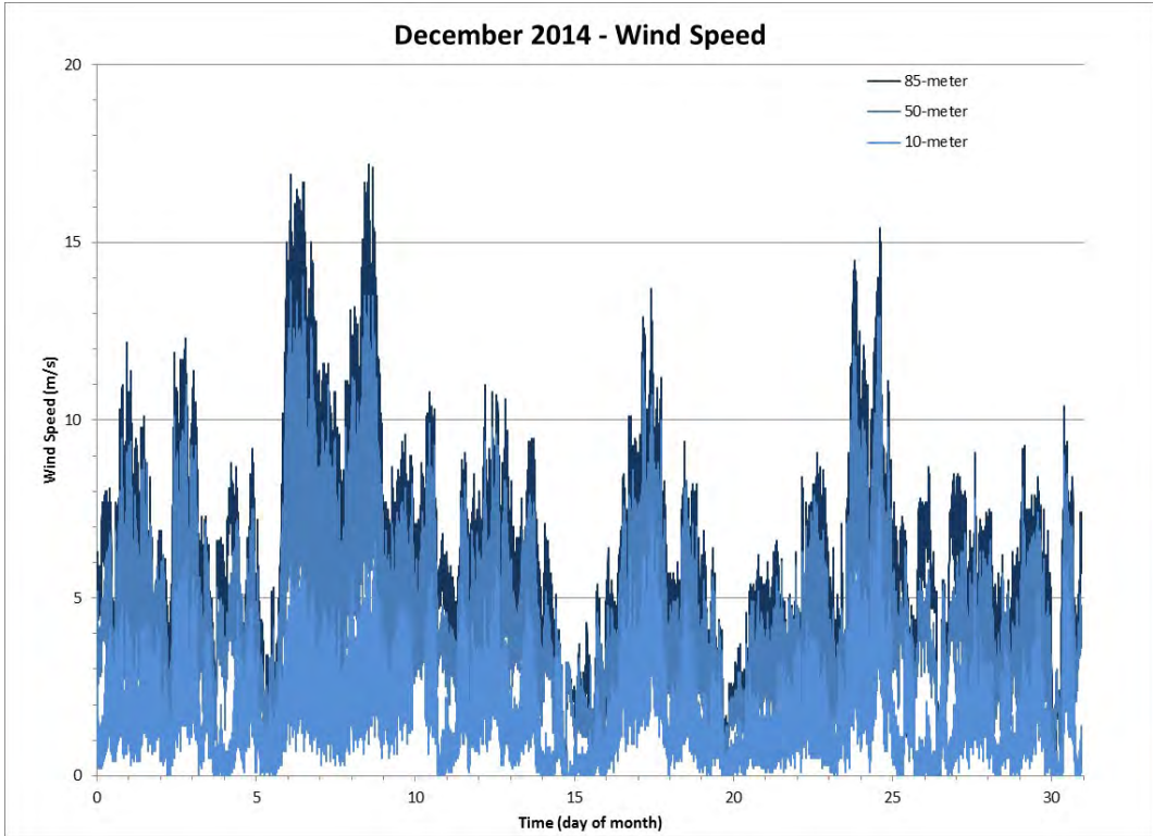
Figure 108 Wind Speed for the Month of December 2014
