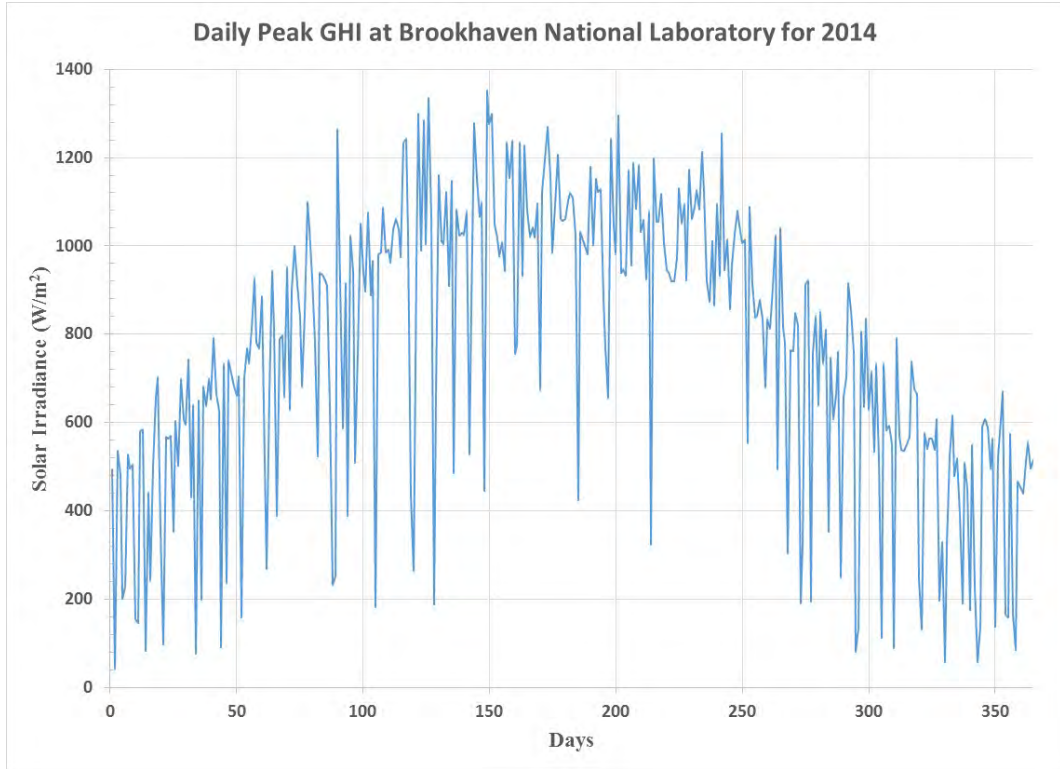
Figure 110 Daily Peak Solar Irradiance at Brookhaven National Laboratory for 2014
