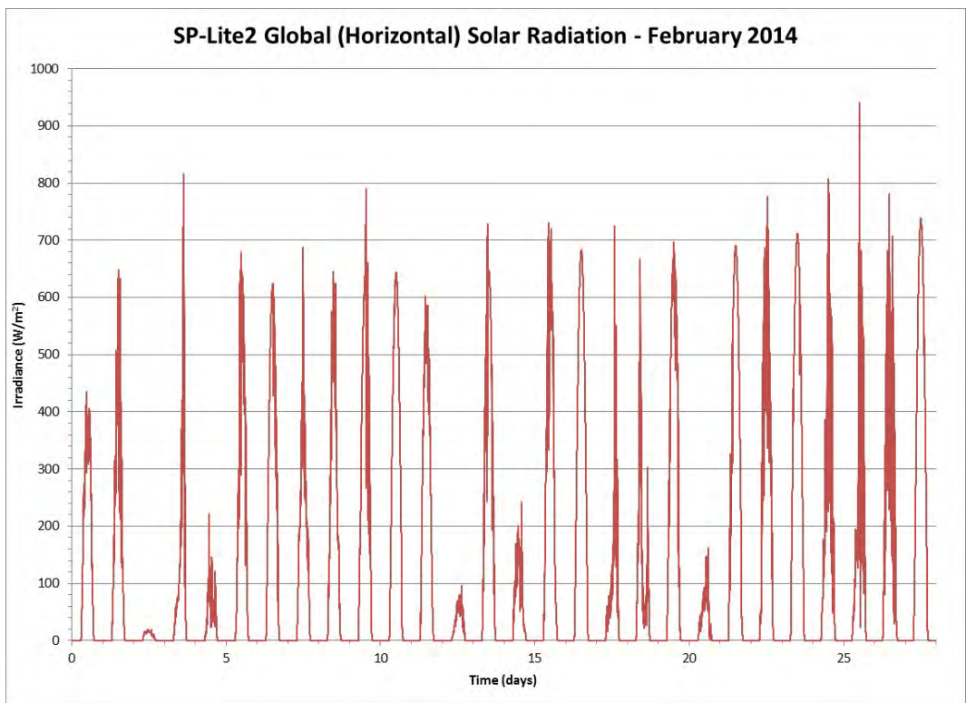
Figure 162 Global Solar Radiation from an SP-Lite2 Pyranometer for the Month of February 2014
