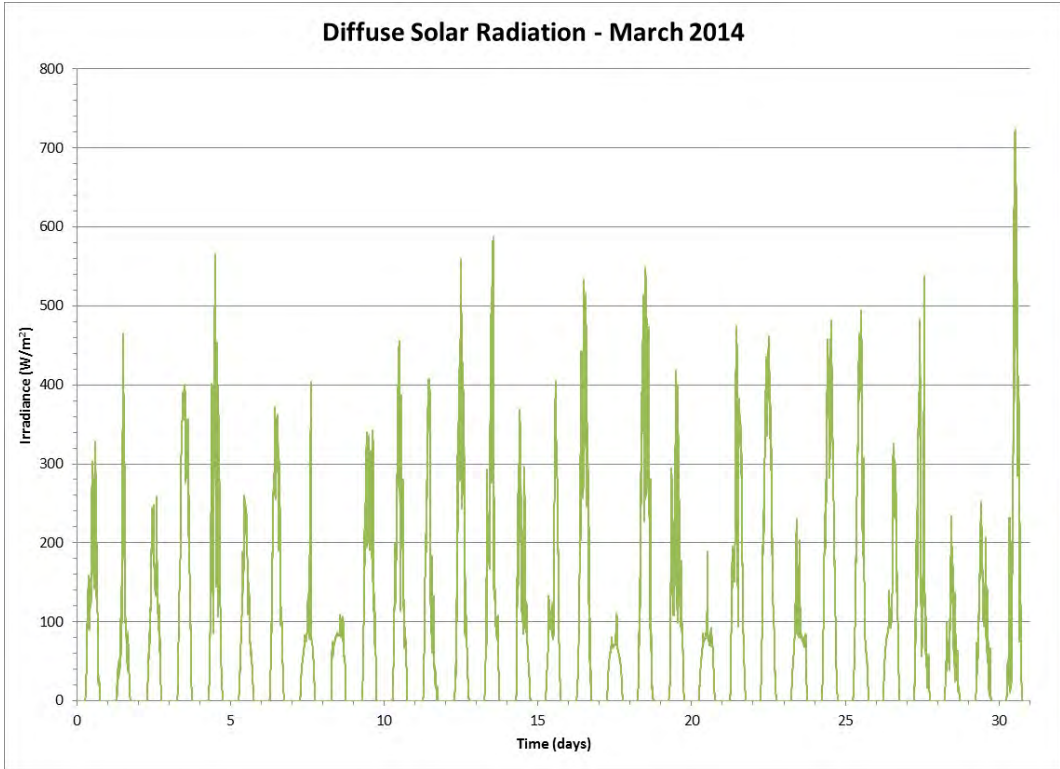
Figure 127 Diffuse Solar Radiation for the Month of March 2014
