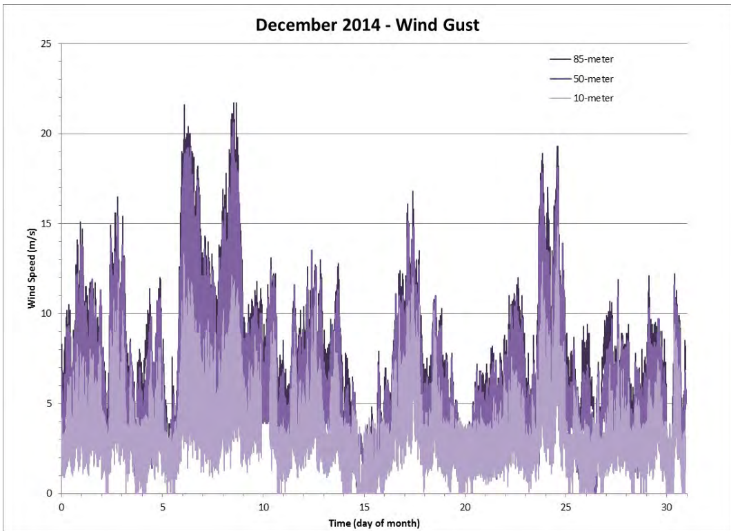
Figure 109 Wind Gust data for the Month of December 2014
