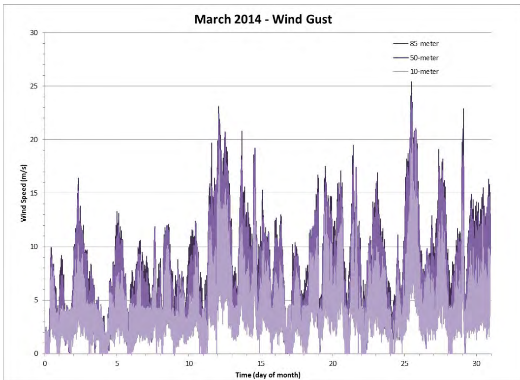
Figure 91 Wind Gust data for the Month of March 2014
