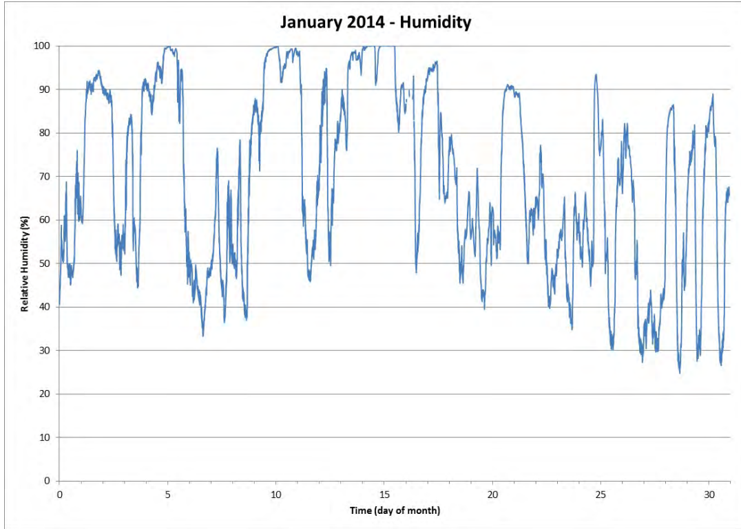
Figure 32 Relative Humidity for the Month of January 2014
