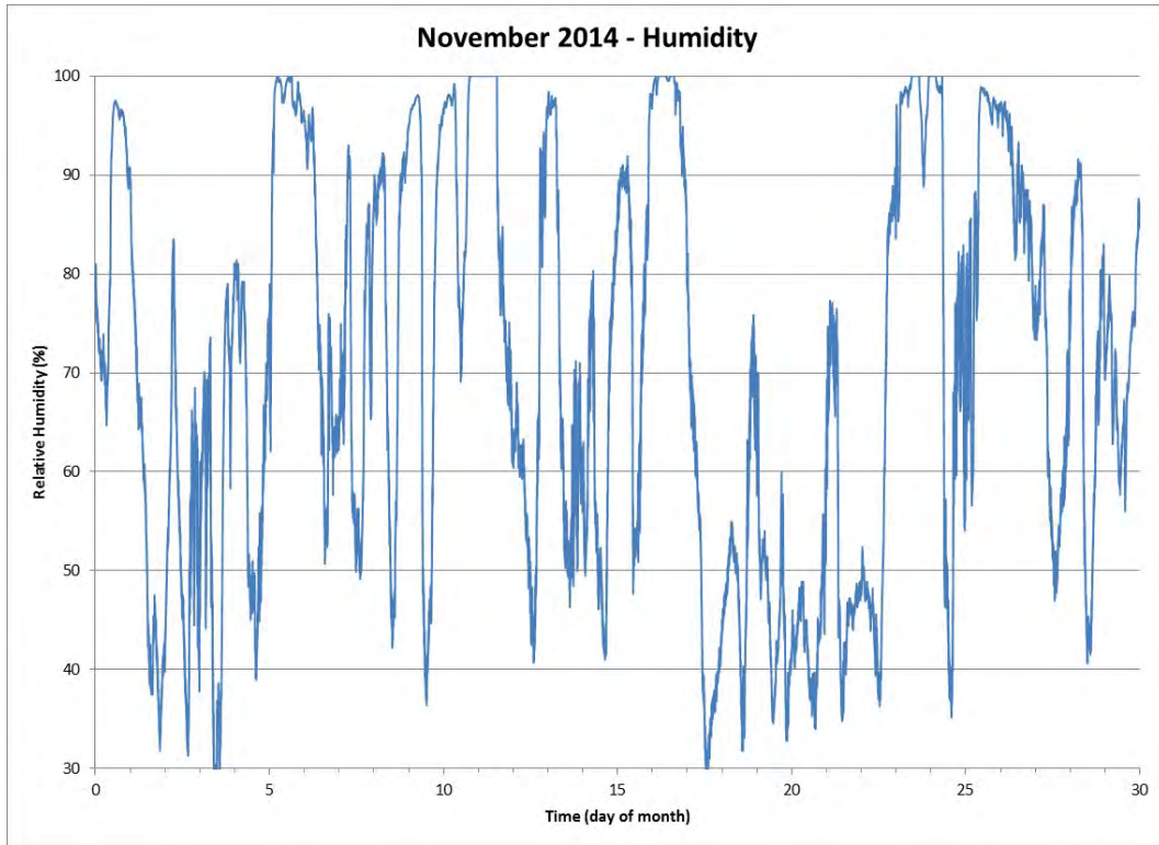
Figure 42 Relative Humidity for the Month of November 2014
