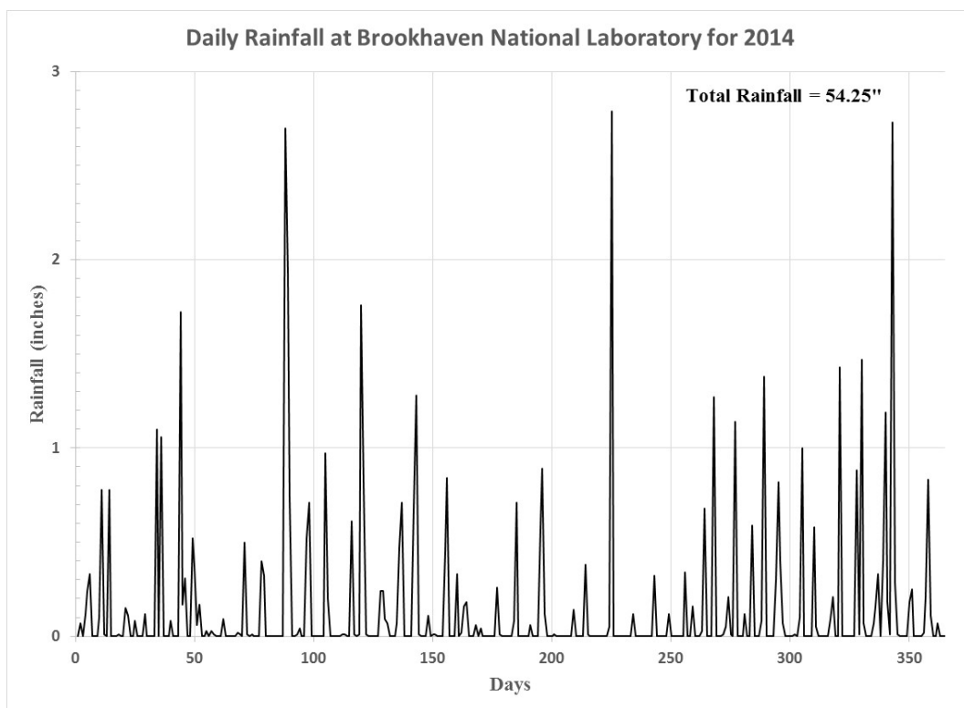
Figure 44 Daily Rainfall Totals at Brookhaven National Laboratory for 2014
