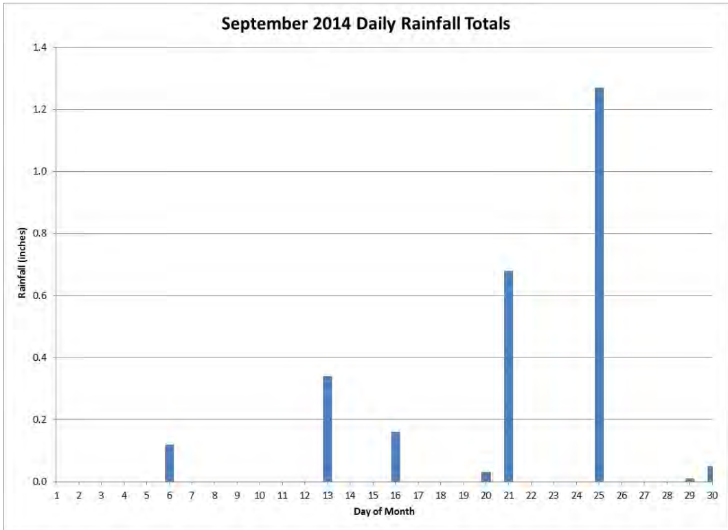
Figure 53 Daily Rainfall for the Month of September 2014
