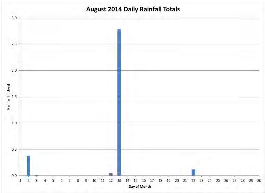
Figure 52 Daily Rainfall for the Month of August 2014
