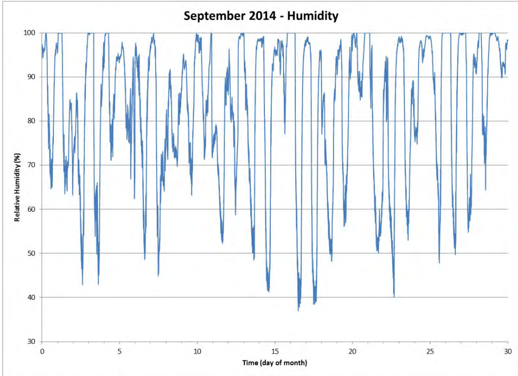
Figure 40 Relative Humidity for the Month of September 2014
