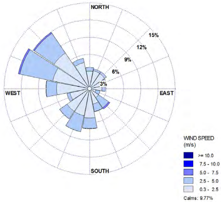
Figure 60 Annual One-hour Wind Roses for the Year 2014 from the 85m level
