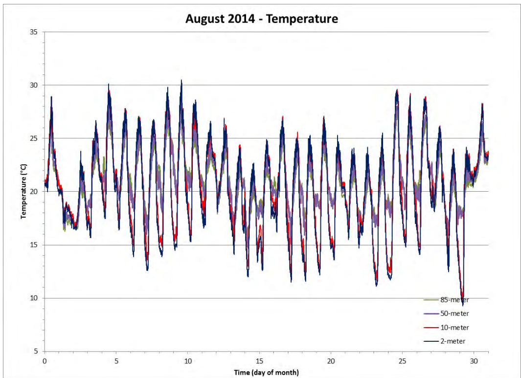
Figure 11 Air Temperature for the Month of August 2014
