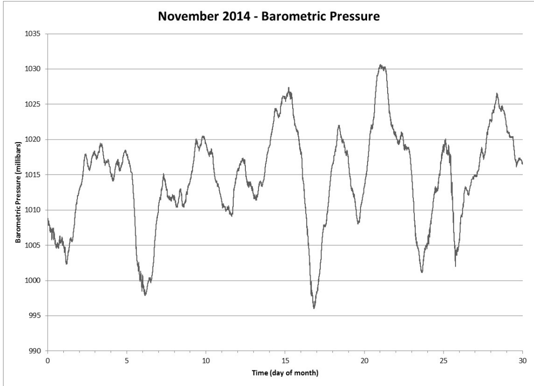
Figure 27 Barometric Pressure for the Month of November 2014
