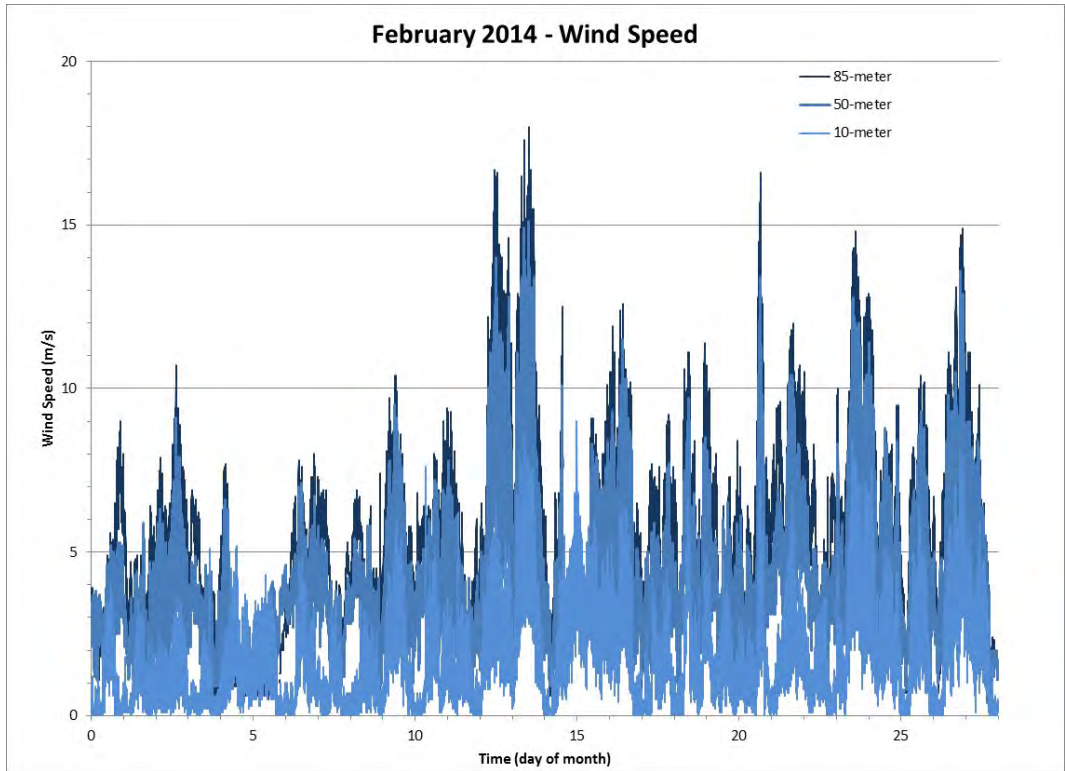
Figure 88 Wind Speed for the Month of February 2014
