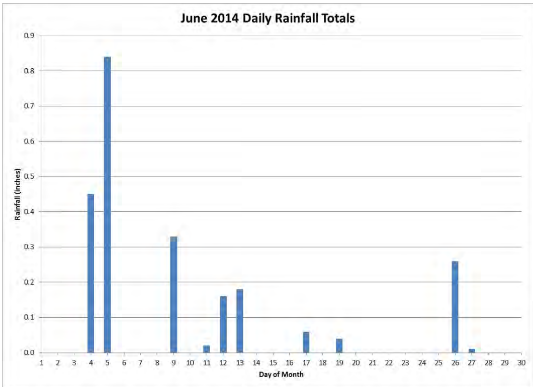
Figure 50 Daily Rainfall for the Month of June 2014
