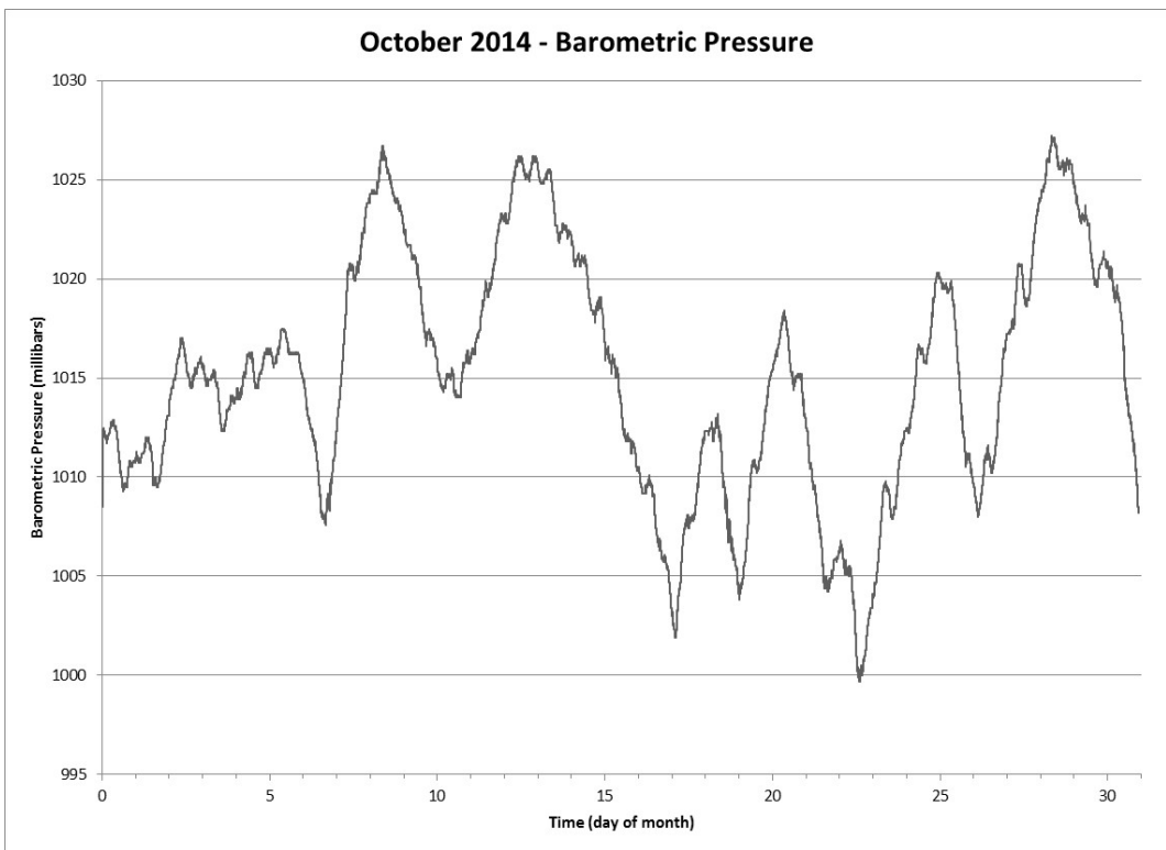
Figure 26 Barometric Pressure for the Month of October 2014
