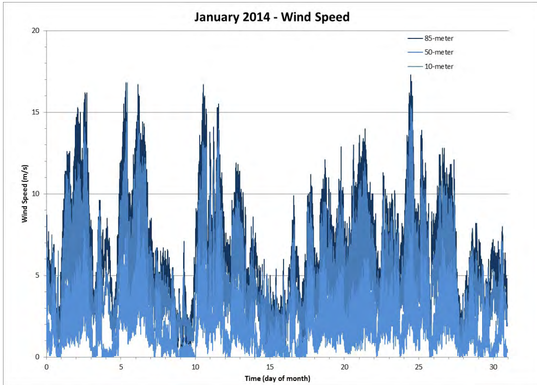
Figure 86 Wind Speed for the Month of January 2014
