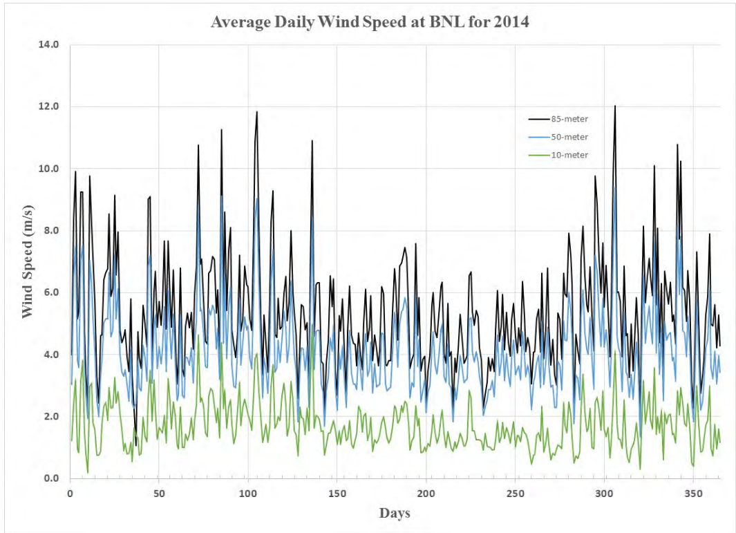
Figure 57 Average Daily Wind Speed (M/s) at the 10-meter, 50-meter and 85-meter heights at Brookhaven National Laboratory for 2014
