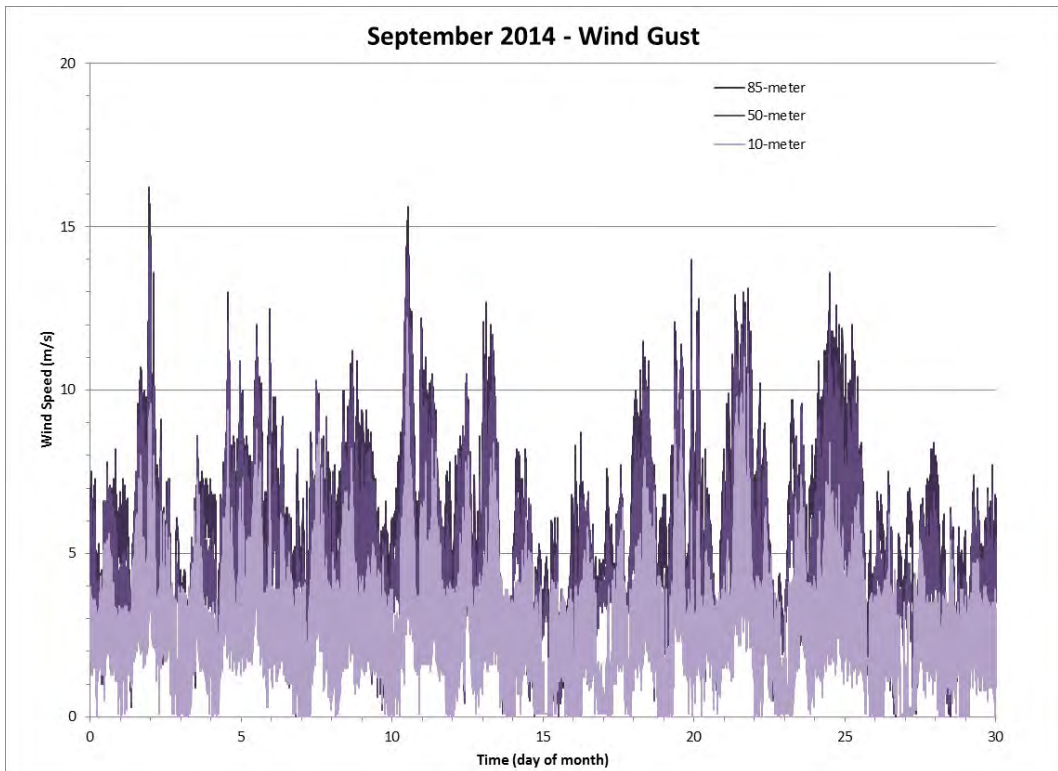
Figure 103 Wind Gust data for the Month of September 2014
