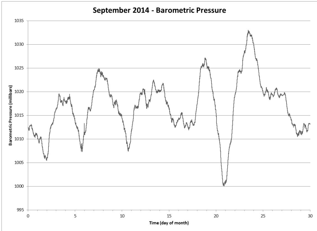
Figure 25 Barometric Pressure for the Month of September 2014
