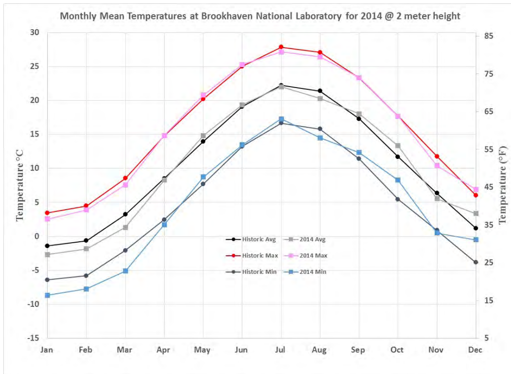
Figure 3 Monthly Mean Temperatures (°C) at Brookhaven National Laboratory for 2014
