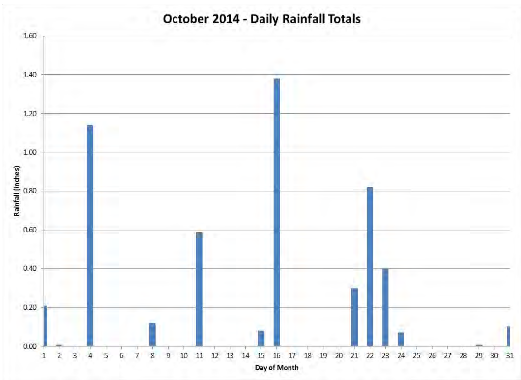
Figure 54 Daily Rainfall for the Month of October 2014
