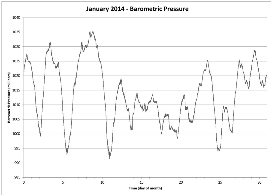
Figure 17 Barometric Pressure for the Month of January 2014
