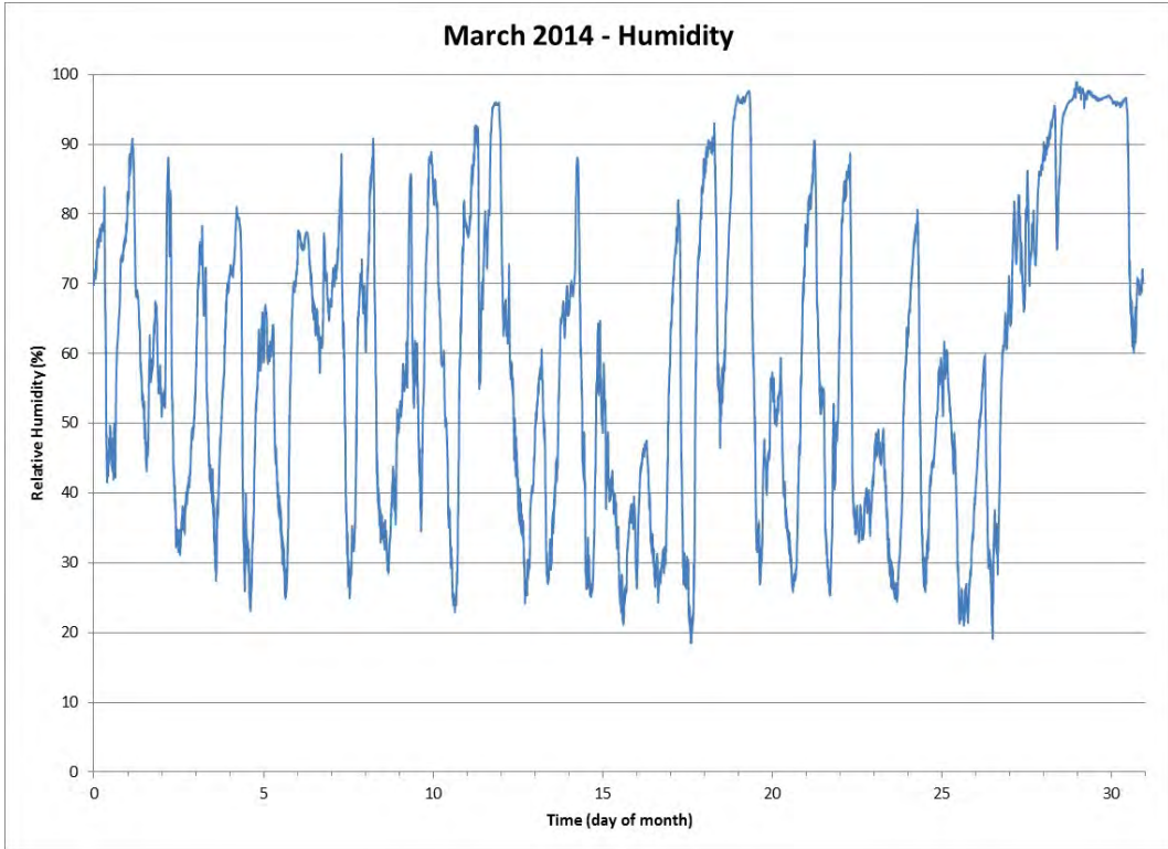
Figure 34 Relative Humidity for the Month of March 2014
