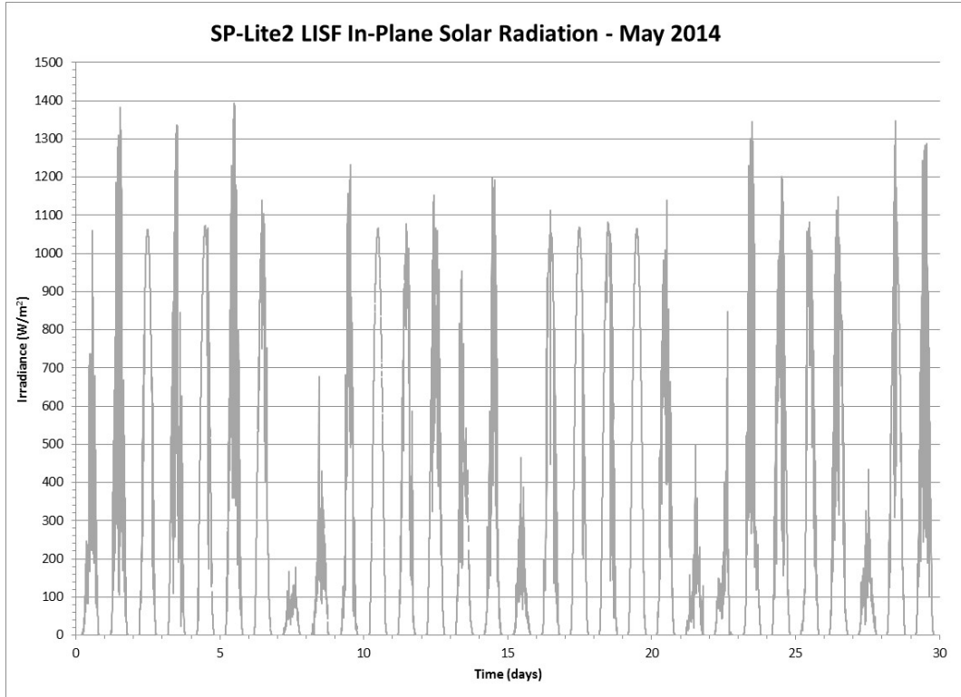
Figure 177 Tilted (27°) Global Solar Radiation from an SP-Lite2 Pyranometer for May 2014
