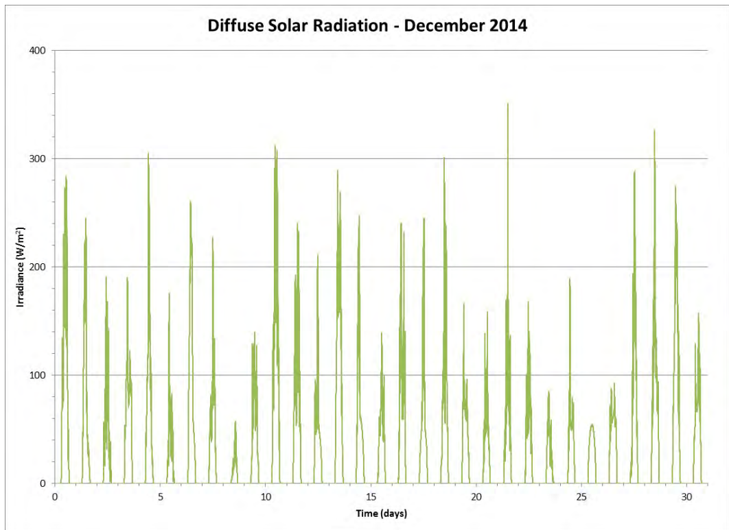
Figure 136 Diffuse Solar Radiation for the Month of December 2014
