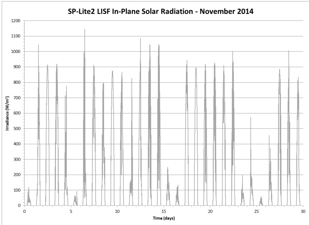
Figure 186 Tilted ( 27^\circ ) Global Solar Radiation from an SP-Lite2 Pyranometer for November 2014
