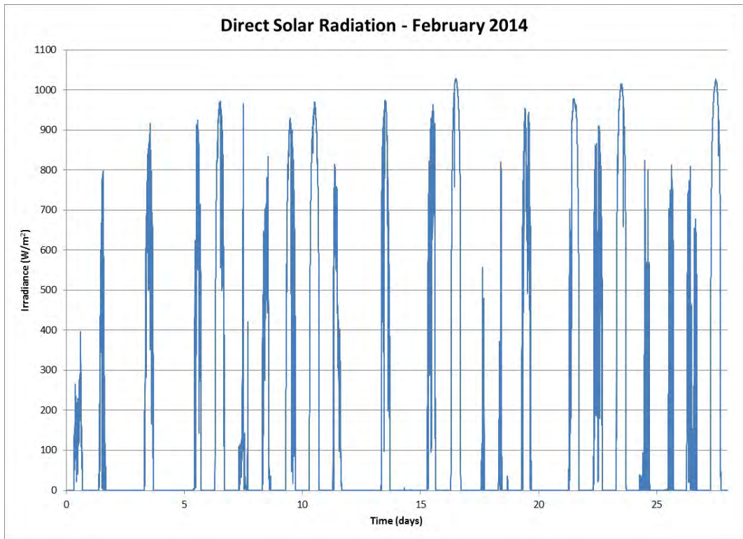
Figure 138 Direct Solar Radiation for the Month of February 2014
