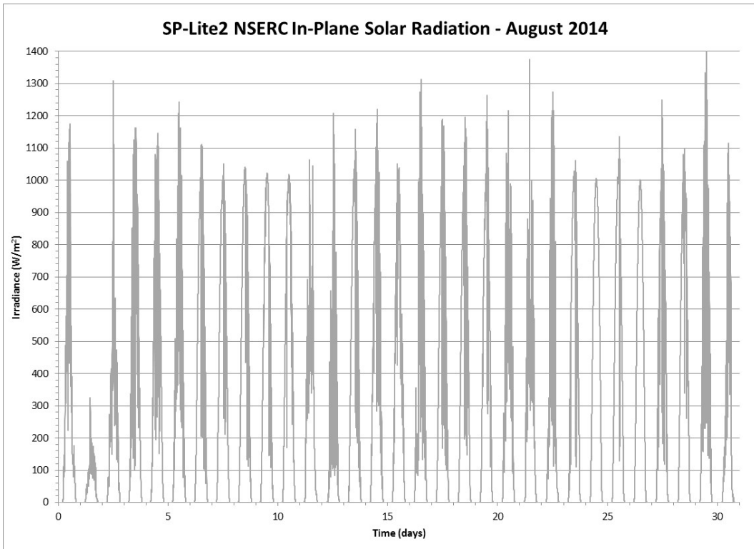
Figure 181 Tilted ( 23^\circ ) Global Solar Radiation from an SP-Lite2 Pyranometer for August 2014
