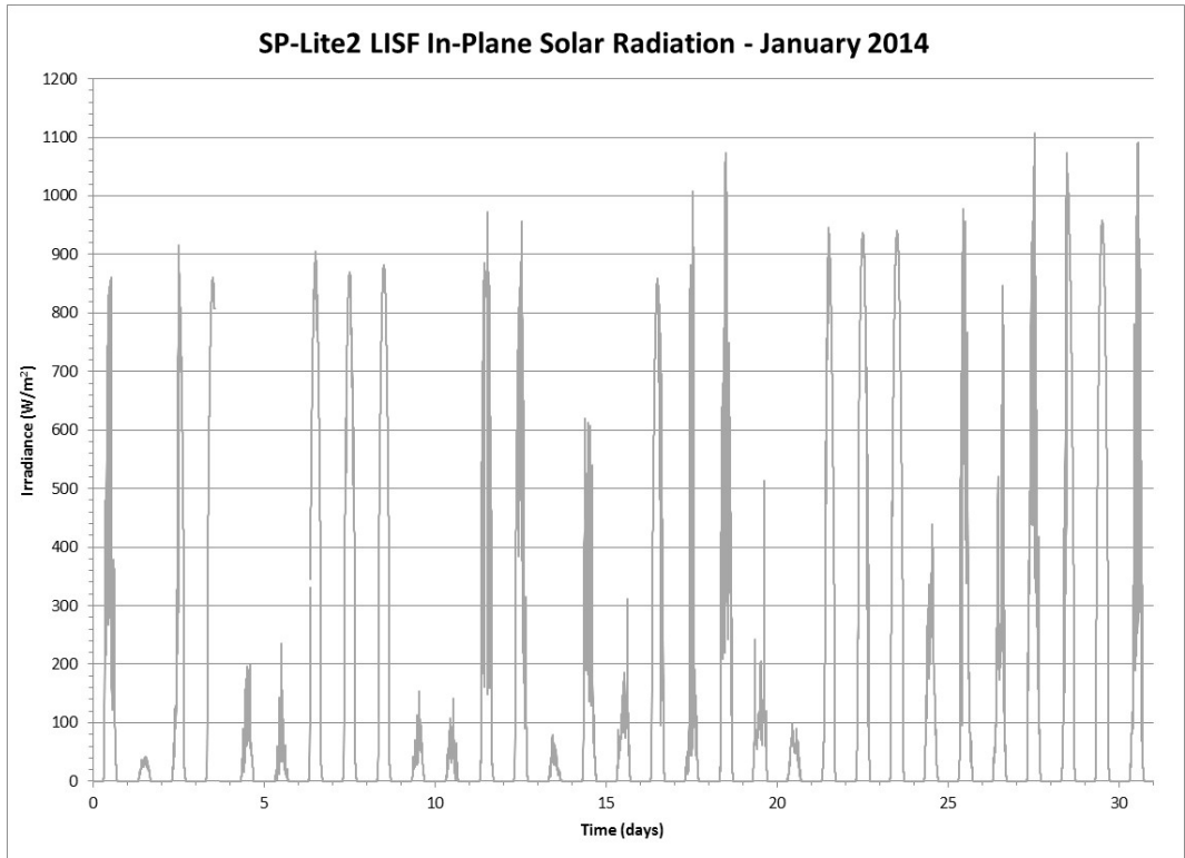
Figure 173 Tilted ( 27^\circ ) Global Solar Radiation from an SP-Lite2 Pyranometer for January 2014
