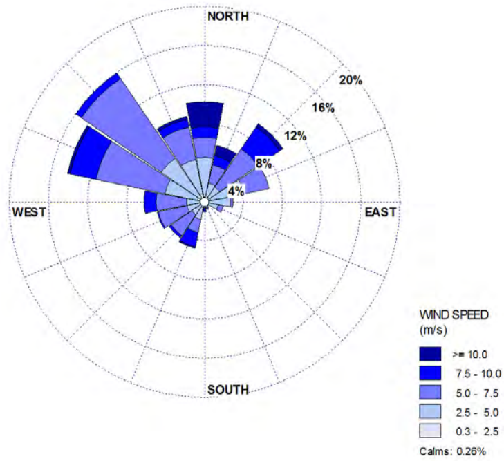
Figure 84 One-hour Wind Roses for the Month of December 2014 from the 85m level
