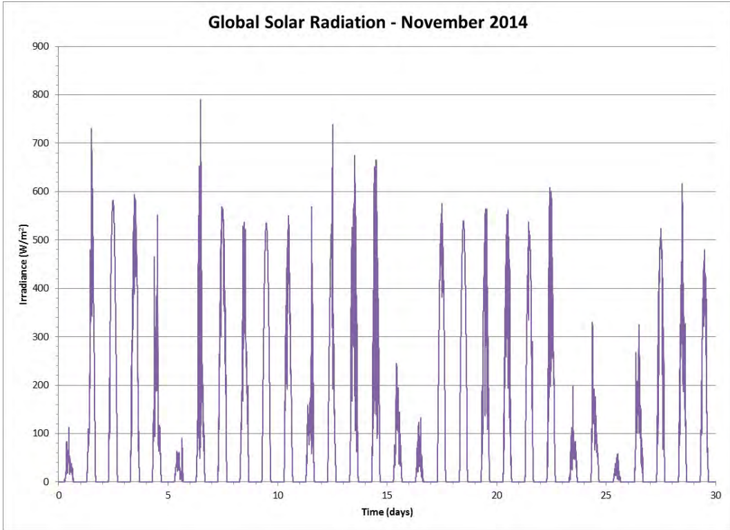
Figure 123 Global Solar Radiation for the Month of November 2014
