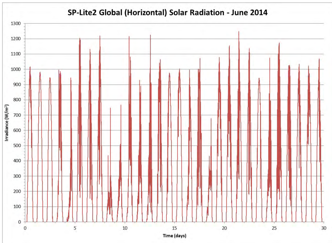
Figure 166 Global Solar Radiation from an SP-Lite2 Pyranometer for the Month of June 2014
