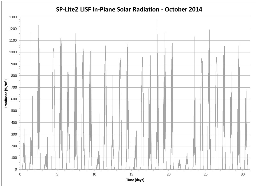
Figure 184 Tilted ( 27^\circ ) Global Solar Radiation from an SP-Lite2 Pyranometer for October 2014
