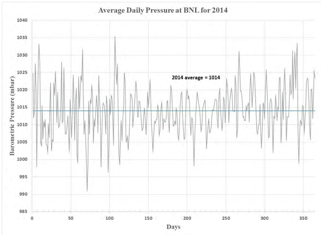
Figure 16 Average Daily Barometric Pressure at Brookhaven National Laboratory for 2014
