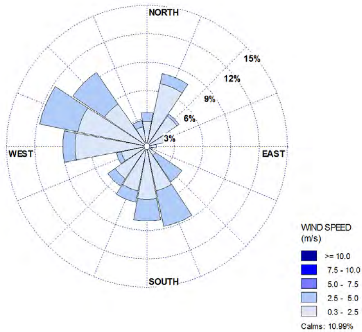
Figure 80 One-hour Wind Roses for the Month of October 2014 from the 85m level
