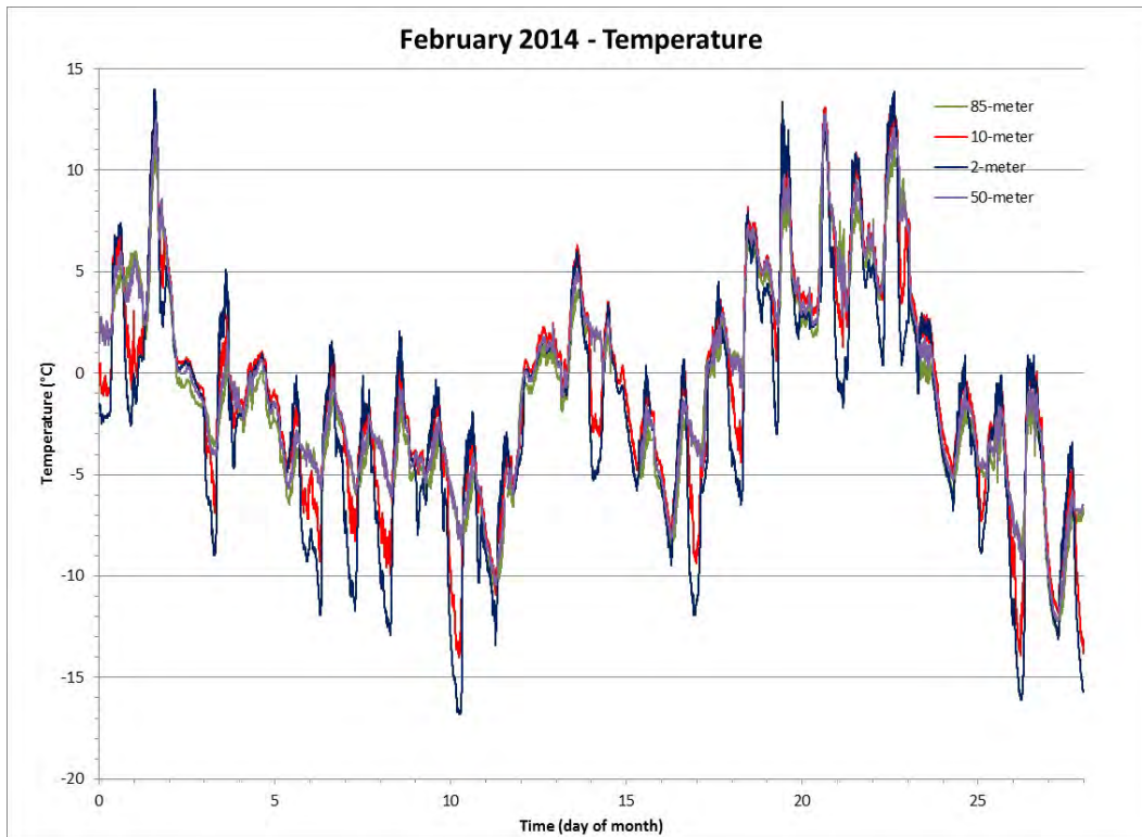
Figure 5 Air Temperature for the Month of February 2014
