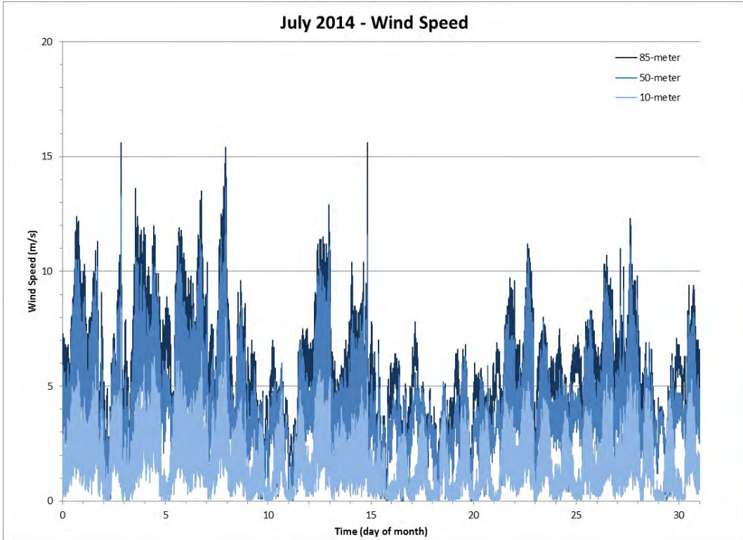
Figure 98 Wind Speed for the Month of July 2014
