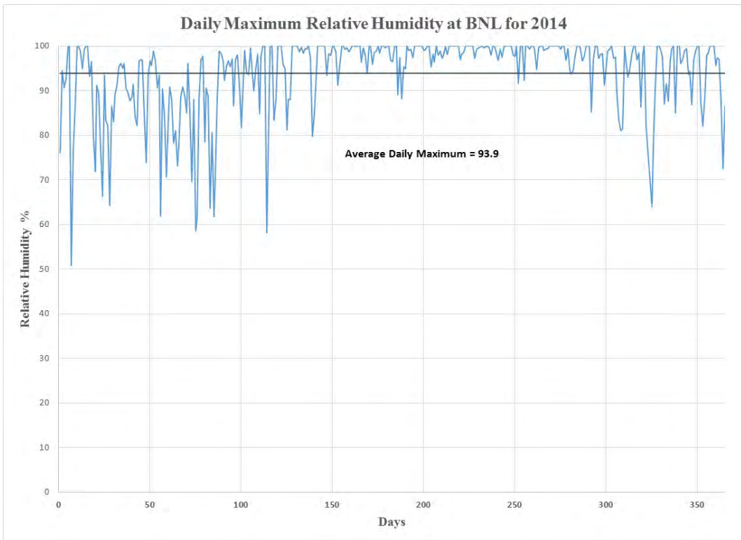
Figure 31 Maximum Daily Humidity at Brookhaven National Laboratory for 2014
