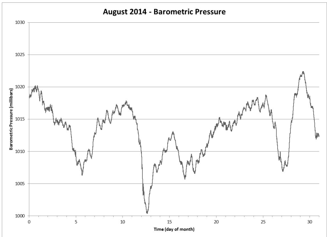
Figure 24 Barometric Pressure for the Month of August 2014
