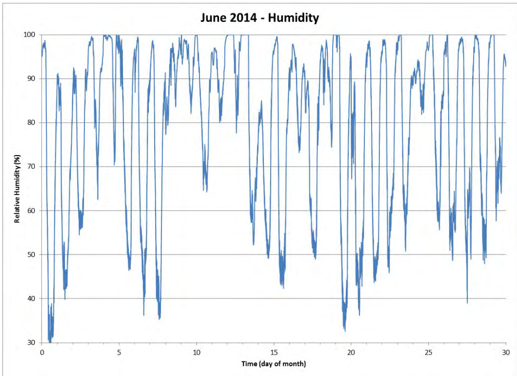
Figure 37 Relative Humidity for the Month of June 2014
