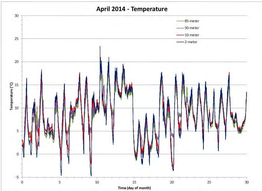
Figure 7 Air Temperature for the Month of April 2014
