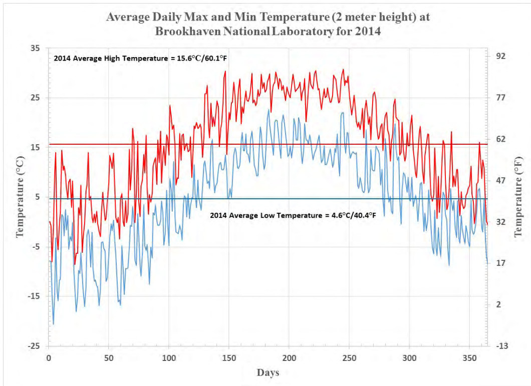
Figure 2 Daily Minimums and Maximums in Temperature taken at the 2 meter height at BNL for 2014
