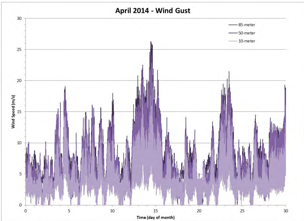
Figure 93 Wind Gust data for the Month of April 2014
