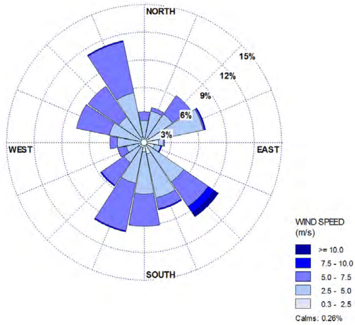
Figure 76 One-hour Wind Roses for the Month of August 2014 from the 85m level
