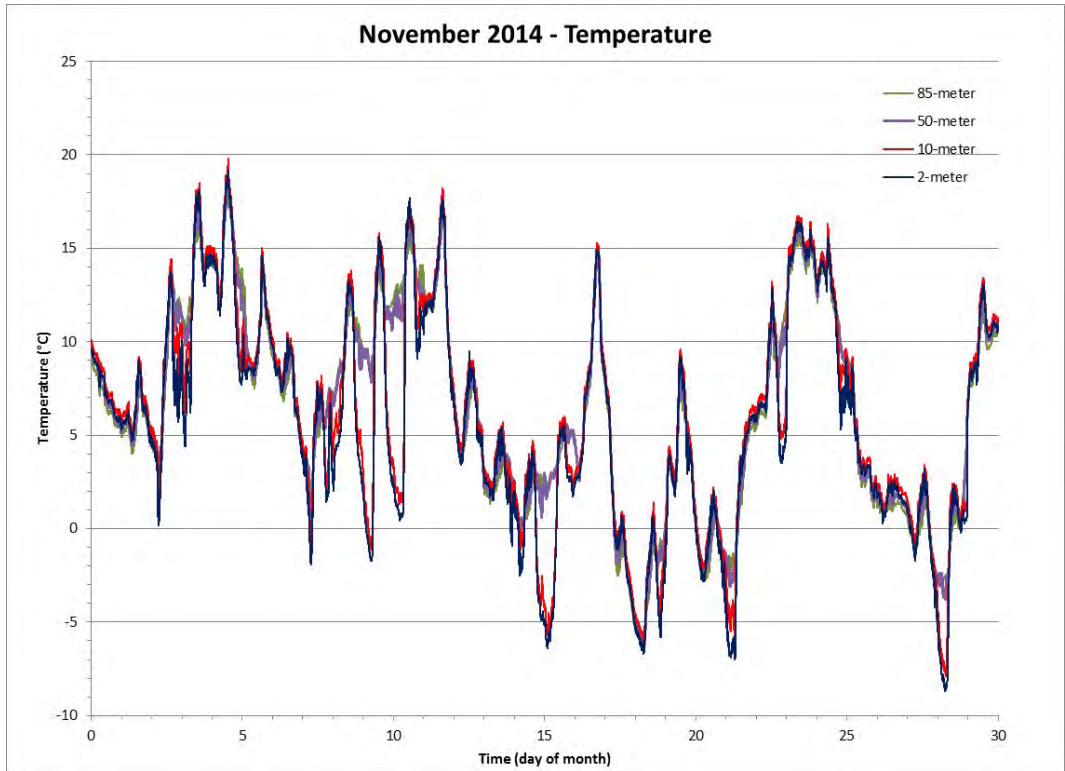
Figure 14 Air Temperature for the Month of November 2014
