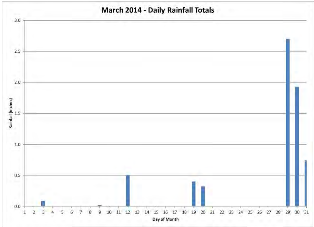
Figure 47 Daily Rainfall for the Month of March 2014
