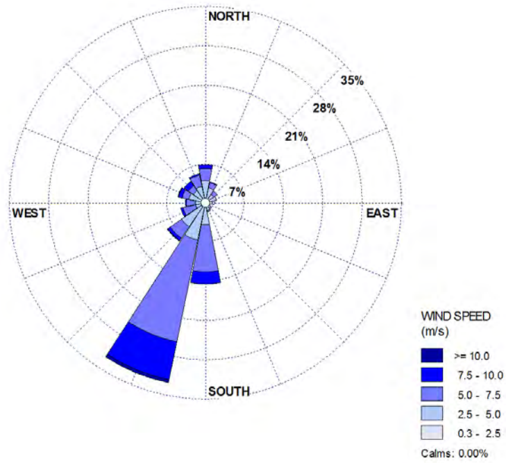
Figure 74 One-hour Wind Roses for the Month of July 2014 from the 85m level
