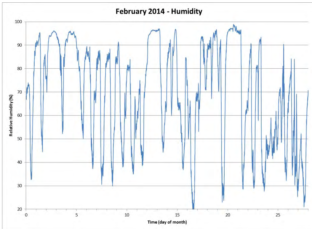
Figure 33 Relative Humidity for the Month of February 2014
