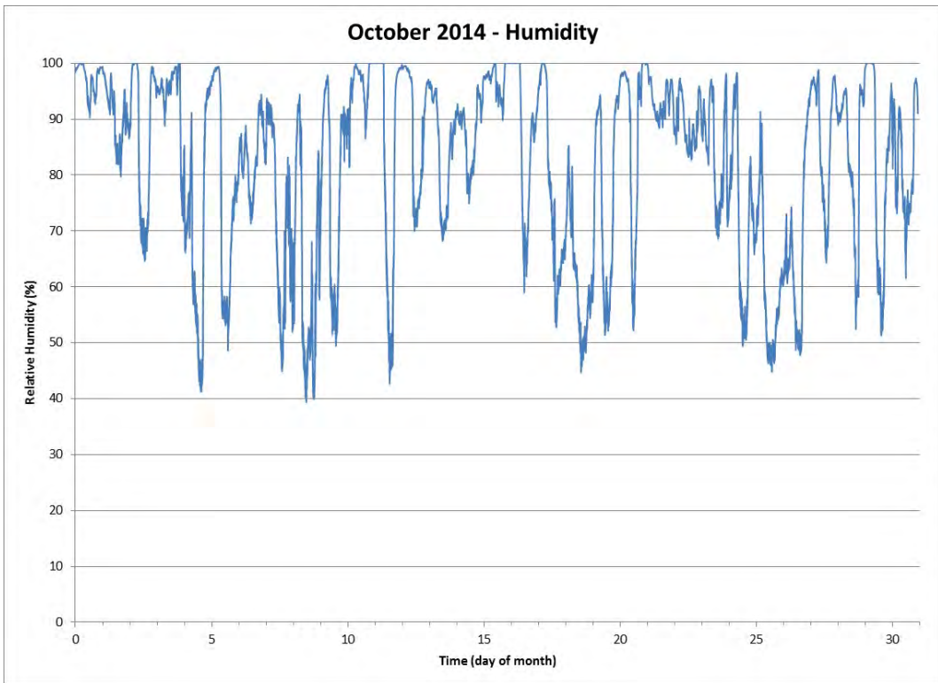
Figure 41 Relative Humidity for the Month of October 2014
