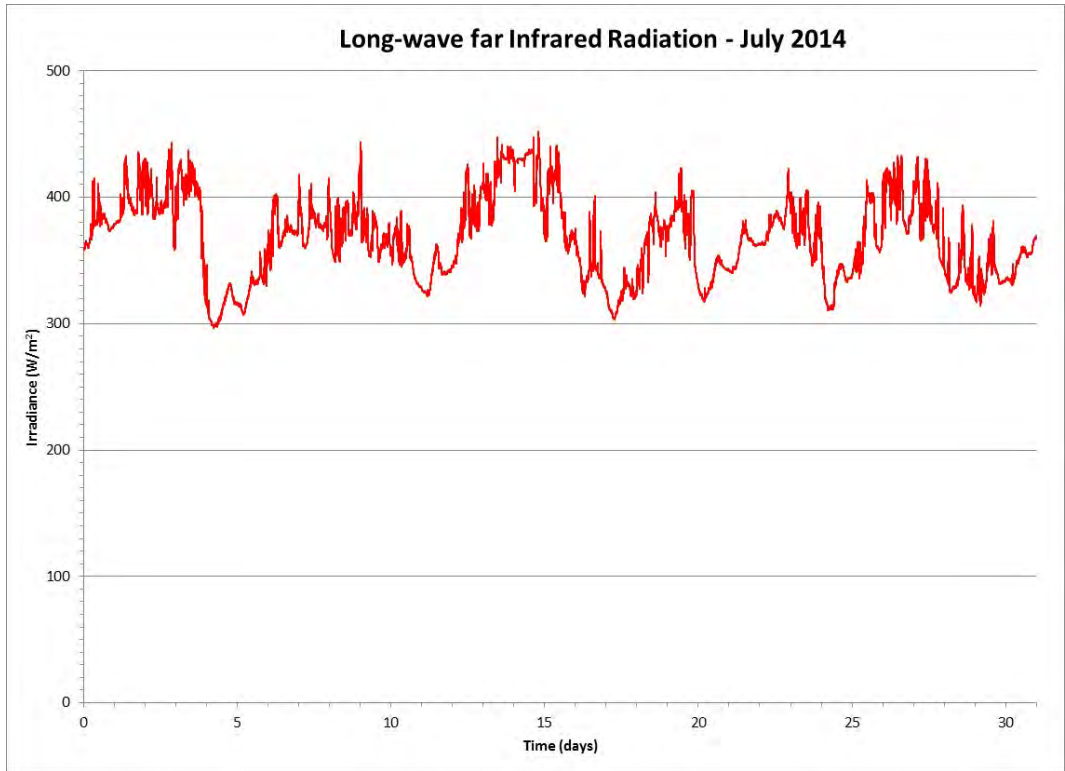
Figure 155 Long-wave Far Infrared Radiation for the Month of July 2014
