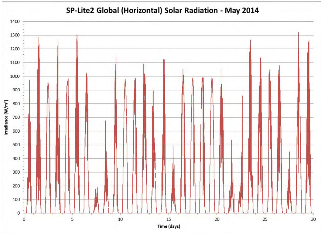
Figure 165 Global Solar Radiation from an SP-Lite2 Pyranometer for the Month of May 2014
