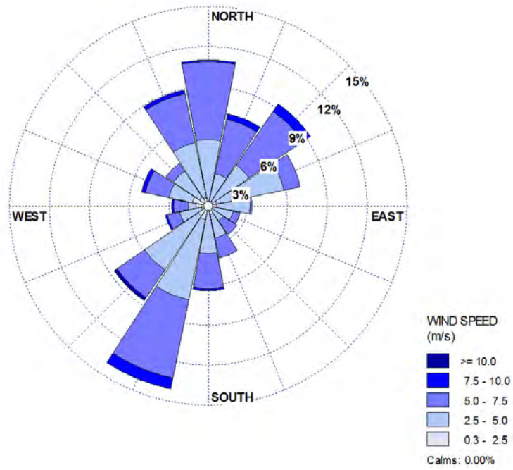
Figure 78 One-hour Wind Roses for the Month of September 2014 from the 85m level
