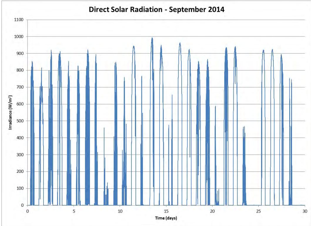
Figure 145 Direct Solar Radiation for the Month September 2014
