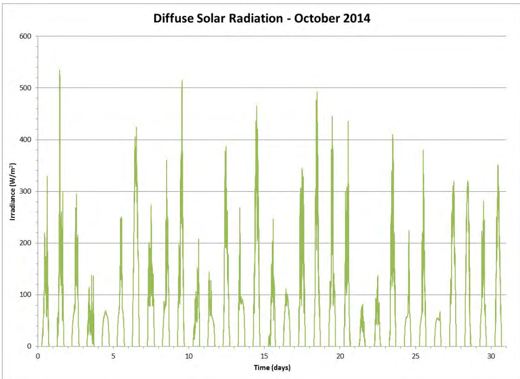
Figure 134 Diffuse Solar Radiation for the Month of October 2014
