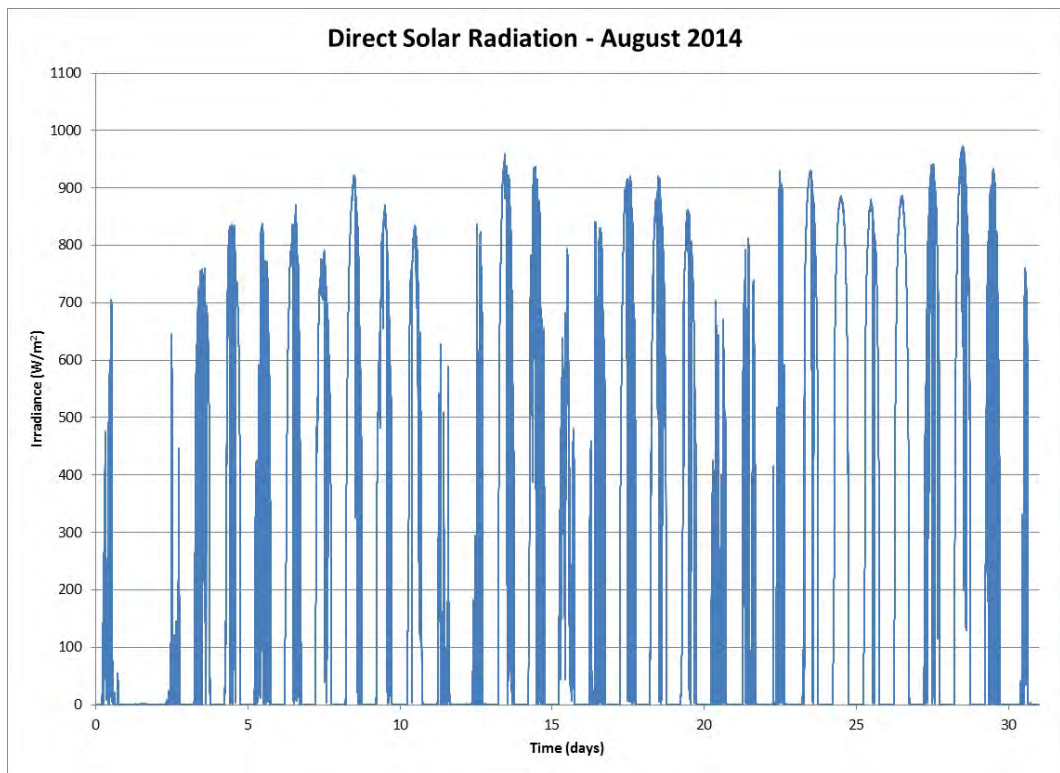
Figure 144 Direct Solar Radiation for the Month August 2014
