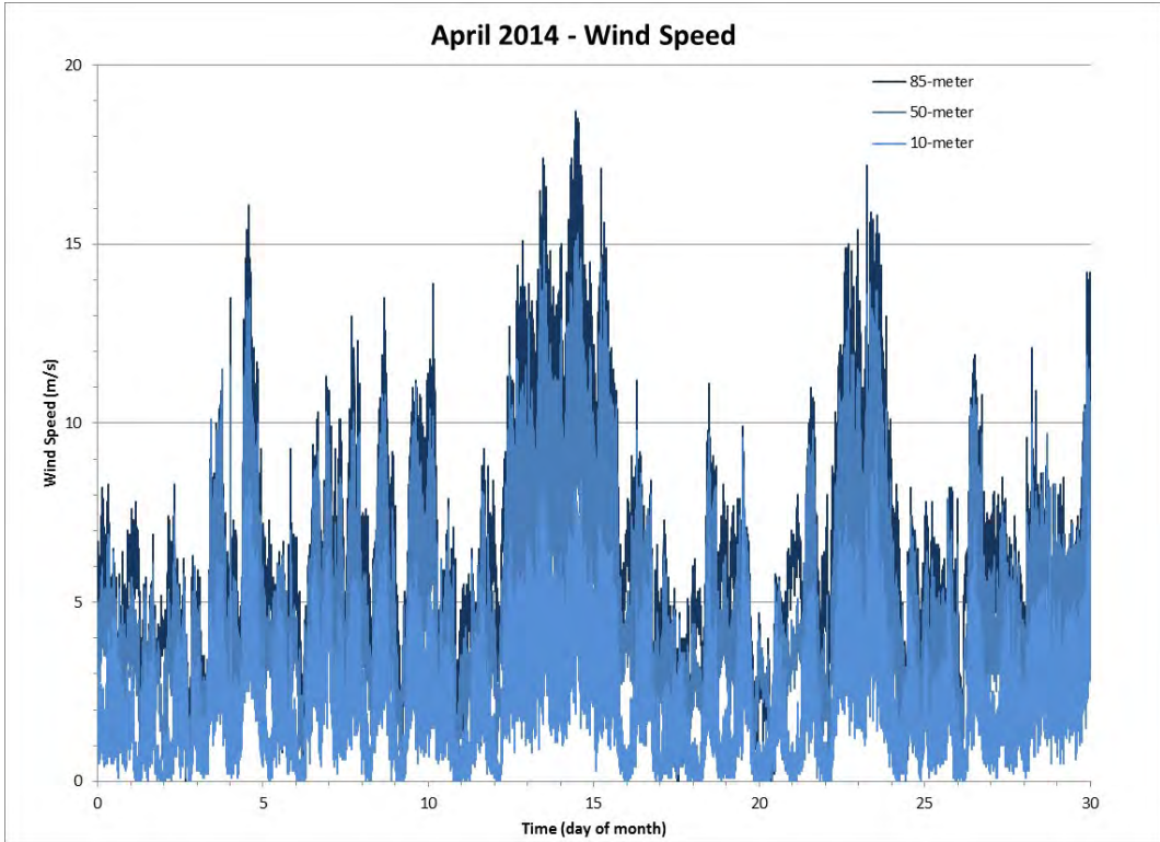
Figure 92 Wind Speed for the Month of April 2014
