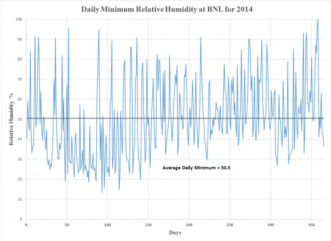
Figure 30 Minimum Daily Humidity at Brookhaven National Laboratory for 2014
