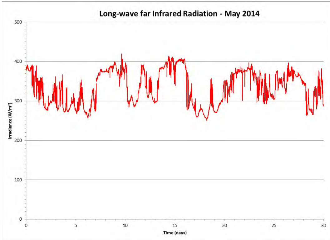
Figure 153 Long-wave Far Infrared Radiation for the Month of May 2014
