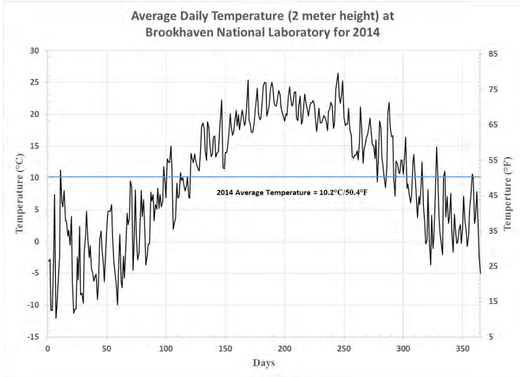
Figure 1 Average Daily Temperature taken at the 2 meter height at BNL for 2014
