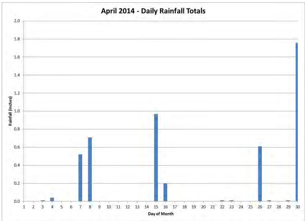
Figure 48 Daily Rainfall for the Month of April 2014
