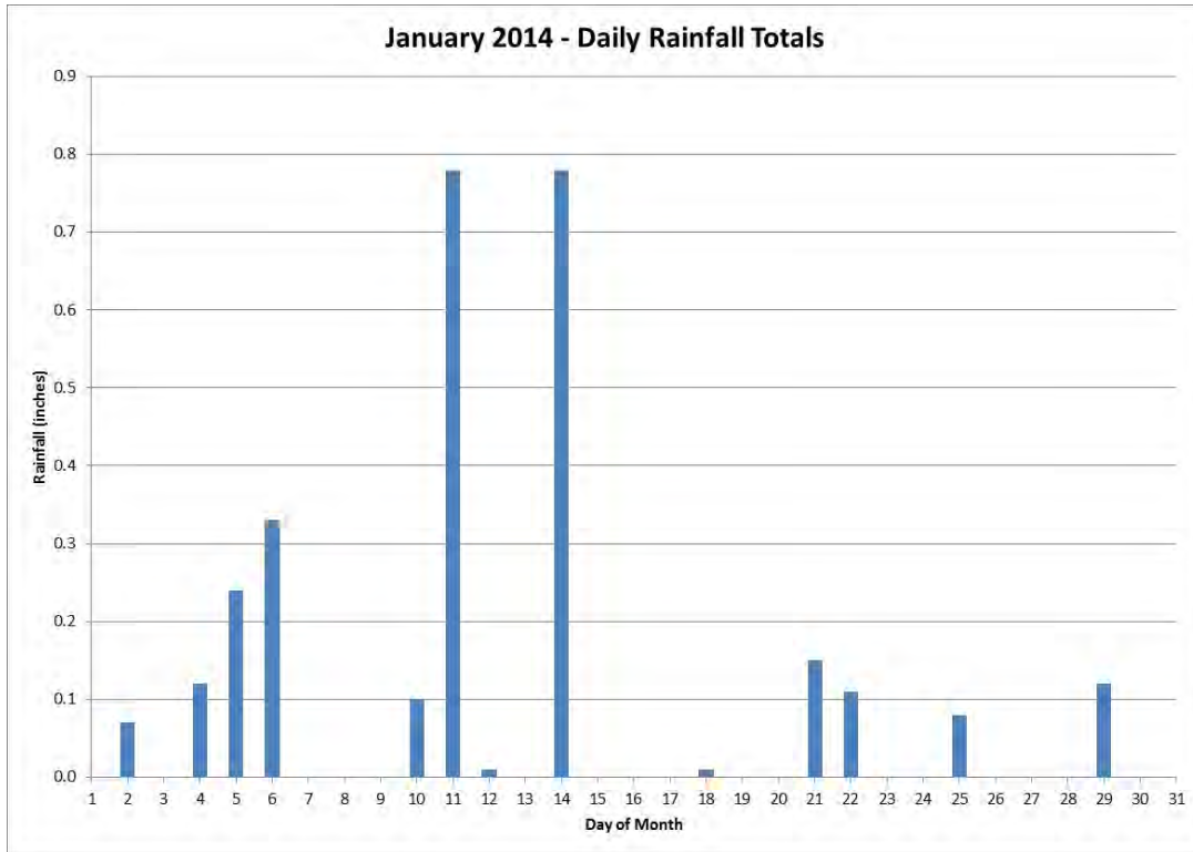
Figure 45 Daily Rainfall for the Month of January 2014
