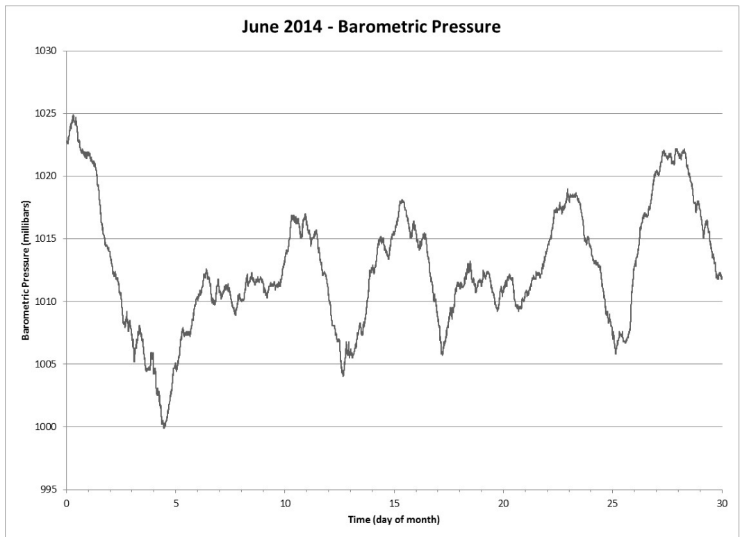
Figure 22 Barometric Pressure for the Month of June 2014
