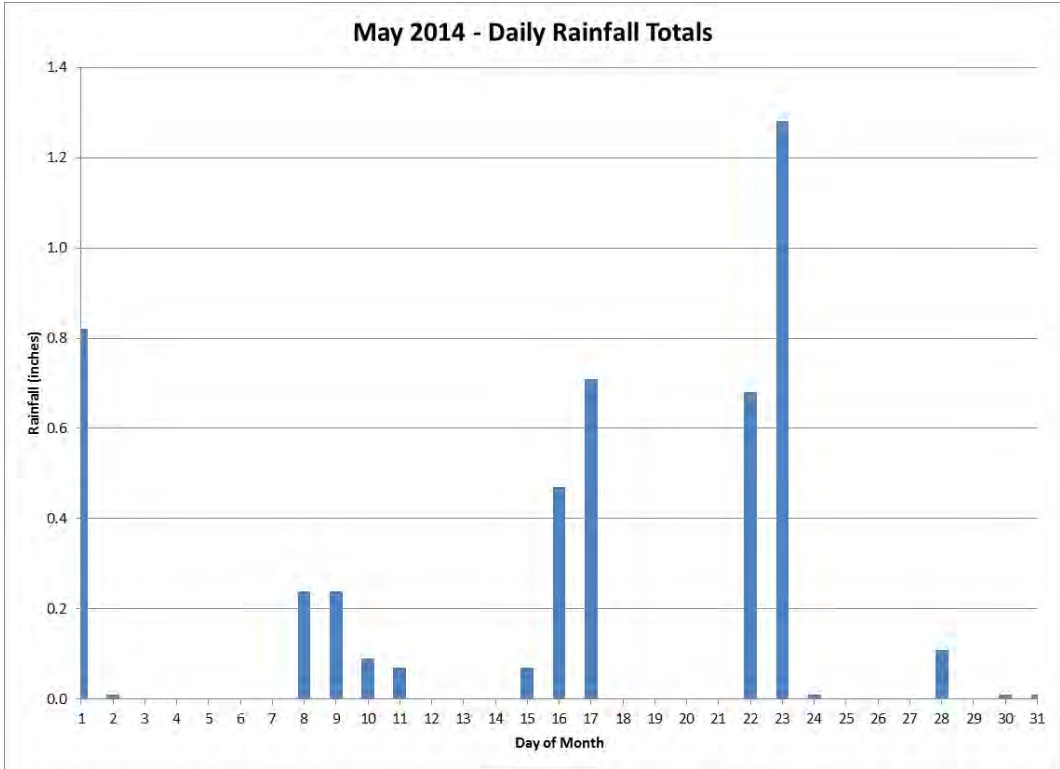
Figure 49 Daily Rainfall for the Month of May 2014
