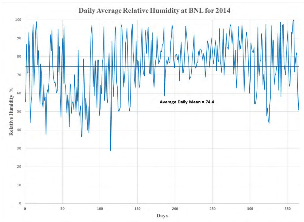
Figure 29 Daily Mean Relative Humidity at Brookhaven National Laboratory for 2014
