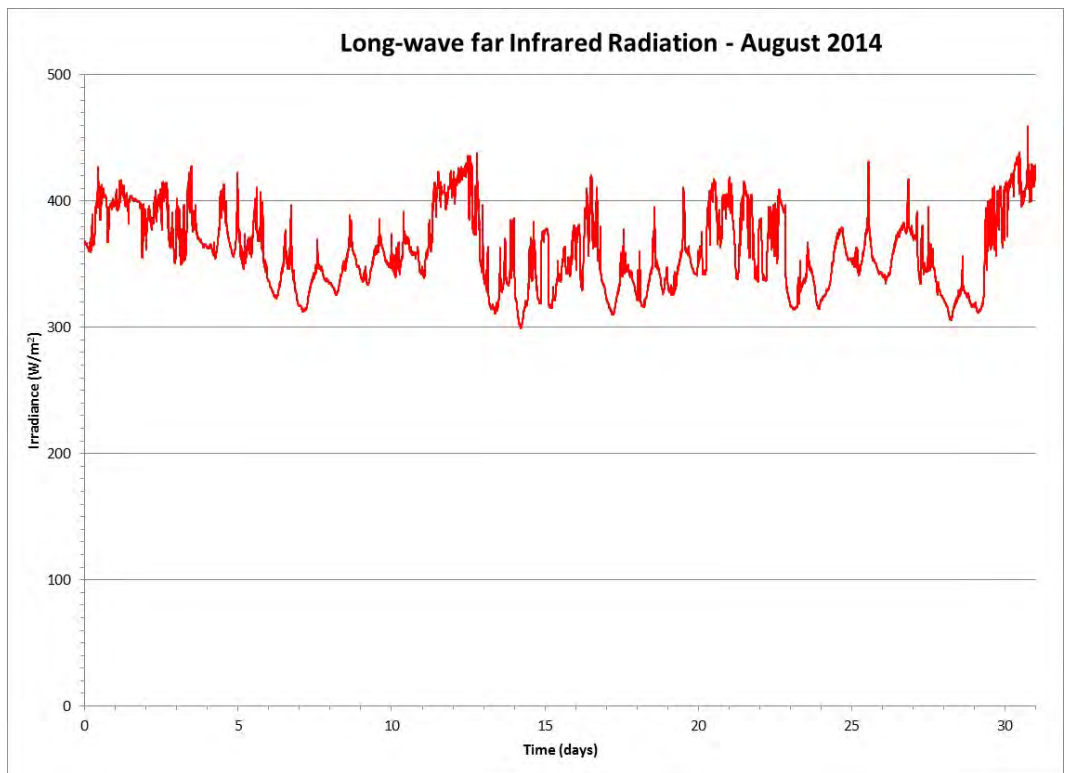
Figure 156 Long-wave Far Infrared Radiation for the Month of August 2014
