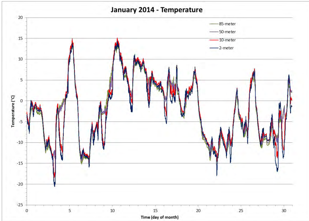
Figure 4 Air Temperature for the Month of January 2014
