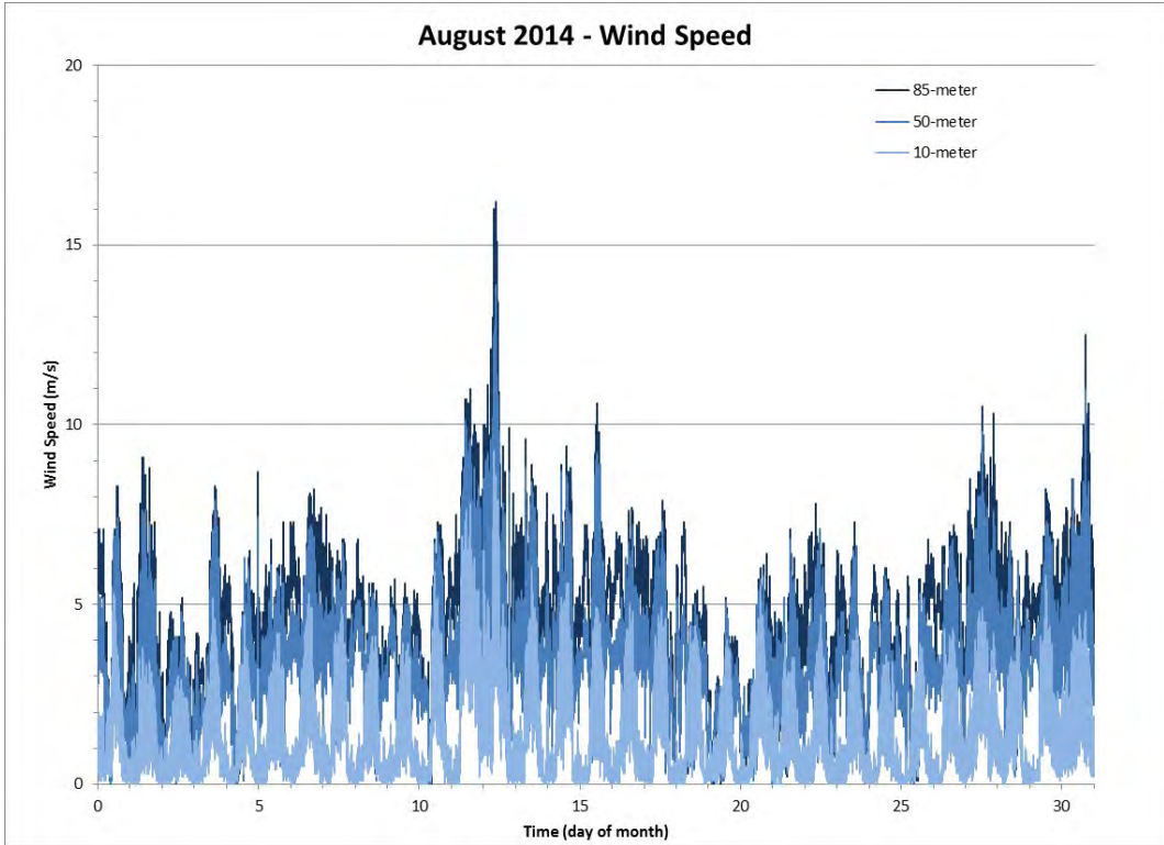
Figure 100 Wind Speed for the Month of August 2014
