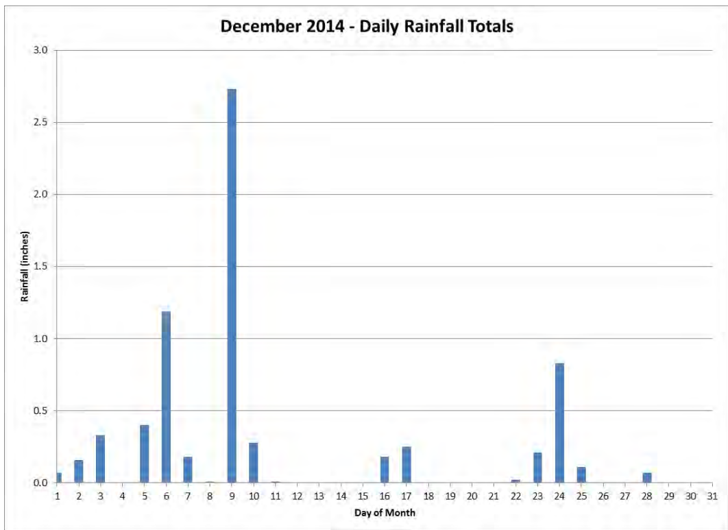
Figure 56 Daily Rainfall for the Month of December 2014
