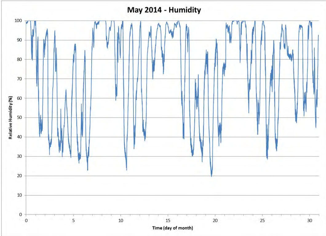
Figure 36 Relative Humidity for the Month of May 2014
