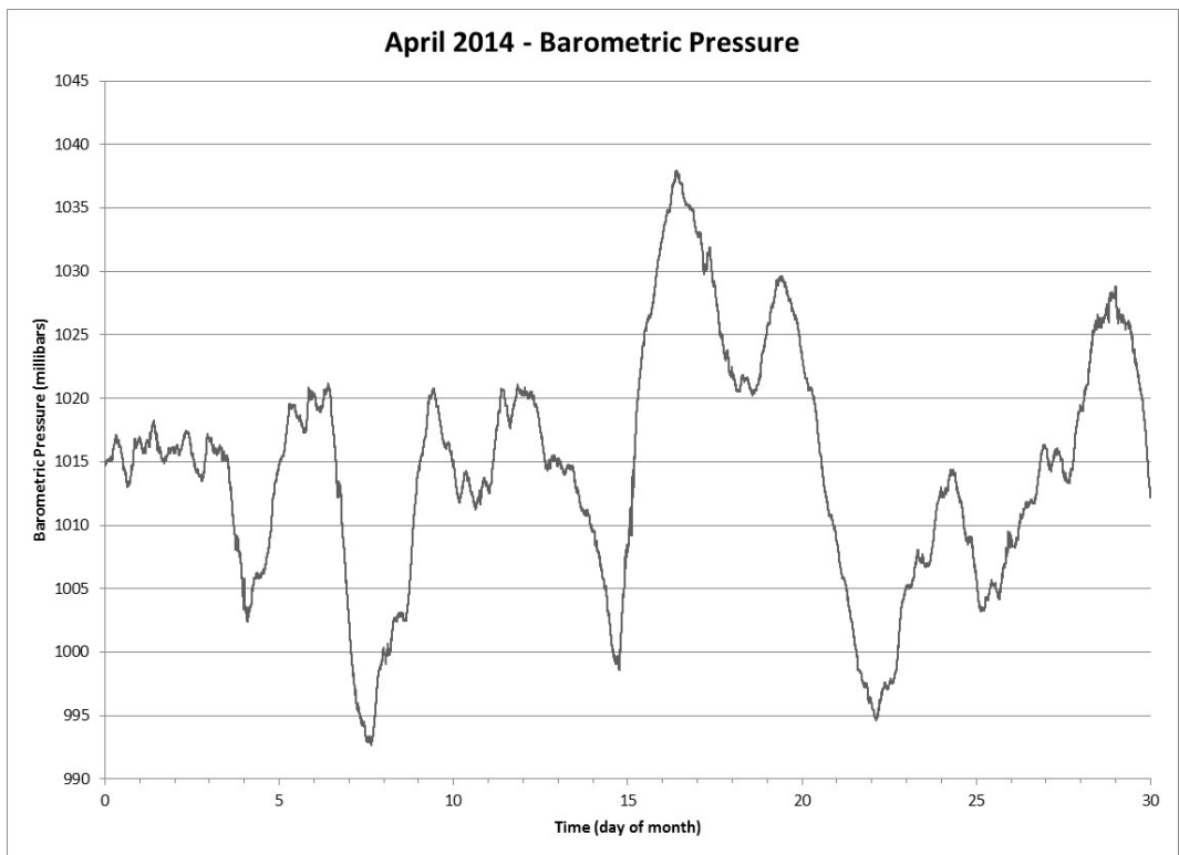
Figure 20 Barometric Pressure for the Month of April 2014
