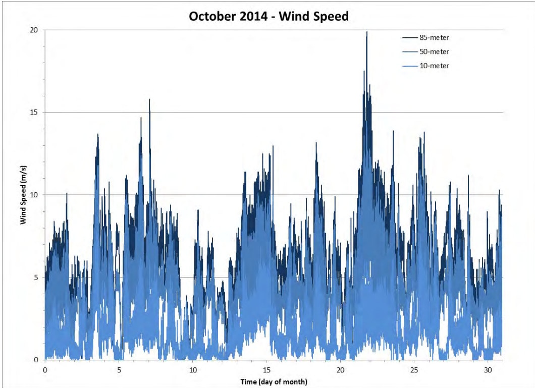
Figure 104 Wind Speed for the Month of October 2014
