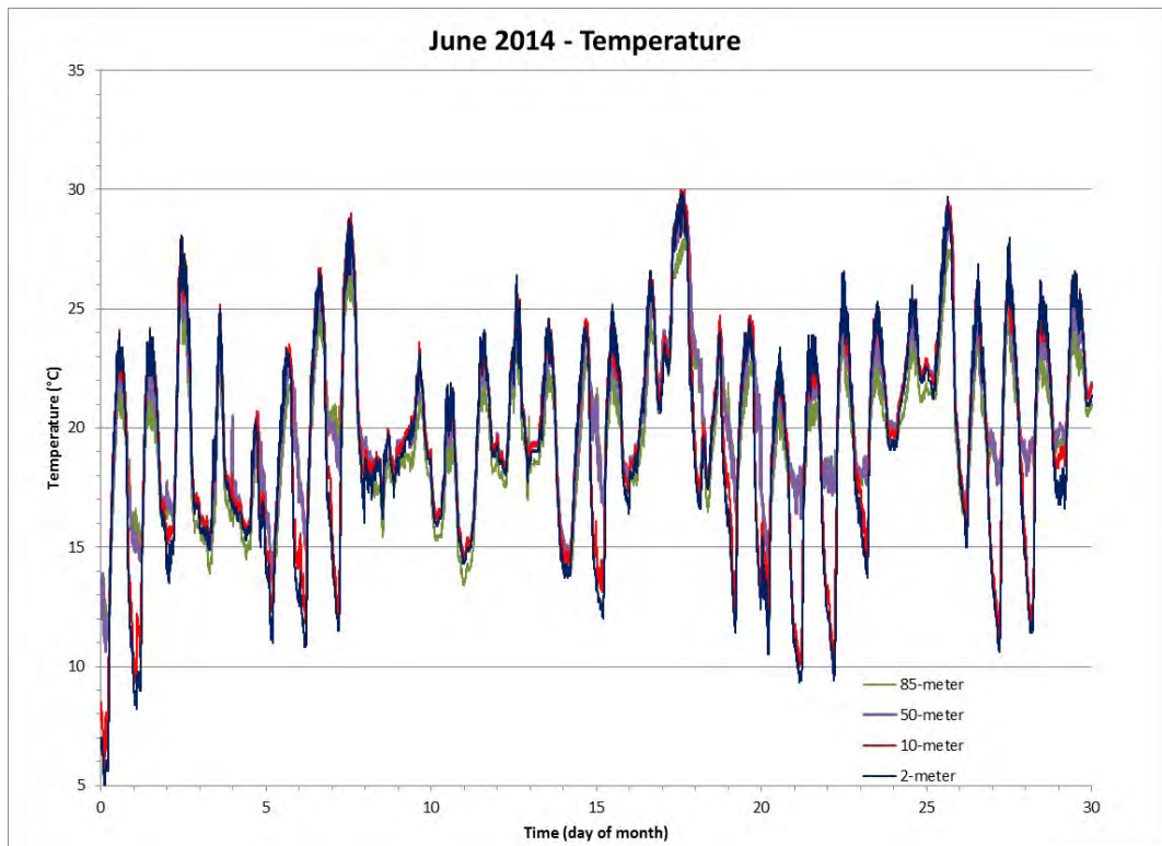
Figure 9 Air Temperature for the Month of June 2014
