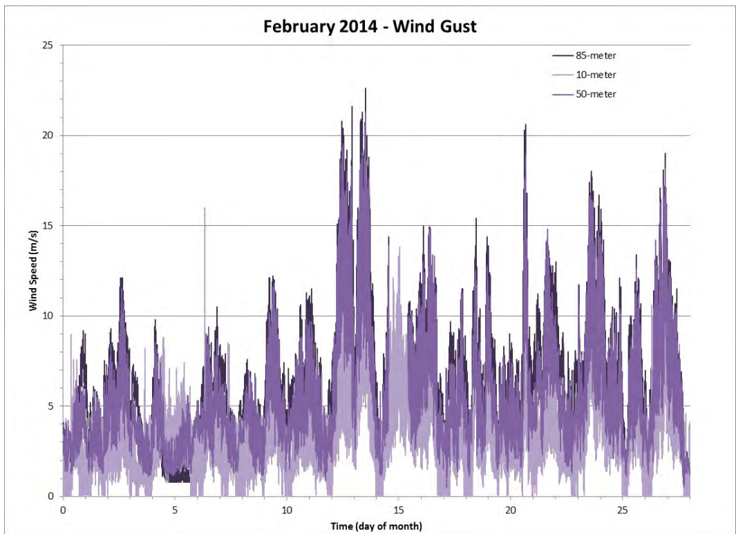
Figure 89 Wind Gust data for the Month of February 2014
