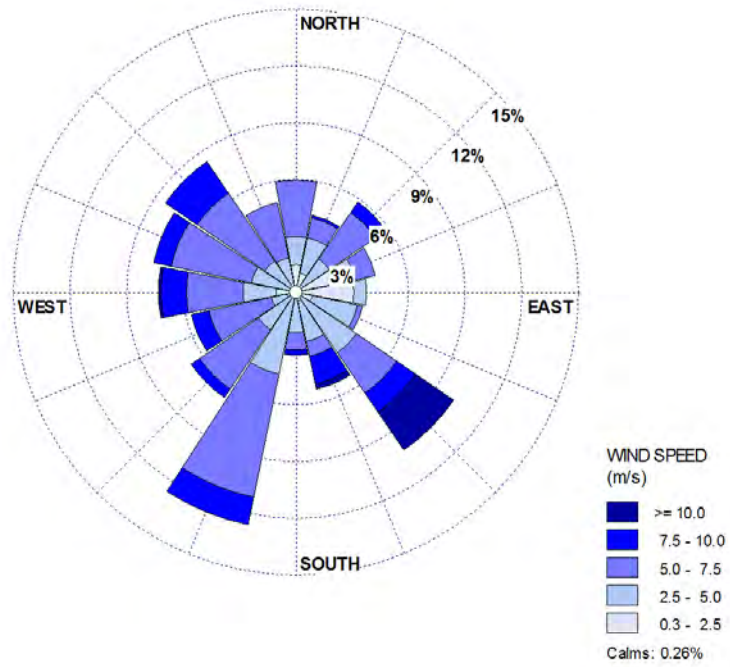
Figure 70 One-hour Wind Roses for the Month of May 2014 from the 85m level
