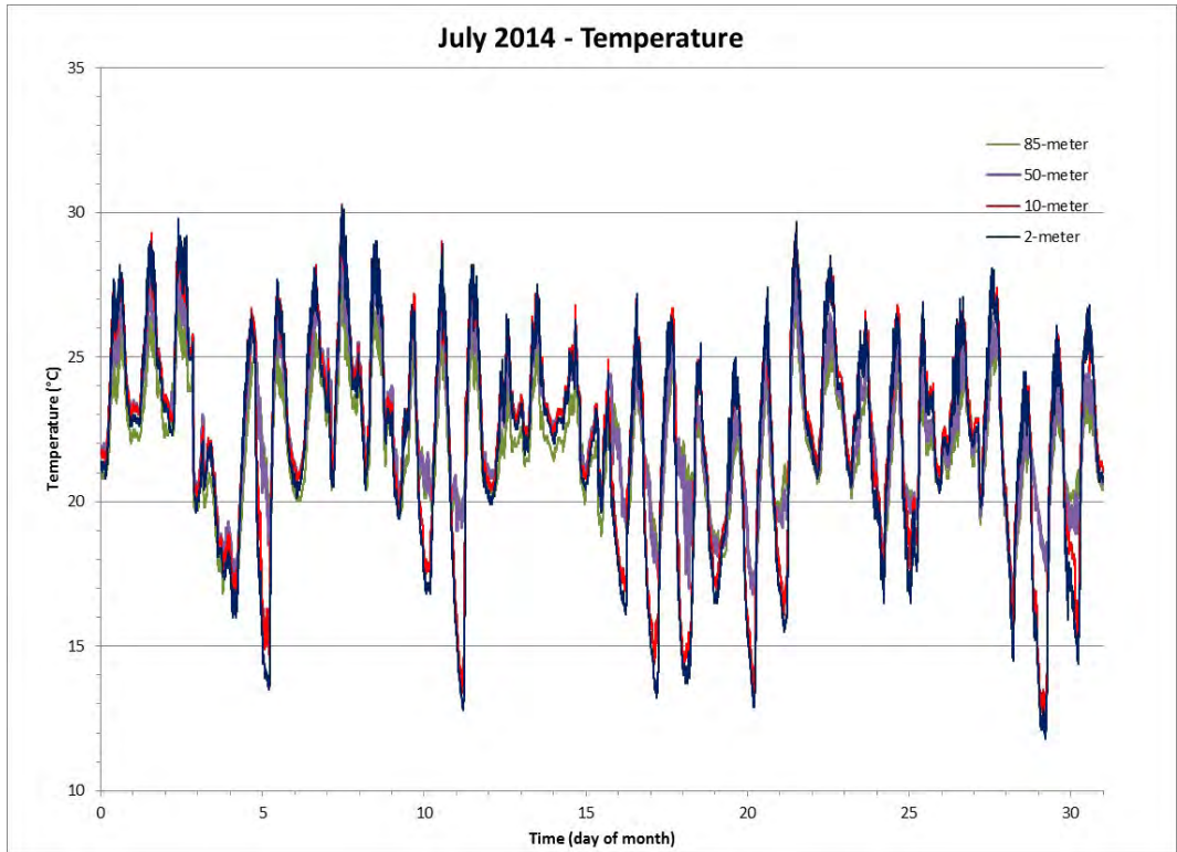
Figure 10 Air Temperature for the Month of July 2014
