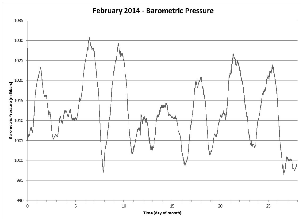
Figure 18 Barometric Pressure for the Month of February 2014
