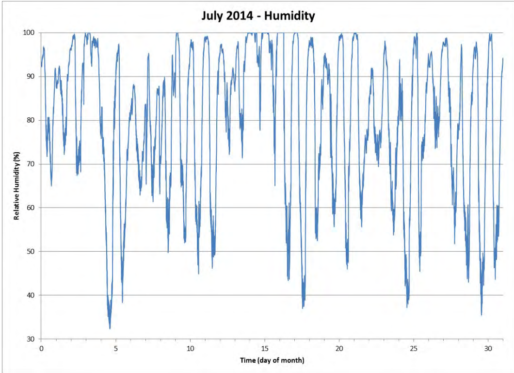
Figure 38 Relative Humidity for the Month of July 2014
