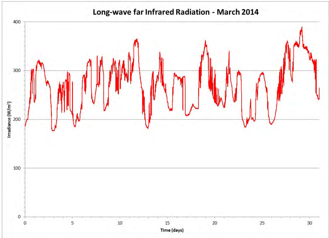
Figure 151 Long-wave Far Infrared Radiation for the Month of March 2014
