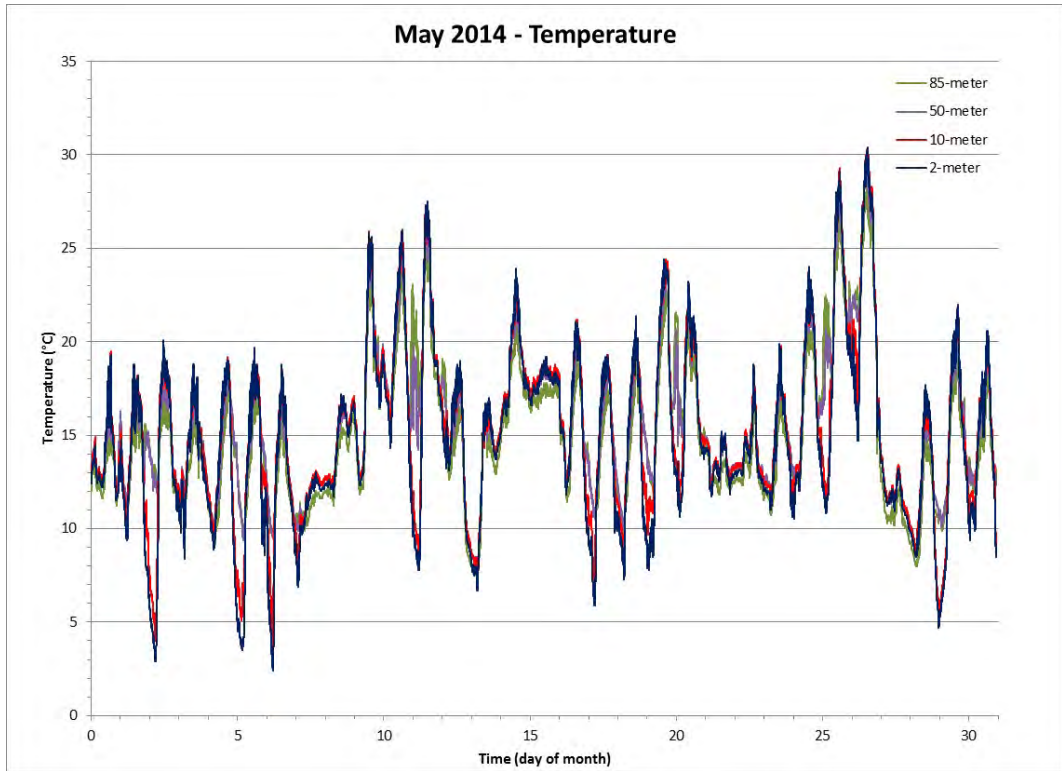
Figure 8 Air Temperature for the Month of May 2014
