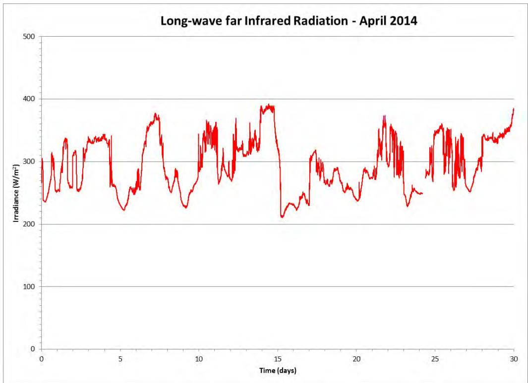
Figure 152 Long-wave Far Infrared Radiation for the Month of April 2014
