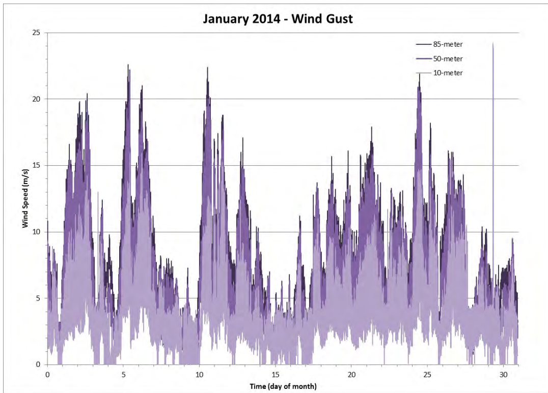
Figure 87 Wind Gust data for the Month of January 2014
