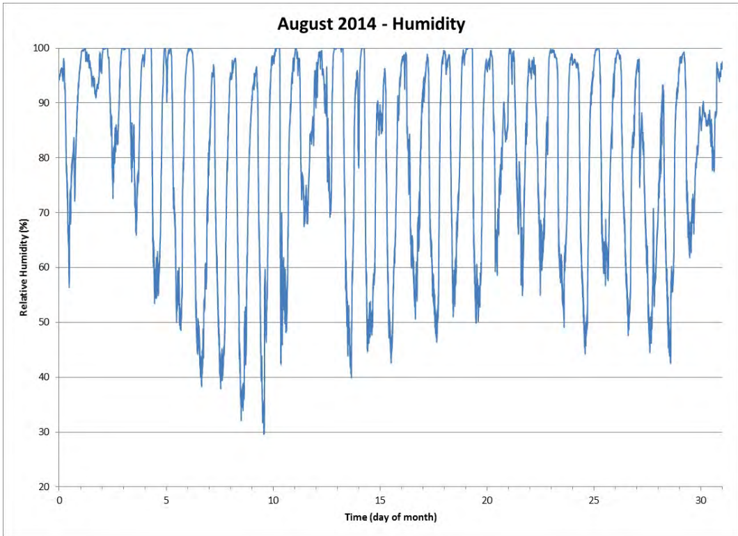
Figure 39 Relative Humidity for the Month of August 2014
