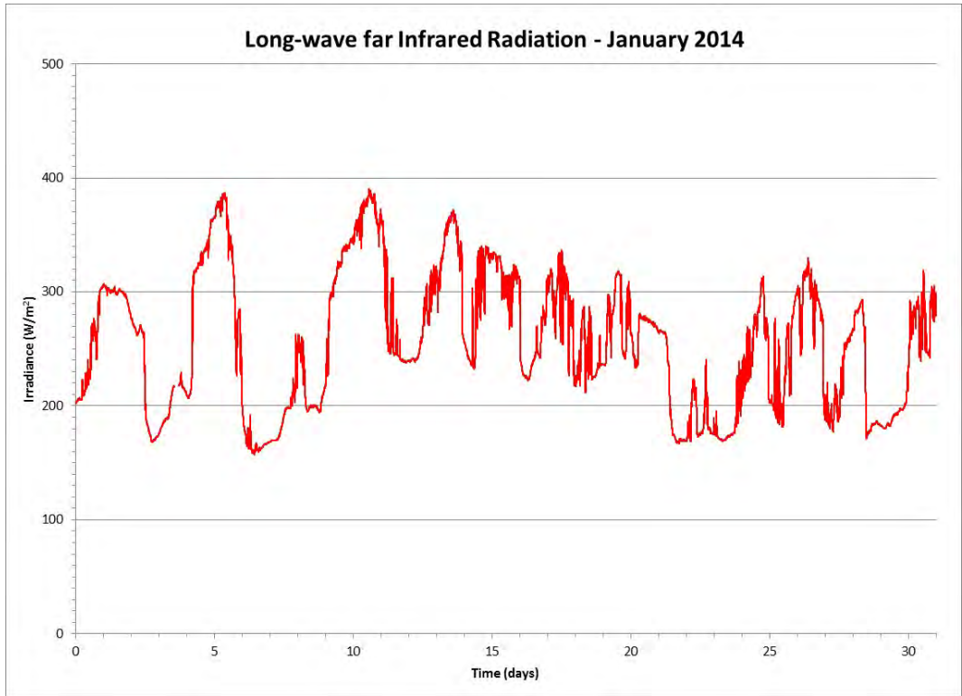
Figure 149 Long-wave Far Infrared Radiation for the Month of January 2014
