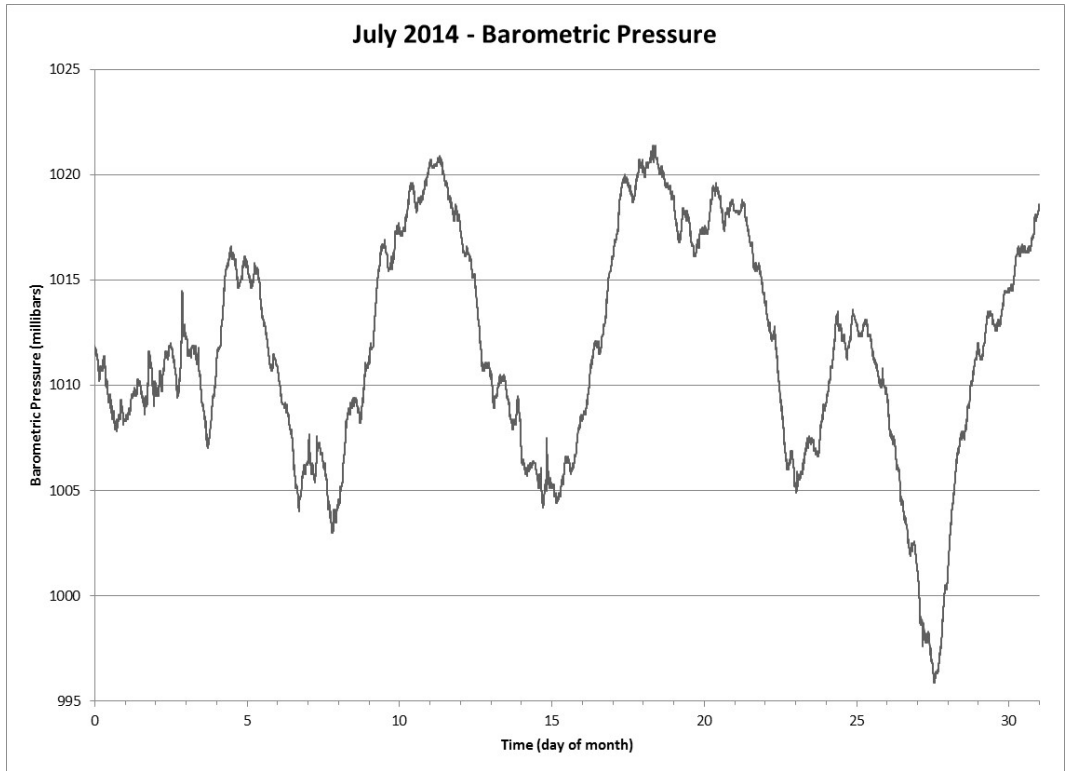
Figure 23 Barometric Pressure for the Month of July 2014
