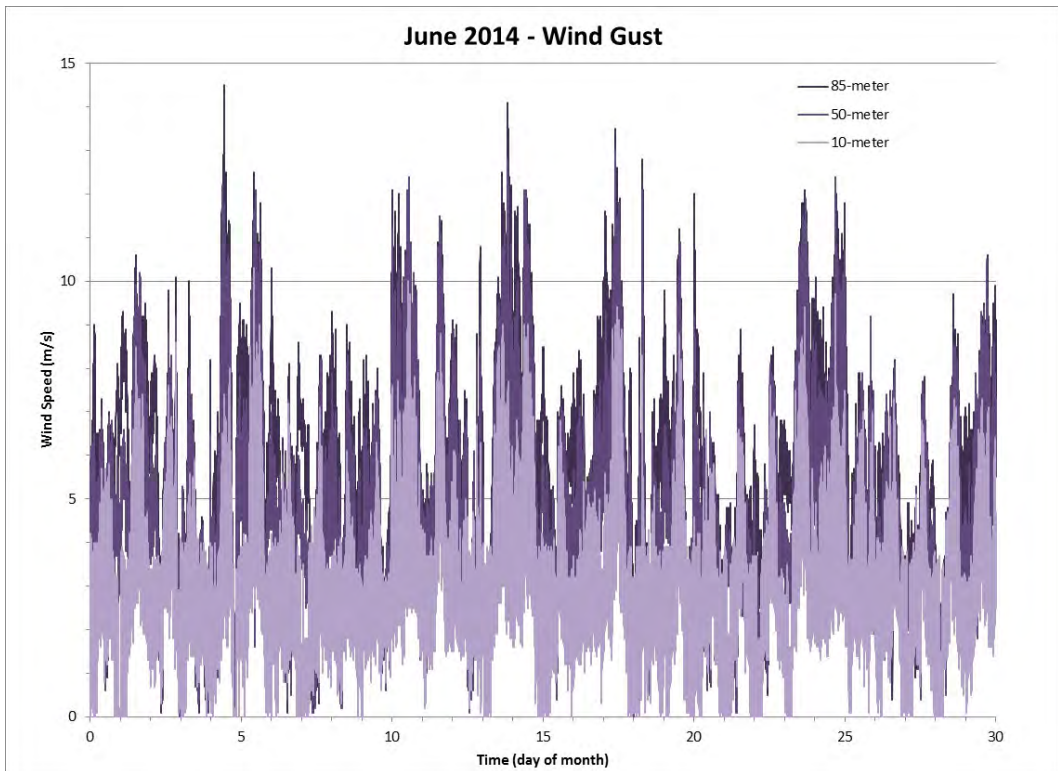
Figure 97 Wind Gust data for the Month of June 2014
