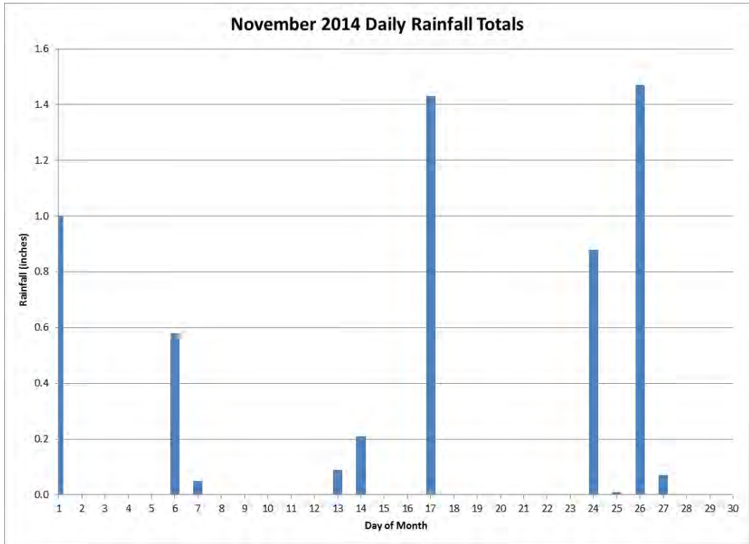
Figure 55 Daily Rainfall for the Month of November 2014
