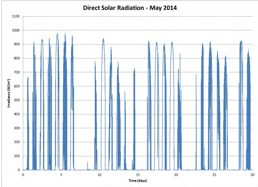
Figure 141 Direct Solar Radiation for the Month May 2014
