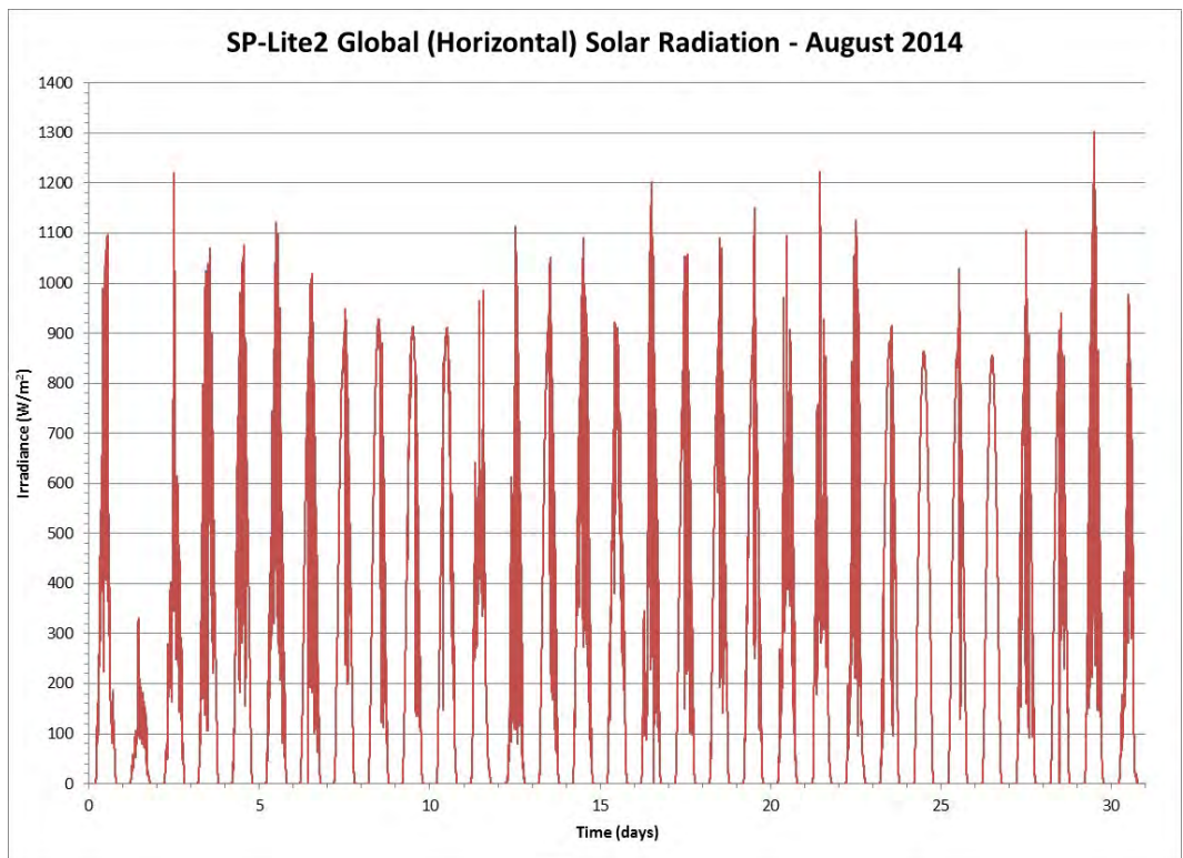
Figure 168 Global Solar Radiation from an SP-Lite2 Pyranometer for the Month of August 2014
