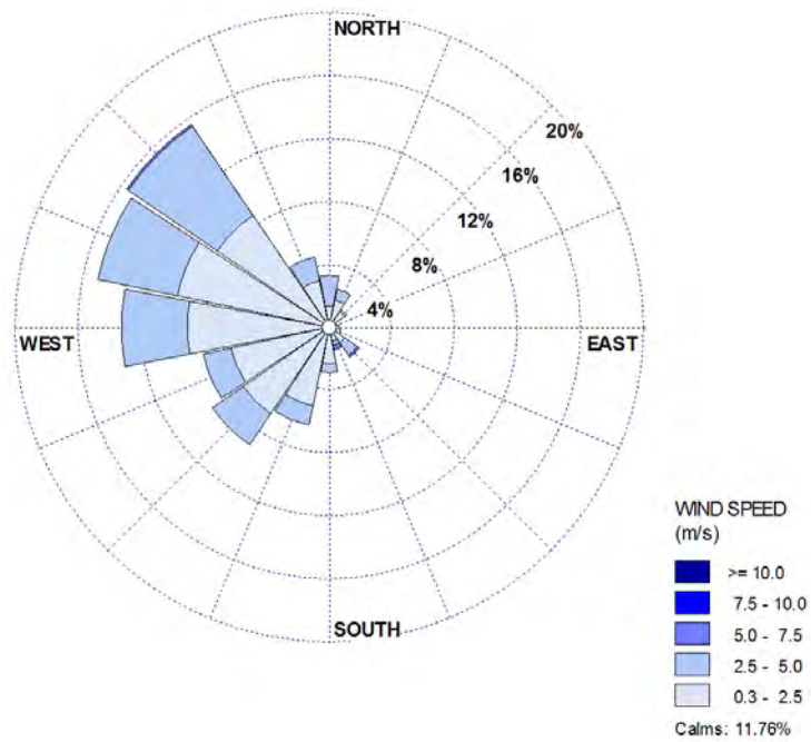
Figure 82 One-hour Wind Roses for the Month of November 2014 from the 85m level
