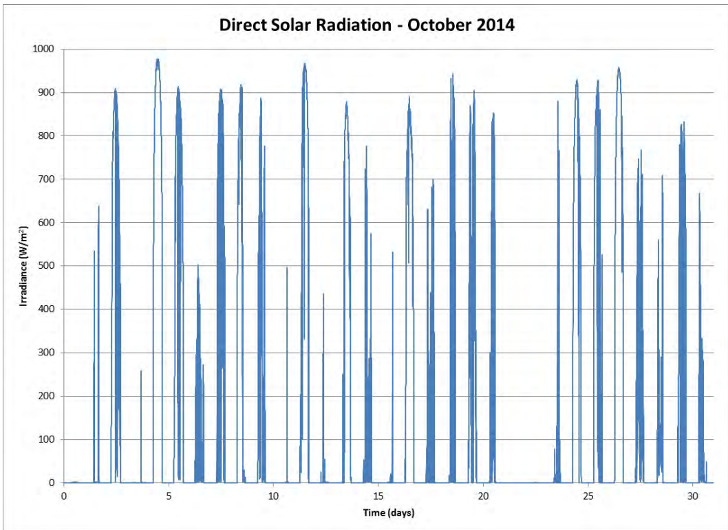
Figure 146 Direct Solar Radiation for the Month October 2014
