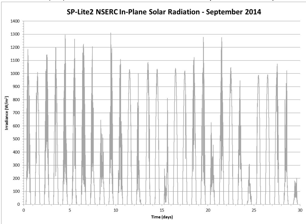
Figure 183 Tilted ( 23^\circ ) Global Solar Radiation from an SP-Lite2 Pyranometer for September 2014
