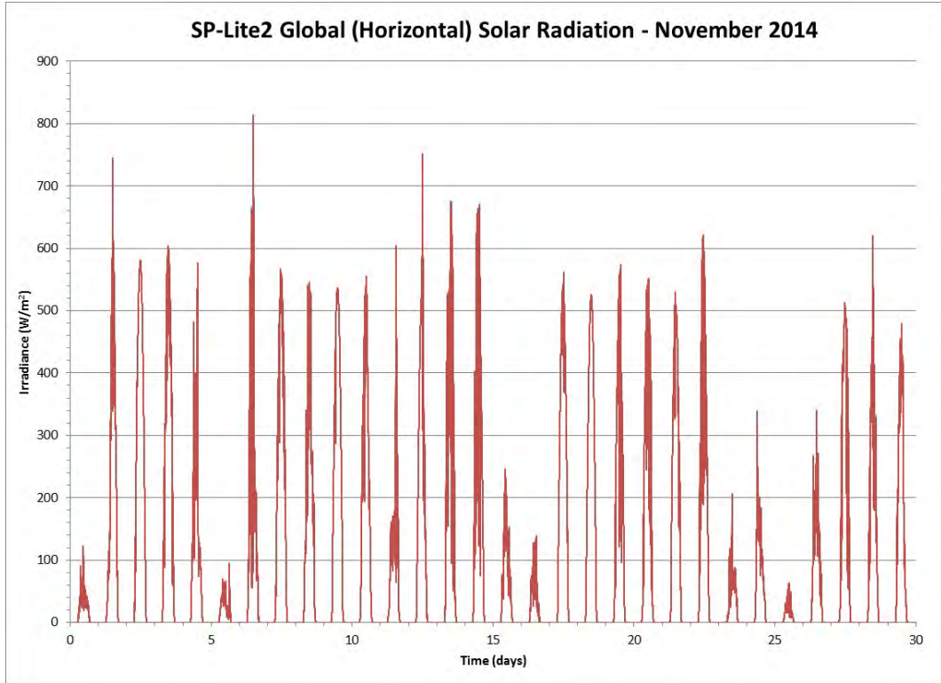
Figure 171 Global Solar Radiation from an SP-Lite2 Pyranometer for the Month of November 2014
