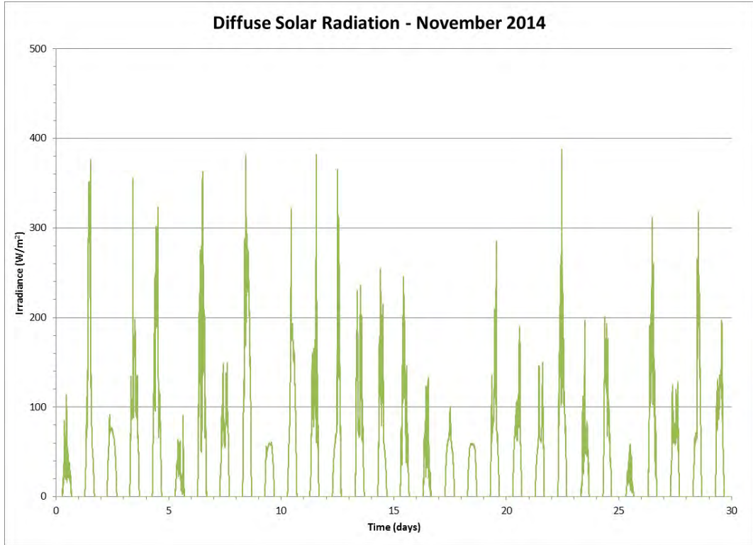
Figure 135 Diffuse Solar Radiation for the Month of November 2014
