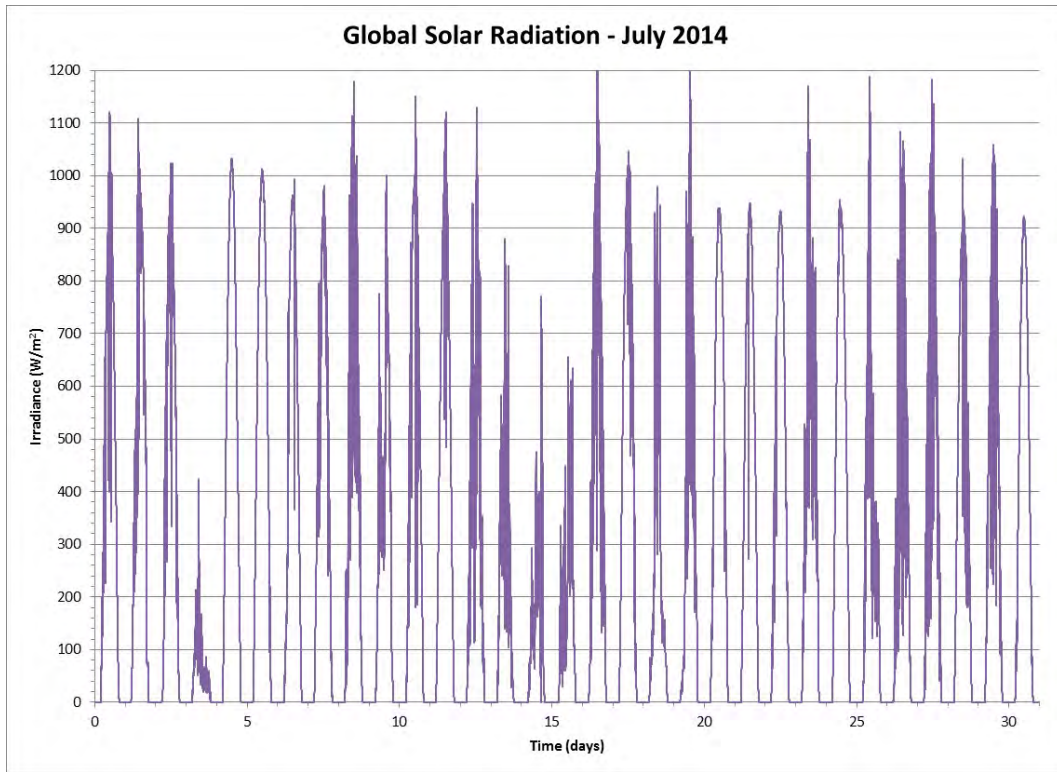
Figure 119 Global Solar Radiation for the Month of July 2014
