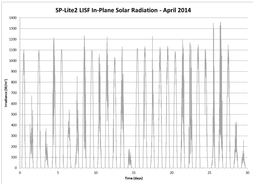
Figure 176 Tilted (27°) Global Solar Radiation from an SP-Lite2 Pyranometer for April 2014
