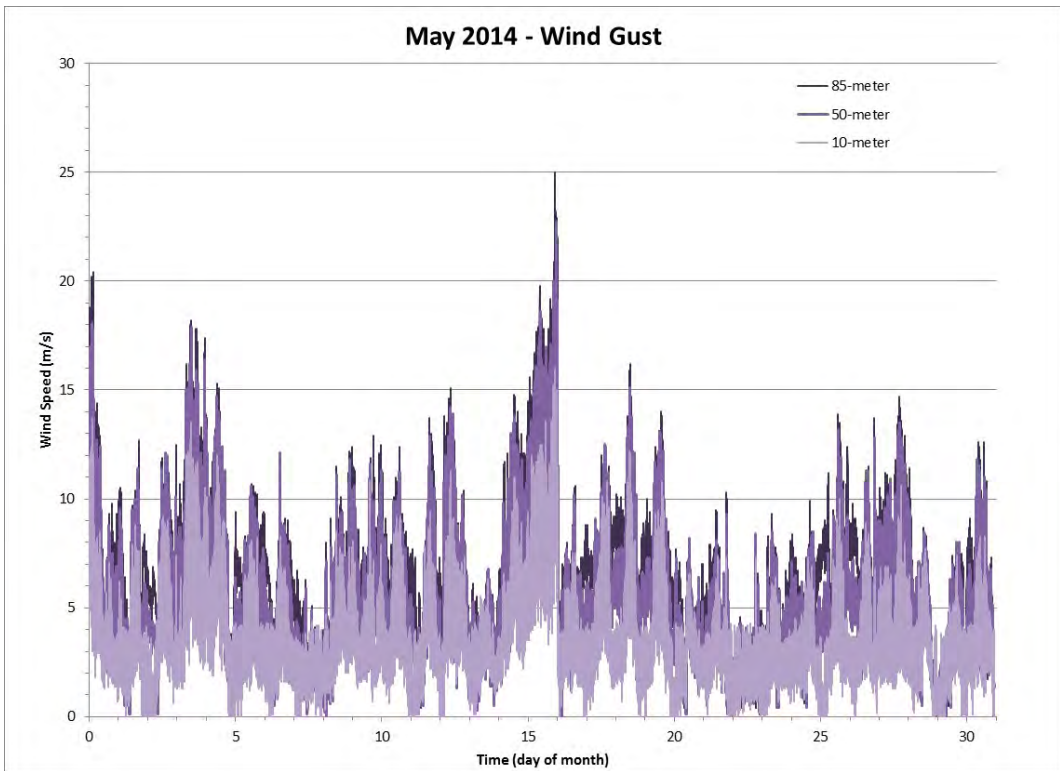
Figure 95 Wind Gust data for the Month of May 2014
