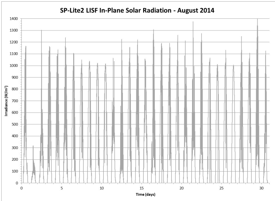
Figure 180 Tilted ( 27^\circ ) Global Solar Radiation from an SP-Lite2 Pyranometer for August 2014
