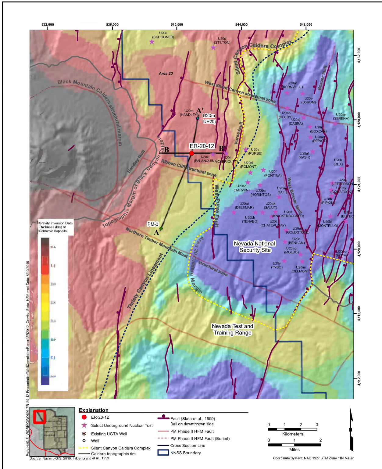
Figure 5-3 Gravity Inversion Map
