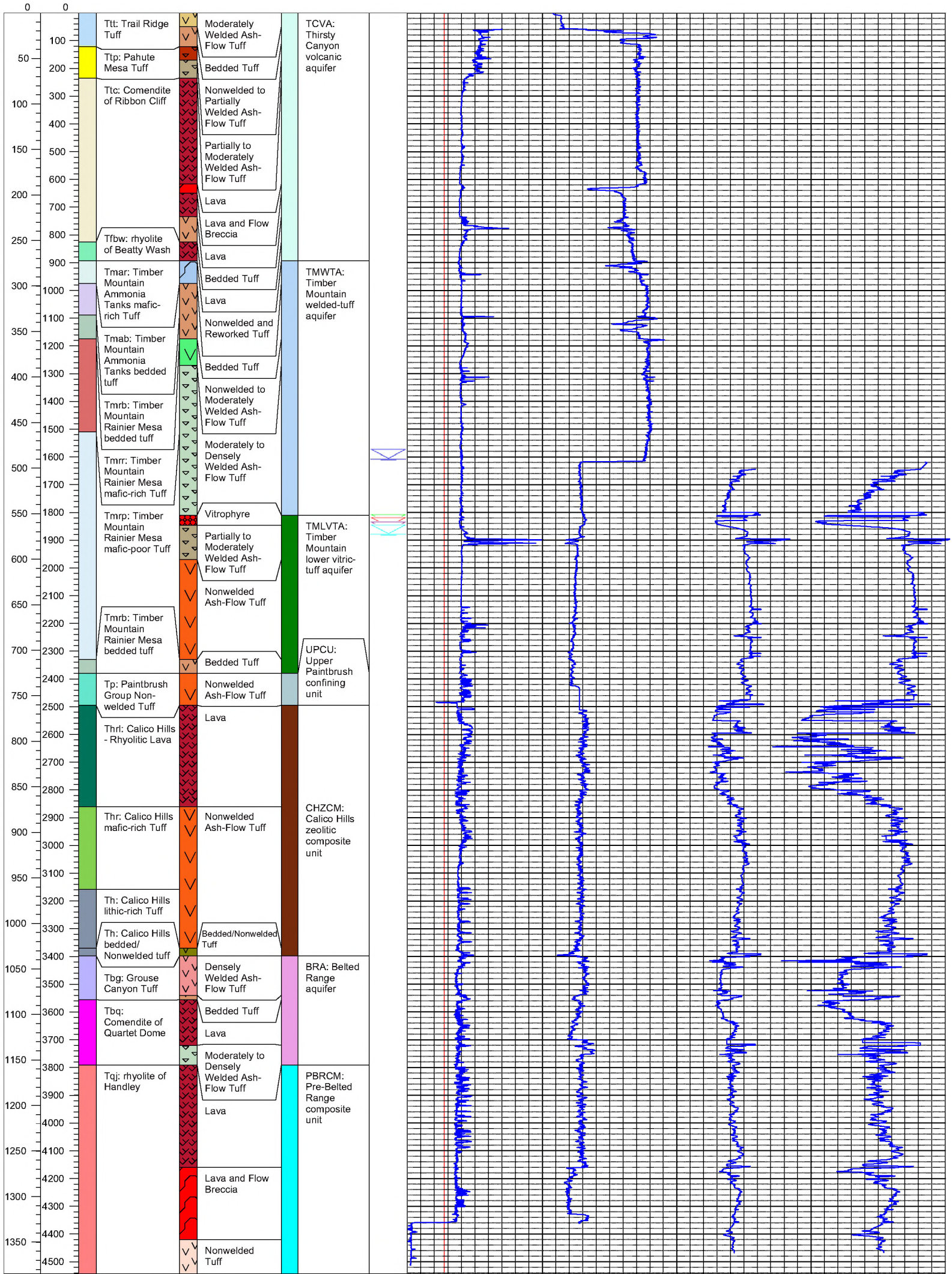
Figure E-3 Geophysical Log Traces of Caliper, Gamma Ray, Delta T, and Sonic Porosity
