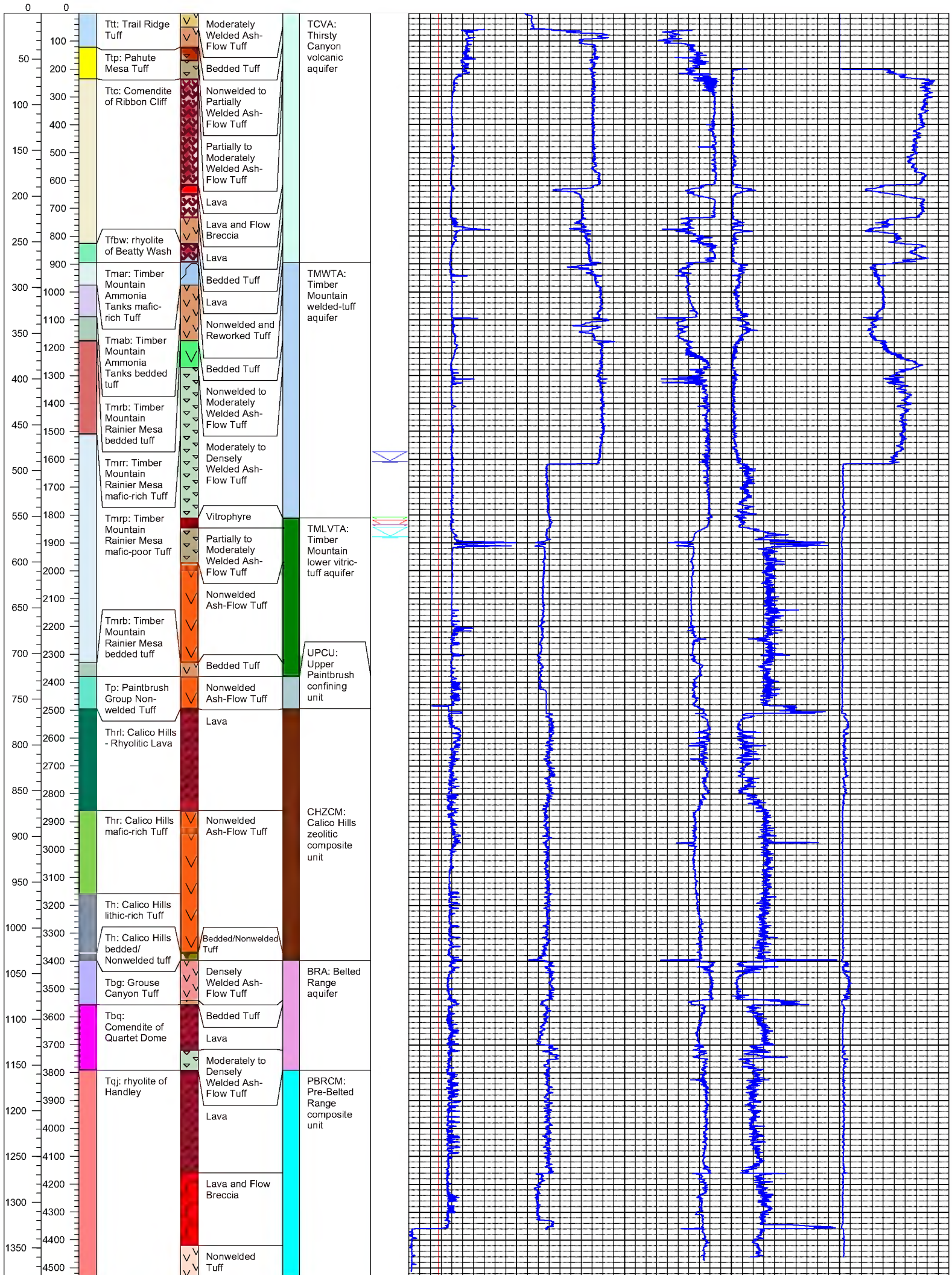
Figure E-2 Geophysical Log Traces of Caliper, Gamma Ray, Bulk Density, and Neutron Porosity
