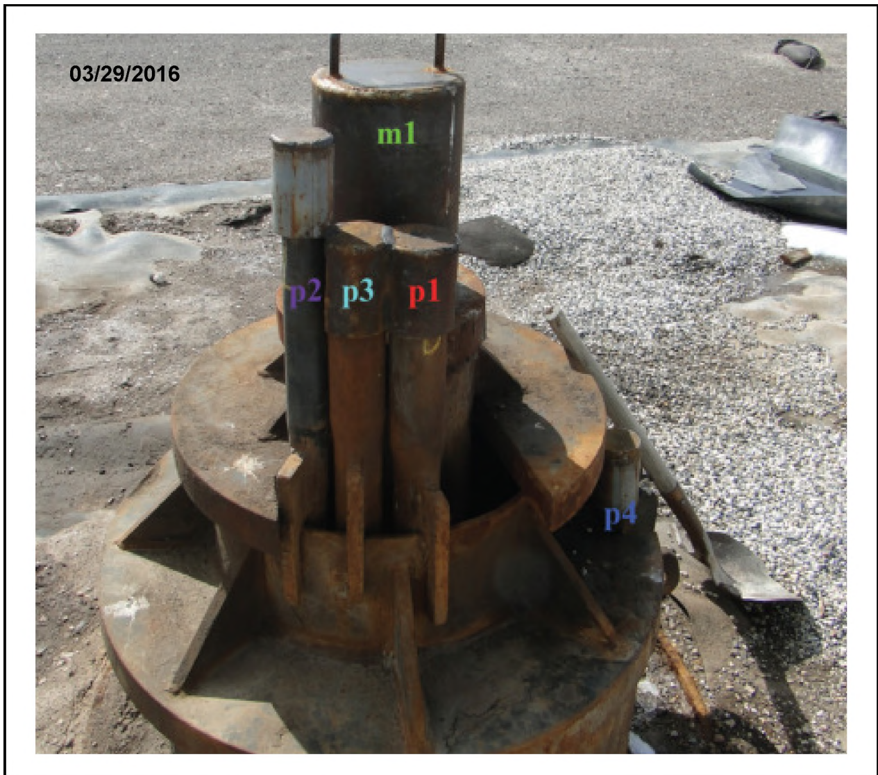
Figure 8-3 Photograph of Well ER-20-12 Wellhead
