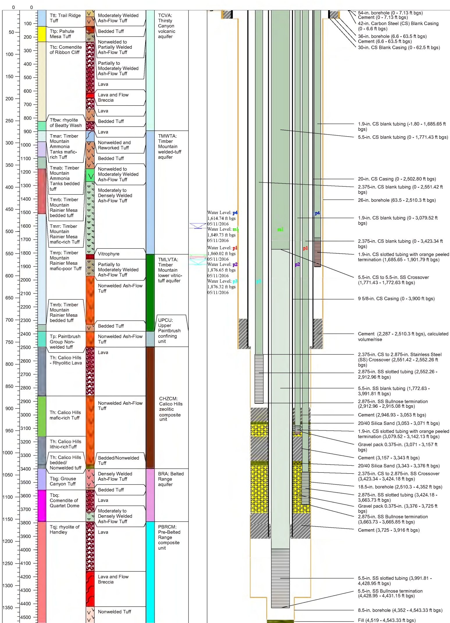
Figure 8-1 Well Completion Diagram for Well ER-20-12
