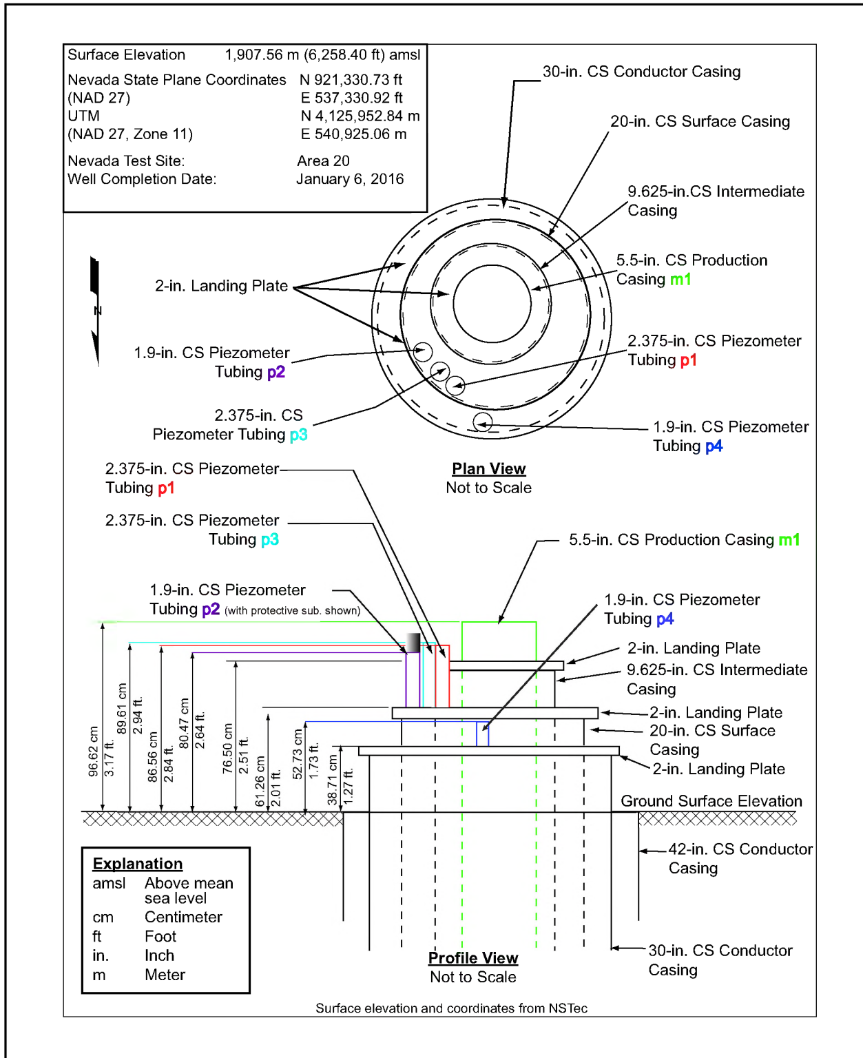
Figure 8-2 Wellhead Diagram for ER-20-12
