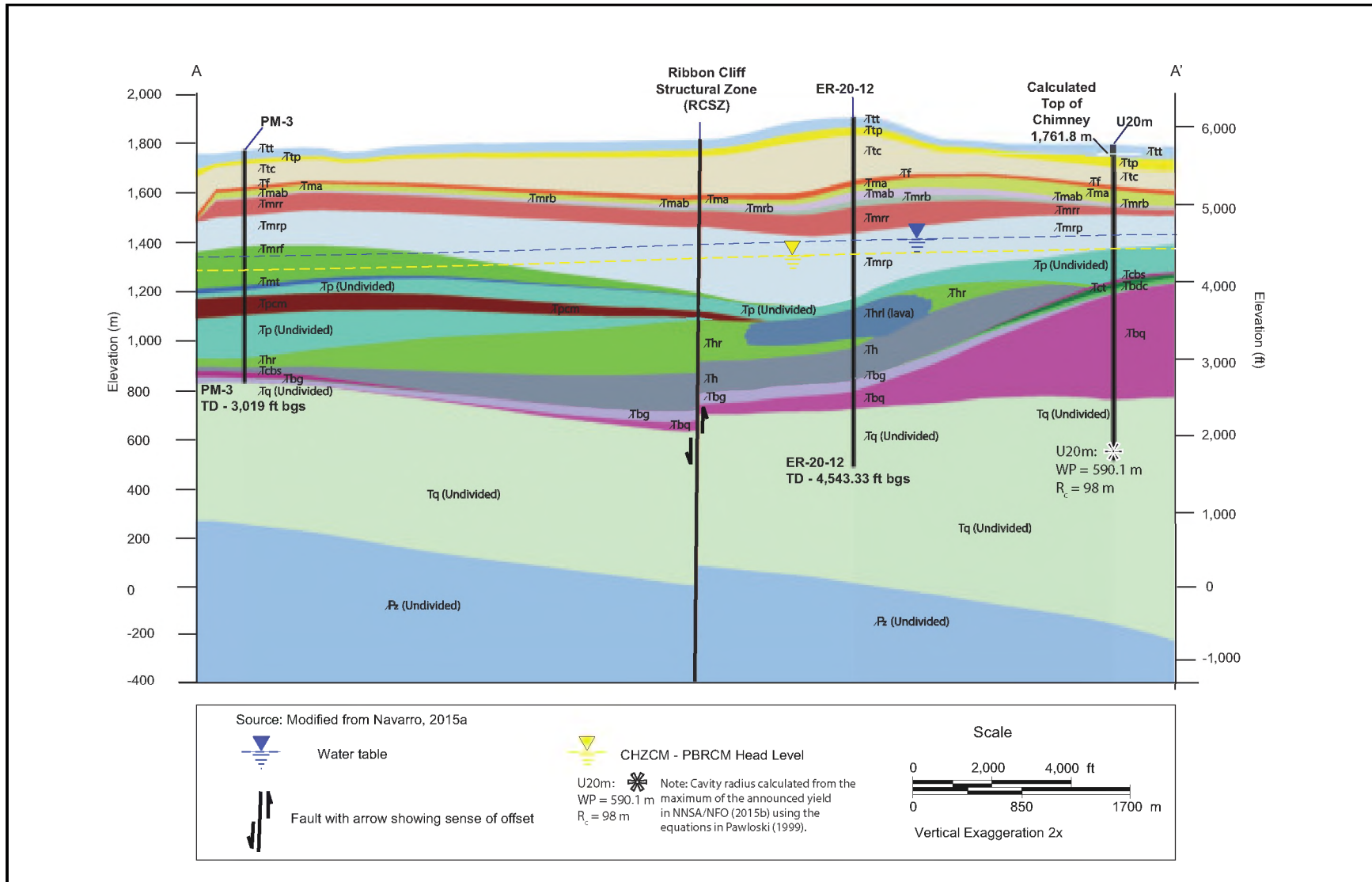
Figure 5-5 Southwest–Northeast Stratigraphic Cross Section A–A’ through Well ER-20-12
