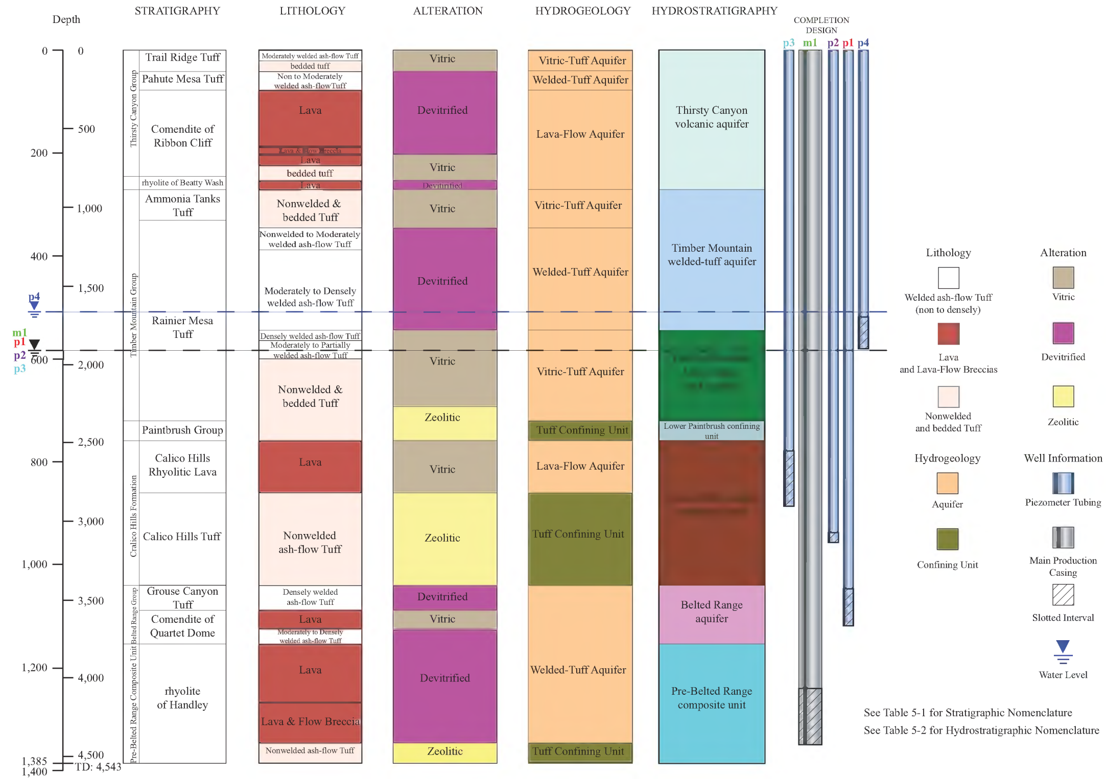
Figure 5-4 Graphical Presentation Showing Geology and Hydrogeology for Well ER-20-12
