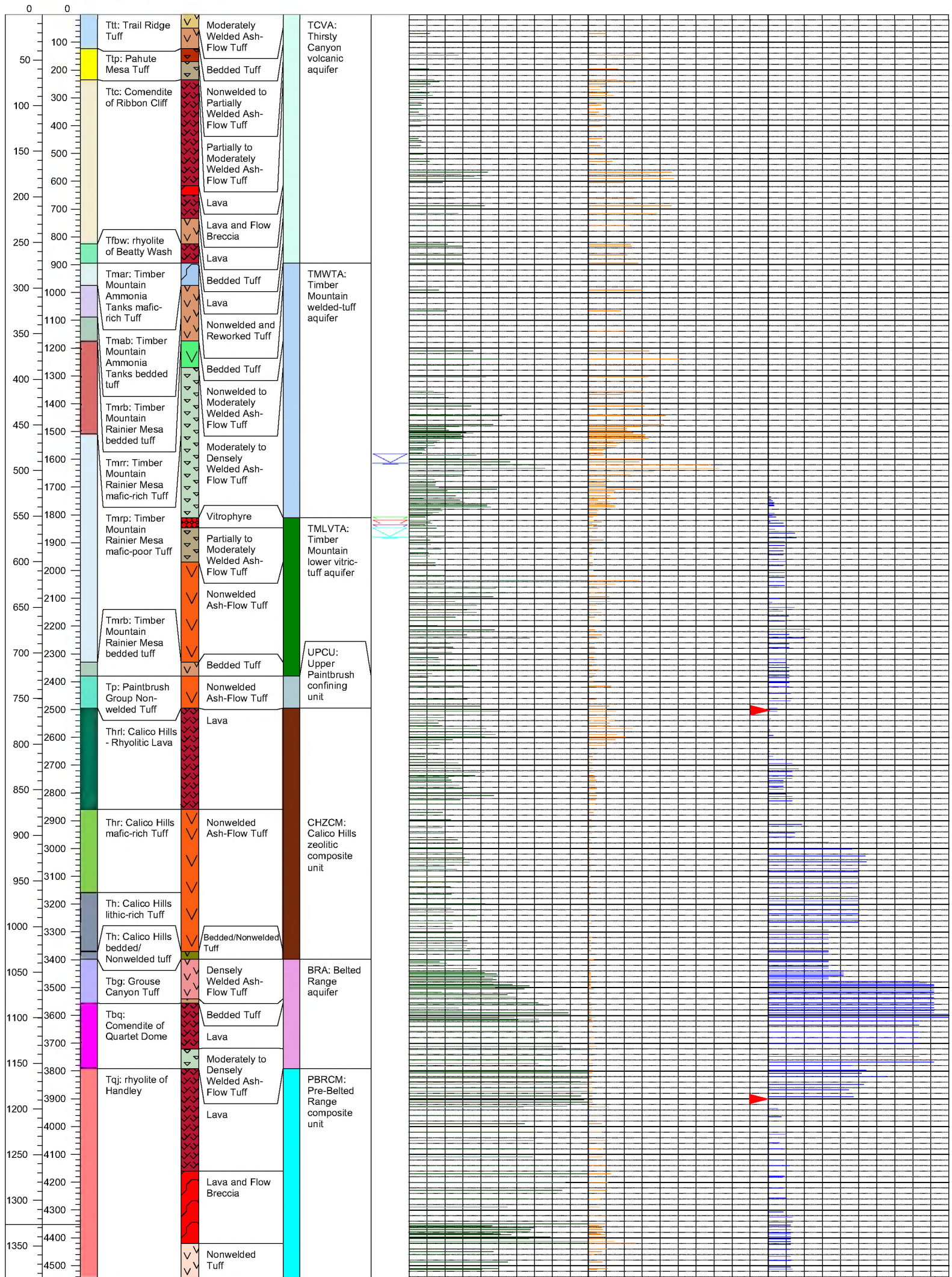
Figure F-1 Bromide and Water Production at ER-20-12
