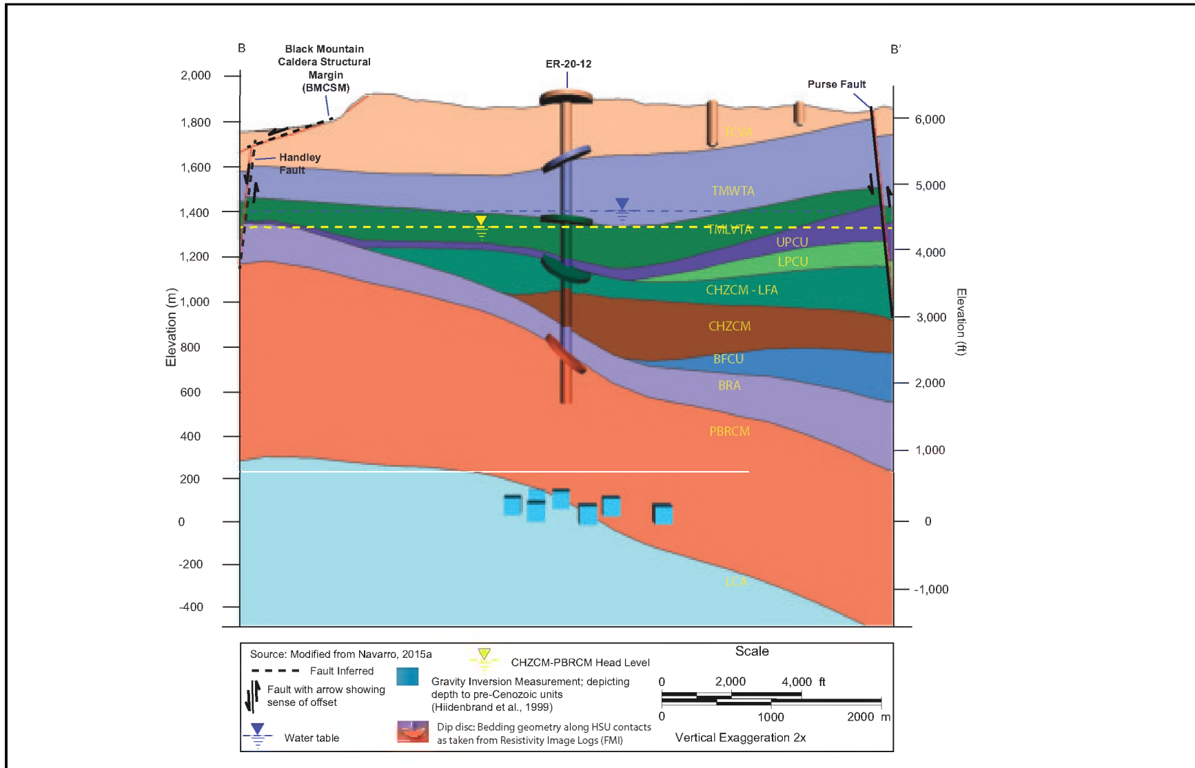
Figure 5-8 East-West Hydrostratigraphic Geologic Cross Section B-B' through Well ER-20-12
