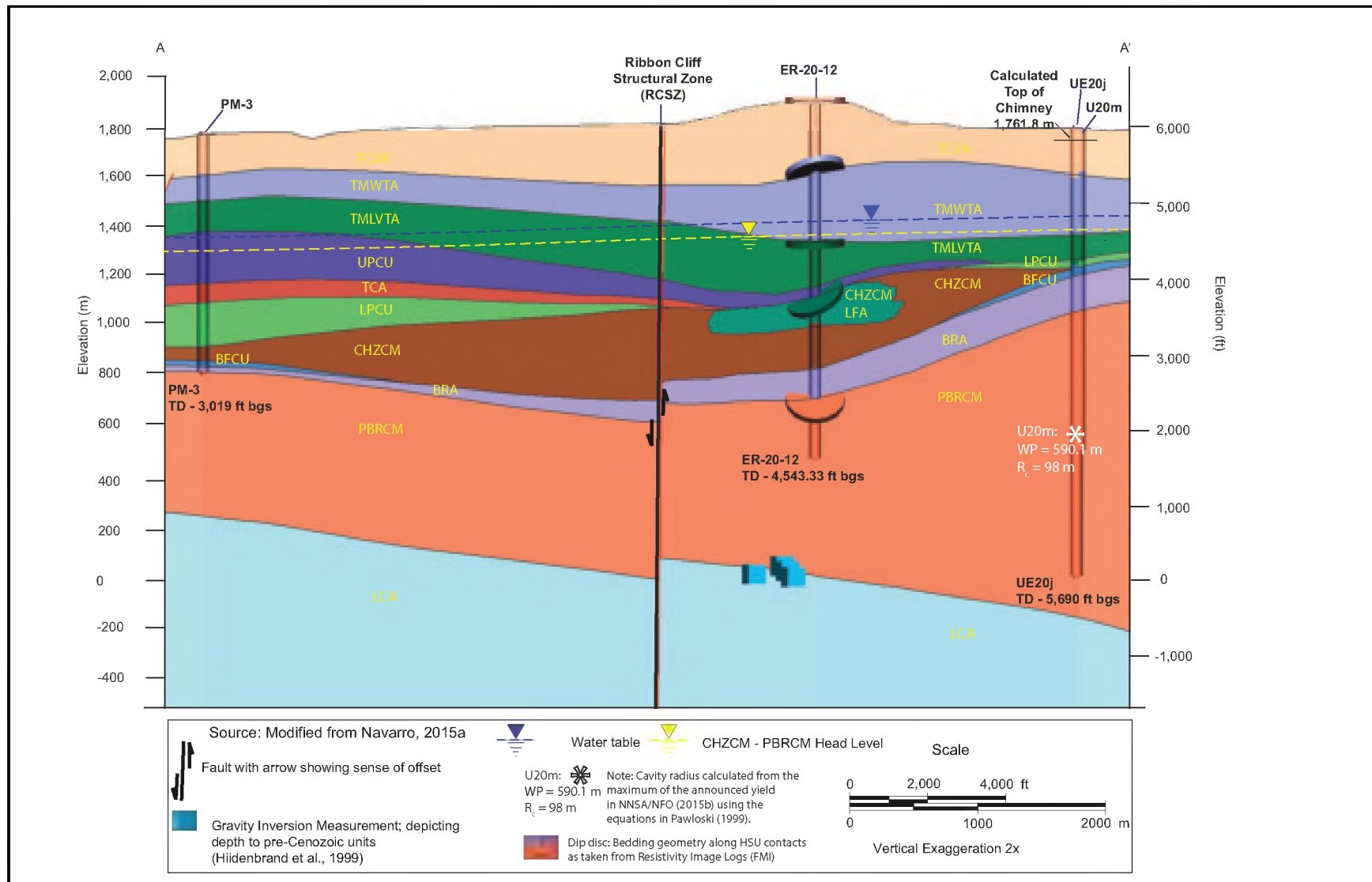
Figure 5-7 Southwest-Northeast Hydrostratigraphic Cross Section A-A' through Well ER-20-12
