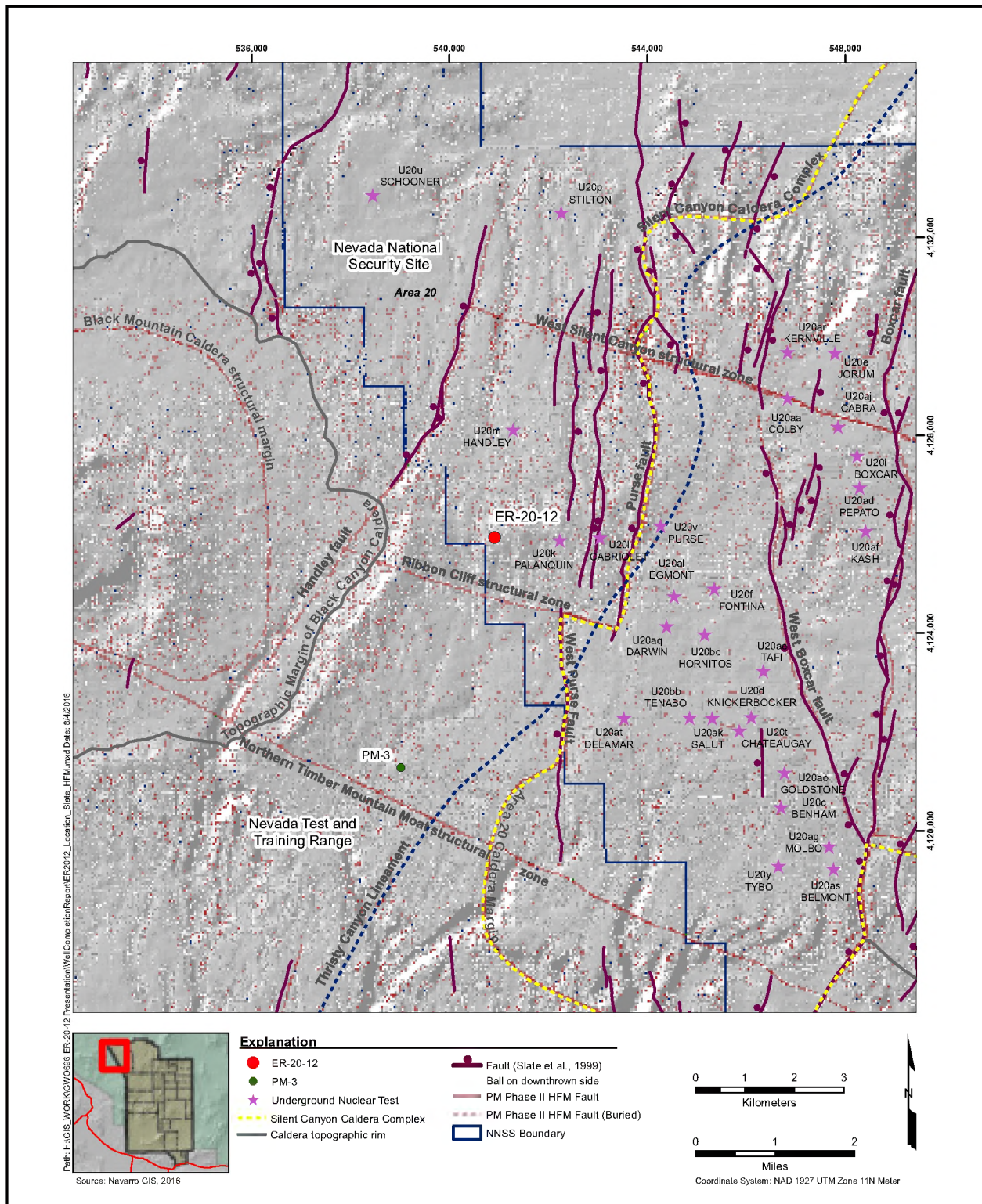
Figure 5-2 Geologic Structure Map of the Well ER-20-12 Area
