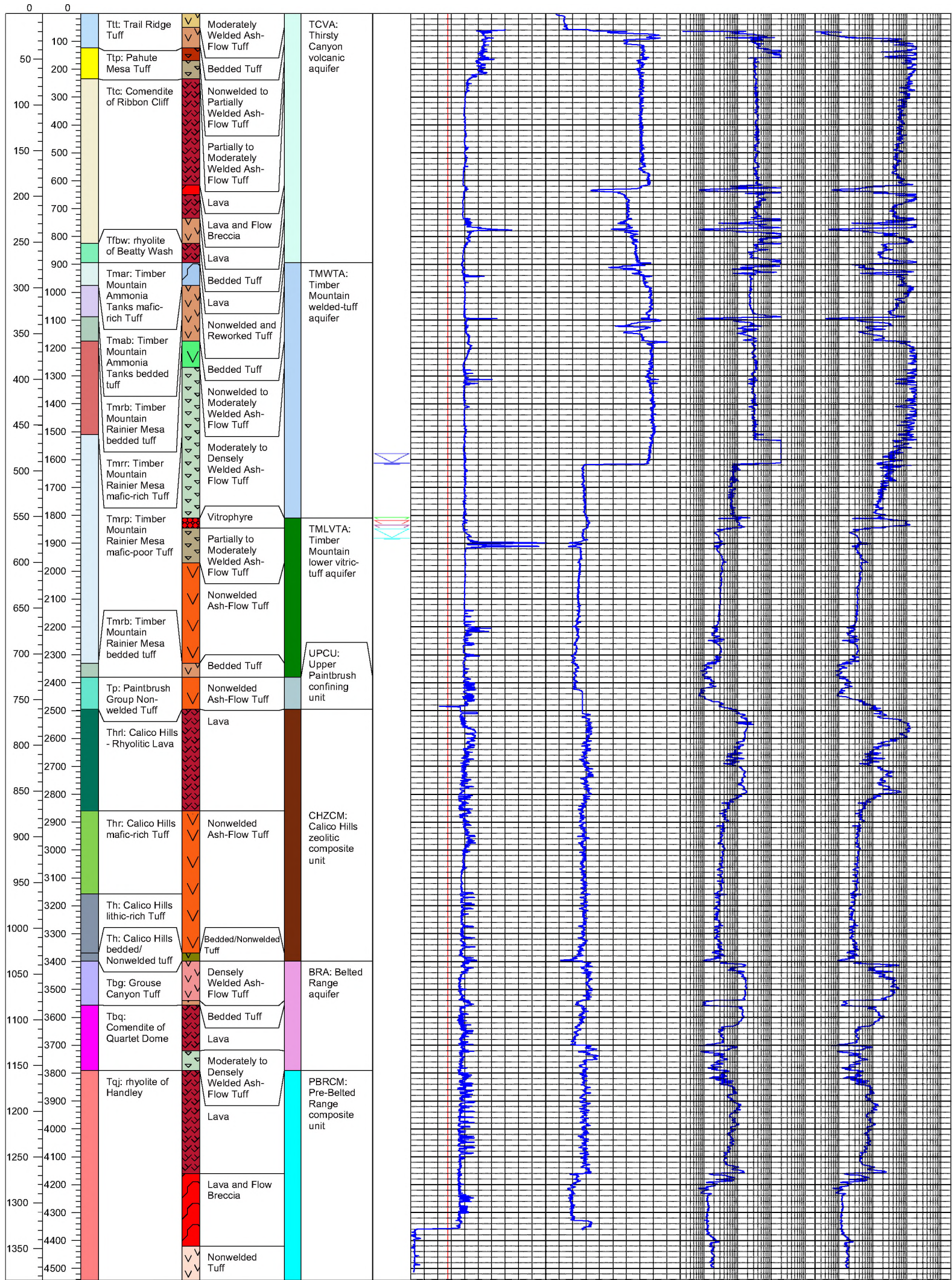
Figure E-5 Geophysical Log Traces of Caliper, Gamma Ray, and Shallow and Deep Resistivity
