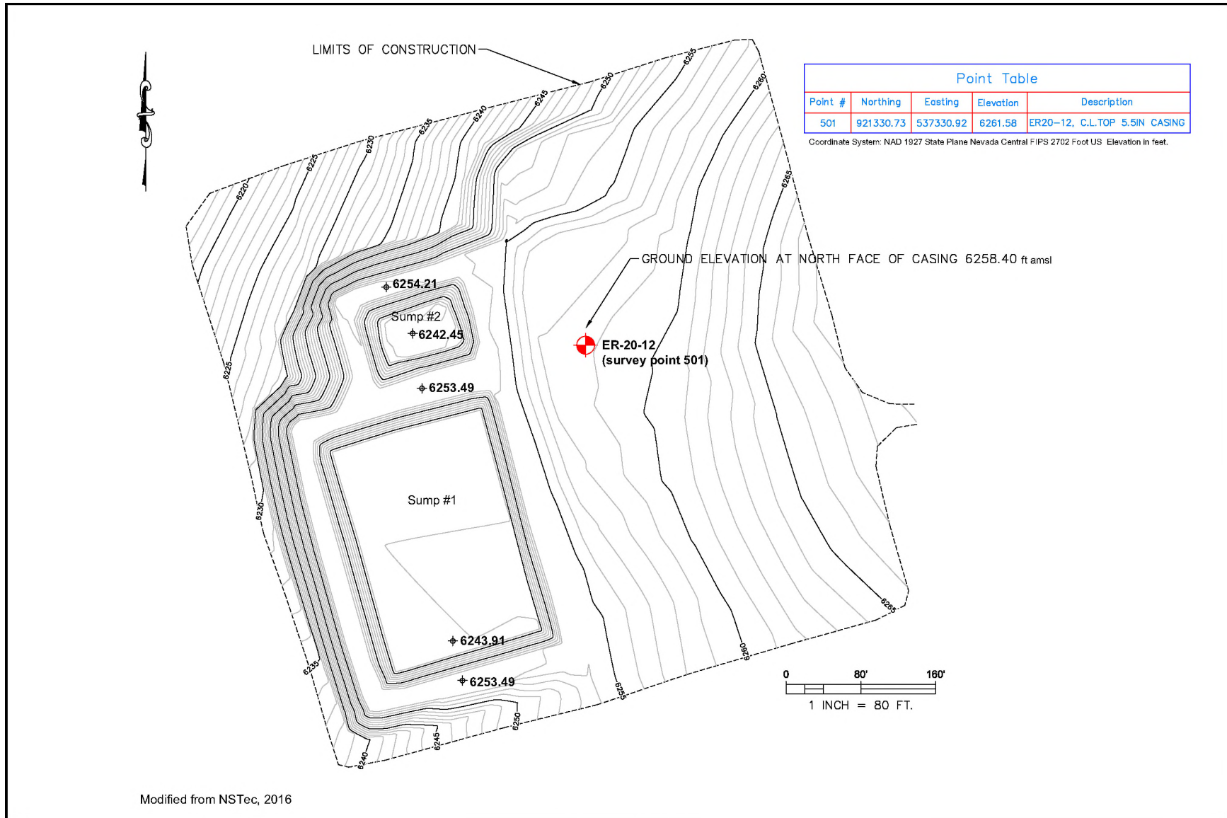
Figure 2-1 Well ER-20-12 As-Built Site Diagram
