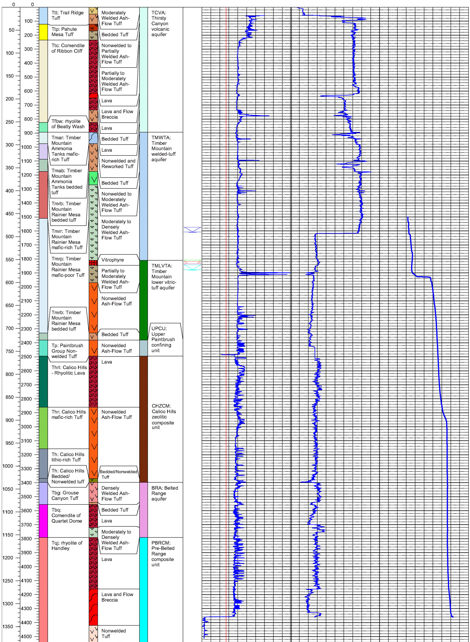
Figure E-1 Geophysical Log Traces of Caliper, Gamma Ray, and Temperature
