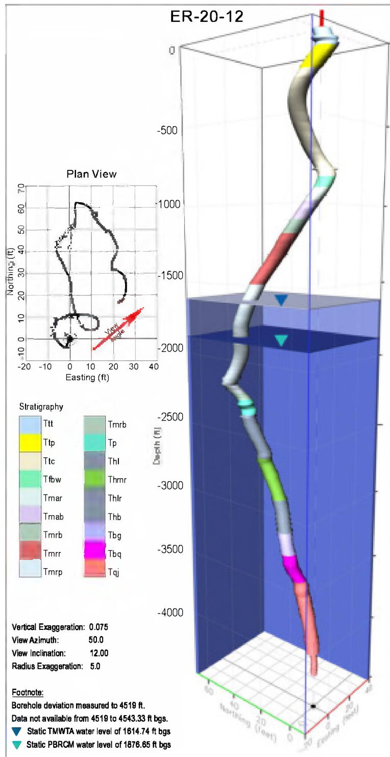
Figure 2-3 Well ER-20-12 Directional Survey Showing Caliper Profile and Stratigraphy
