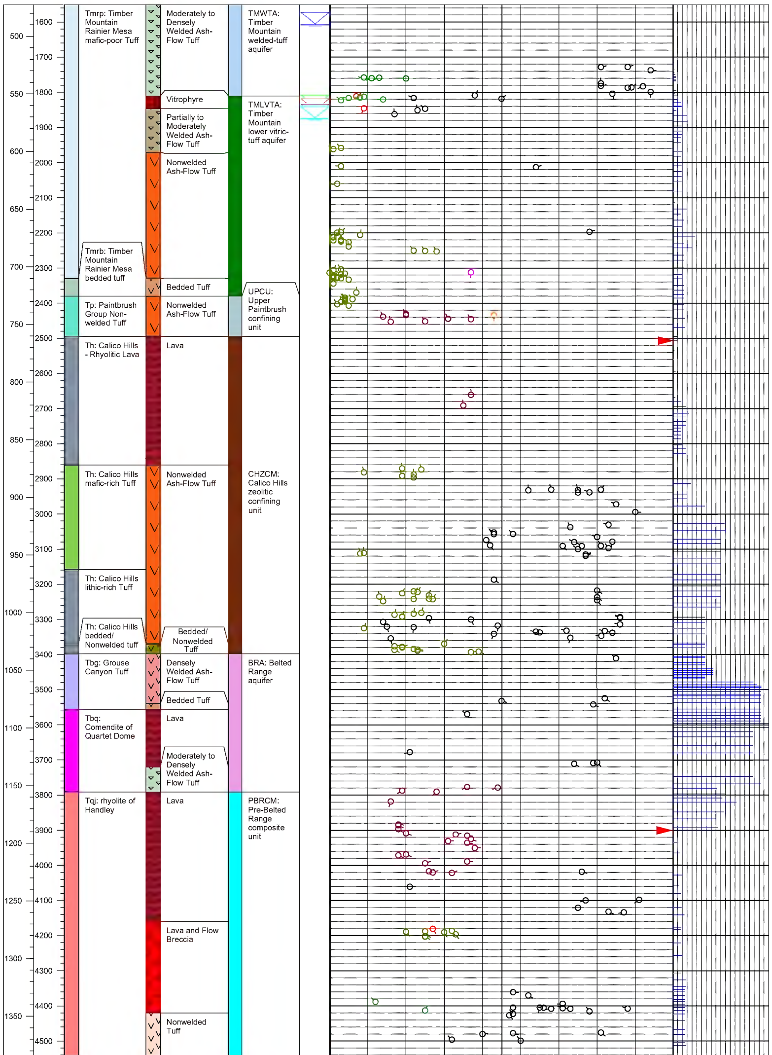
Figure 4-1 Tadpole Diagram for Well ER-20-12
