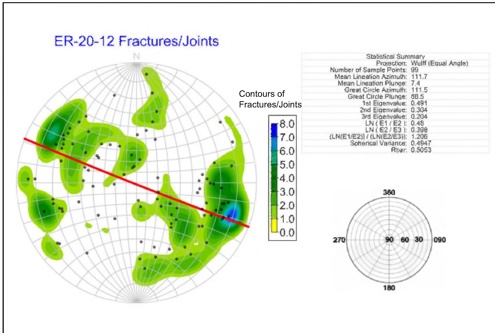
Figure G-1 Stereonet of Fractures and Joints in ER-20-12
