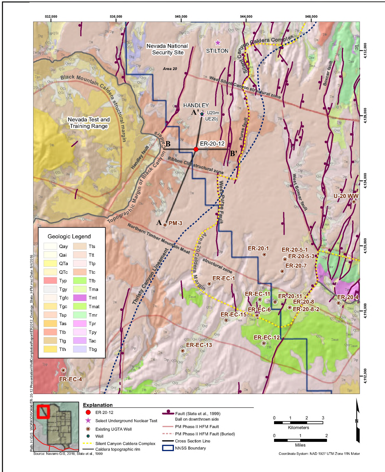
Figure 5-1 Surface Geologic Map of the Well ER-20-12 Area
