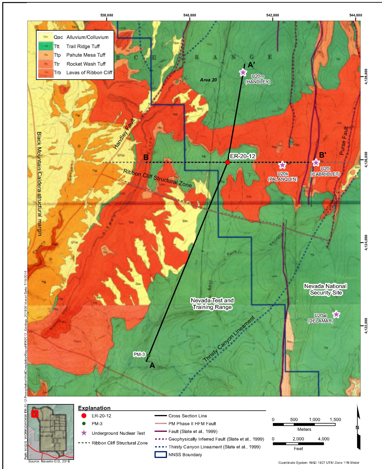
Figure 1-3 Surface Geologic Map of the Well ER-20-12 Area Source: Modified from Christensen, 1966; and modified from Christiansen and Noble, 1968
