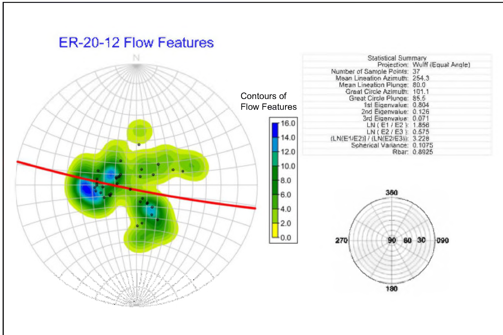
Figure G-5 Stereonet of Flow Features in ER-20-12
