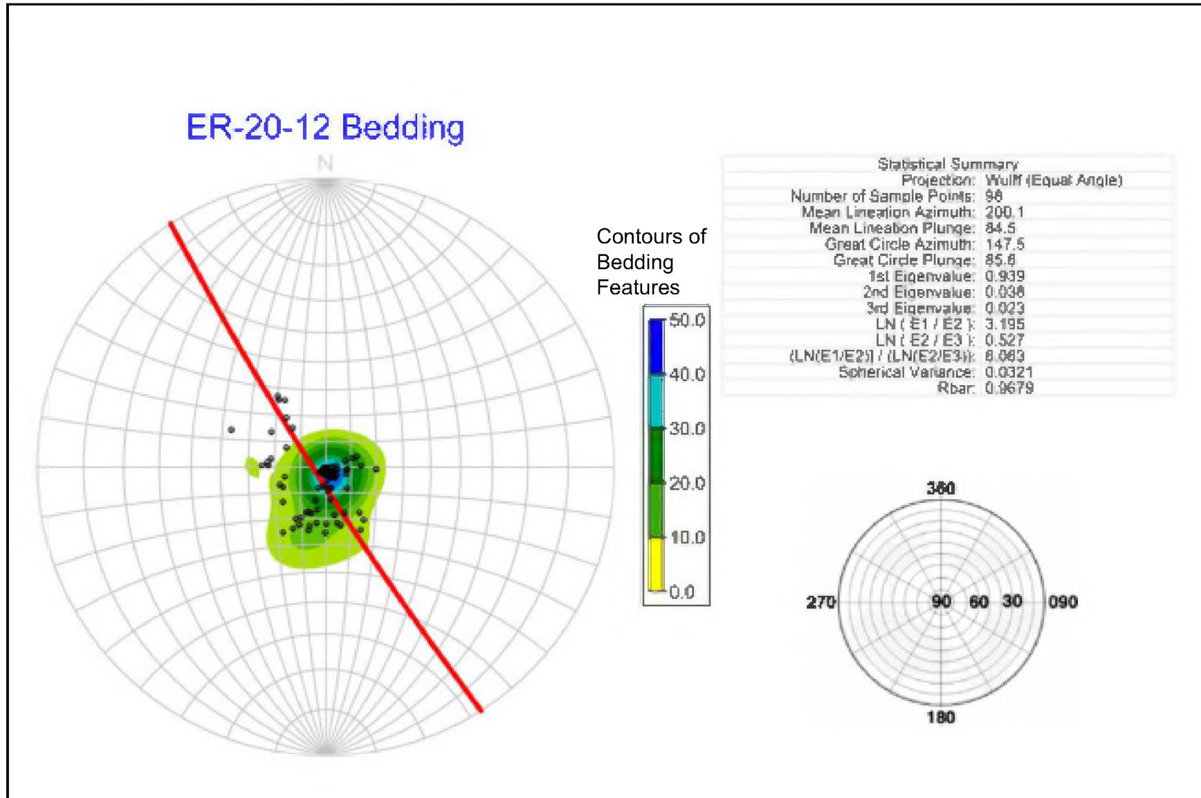
Figure G-3 Stereonet of Bedding Features in ER-20-12
