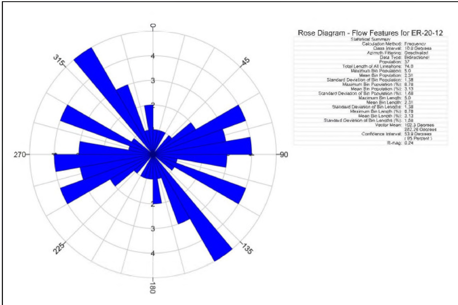
Figure G-6 Rose Diagram of Flow Features in ER-20-12
