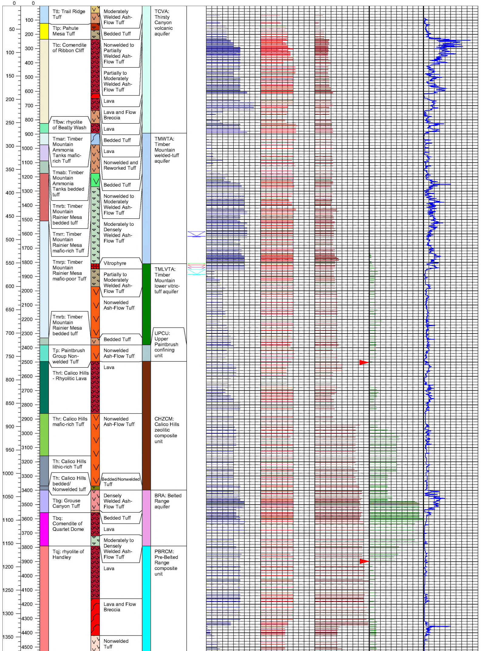
Figure A-1 Drilling Parameters Log for Well ER-20-12
