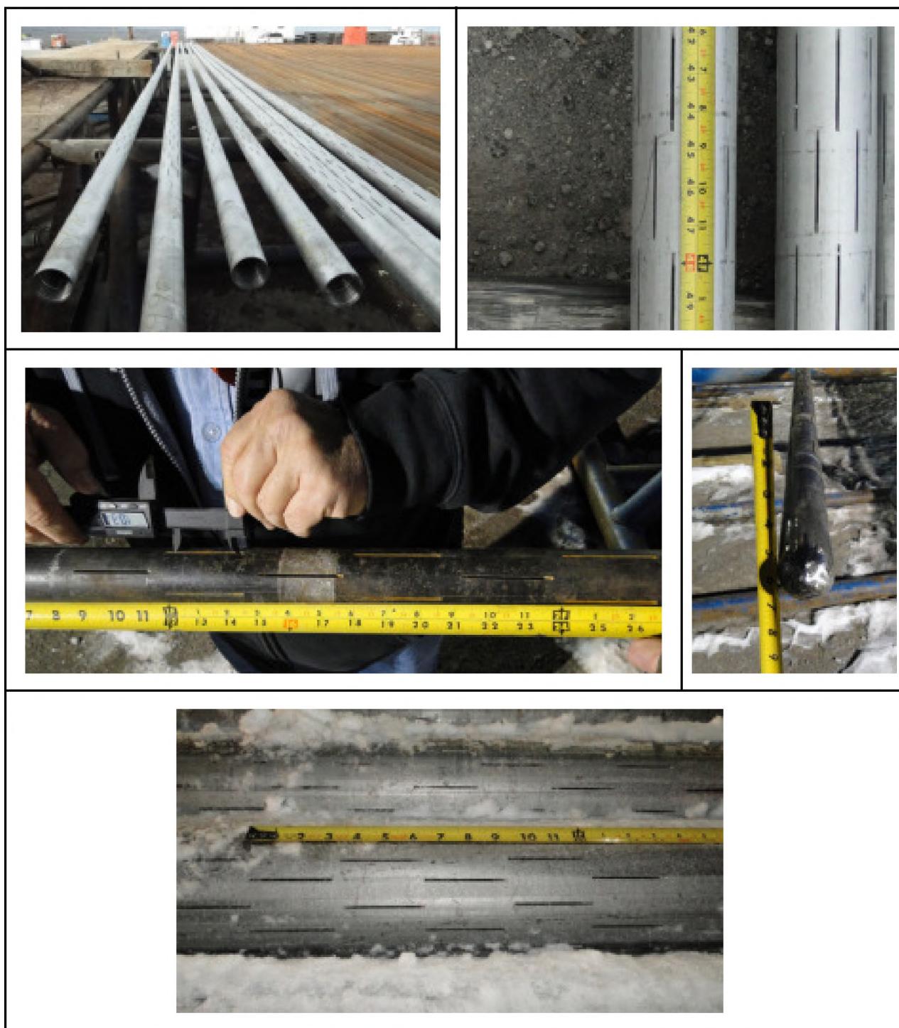
Figure 8-4 Slotted Tubing for ER-20-12
