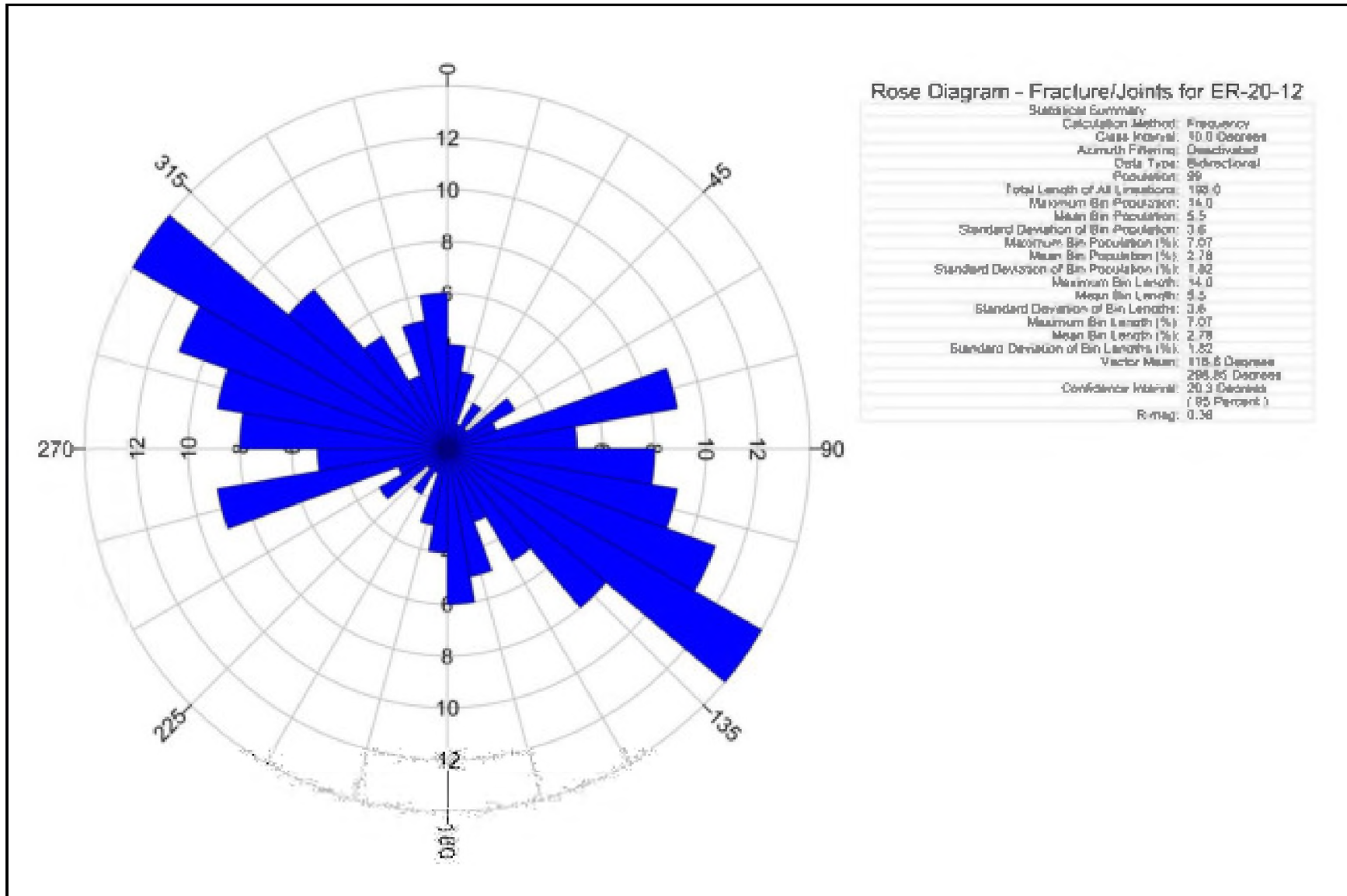
Figure G-2 Rose Diagram of Fractures/Joints in ER-20-12
