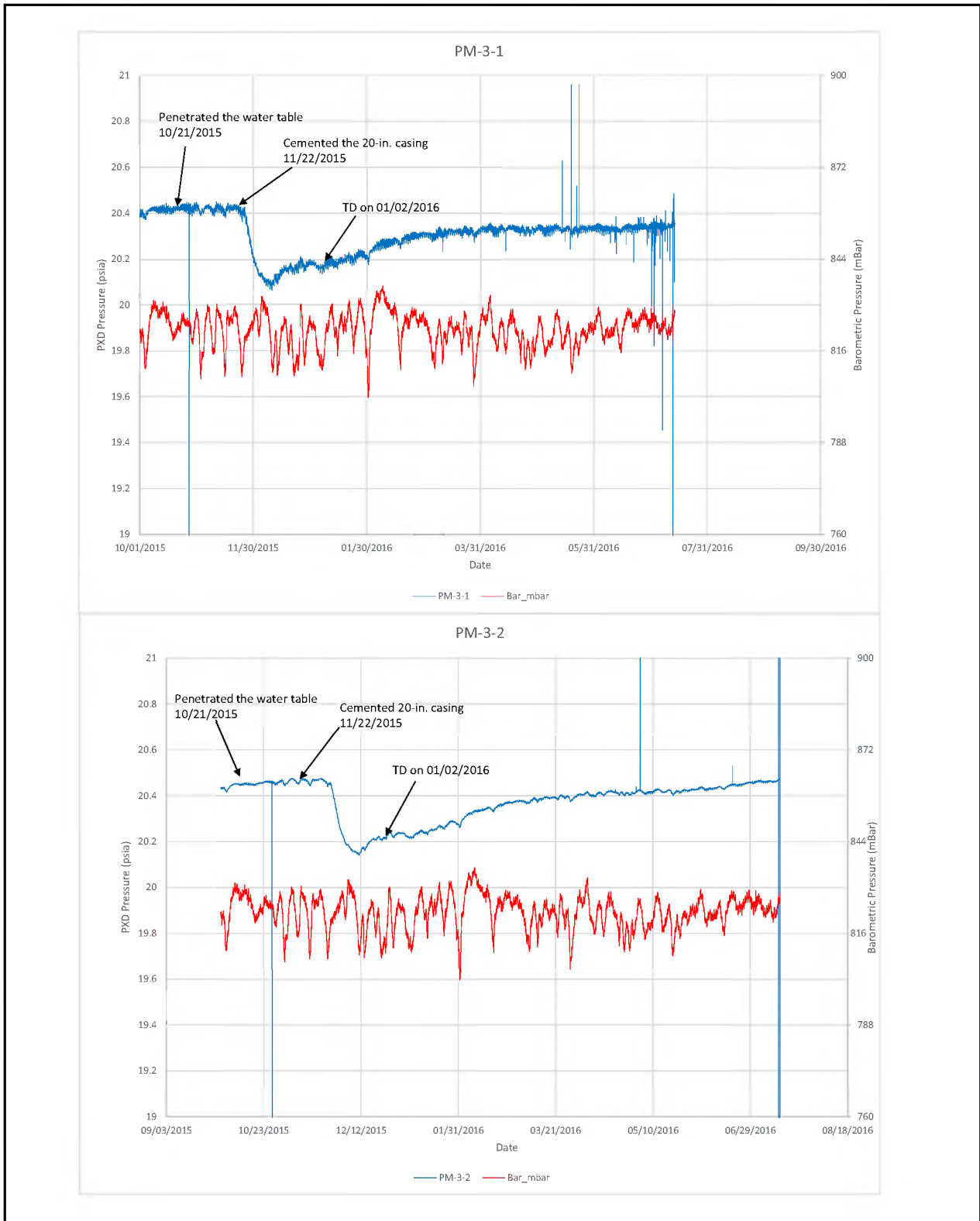
Figure 6-3 Well PM-3 Well Response during Well ER-20-12 Drilling
