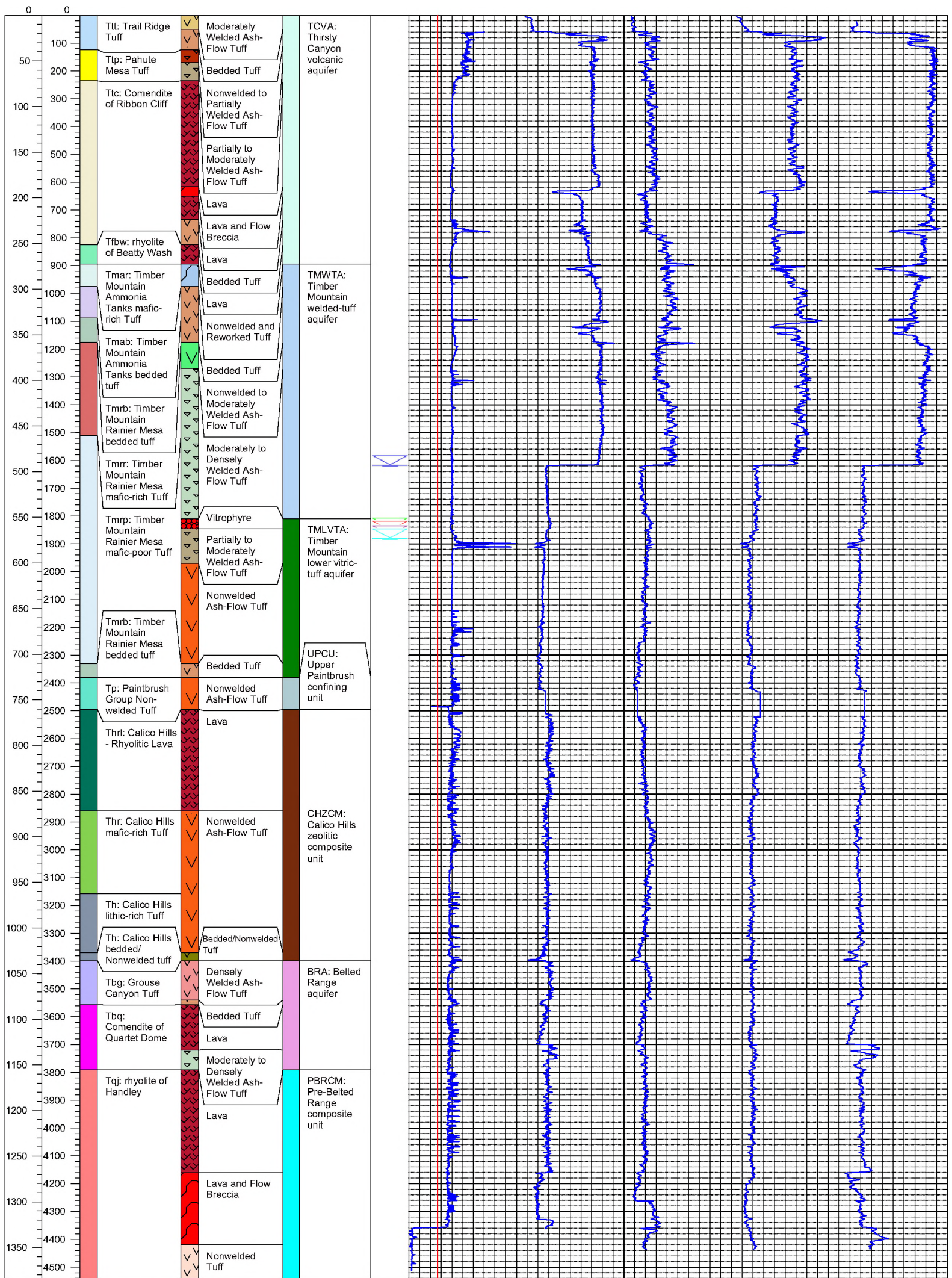
Figure E-4 Geophysical Log Traces of Caliper, Gamma Ray, and Digital Spectralog
