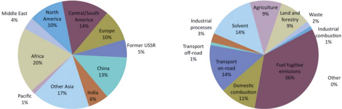
Figure 3-4. Distribution of global NMVOC emissions in 2005 by world region (left) and by major source type (right), from Emissions Data Base for Global Atmosphere Research (EDGAR) v4.1
