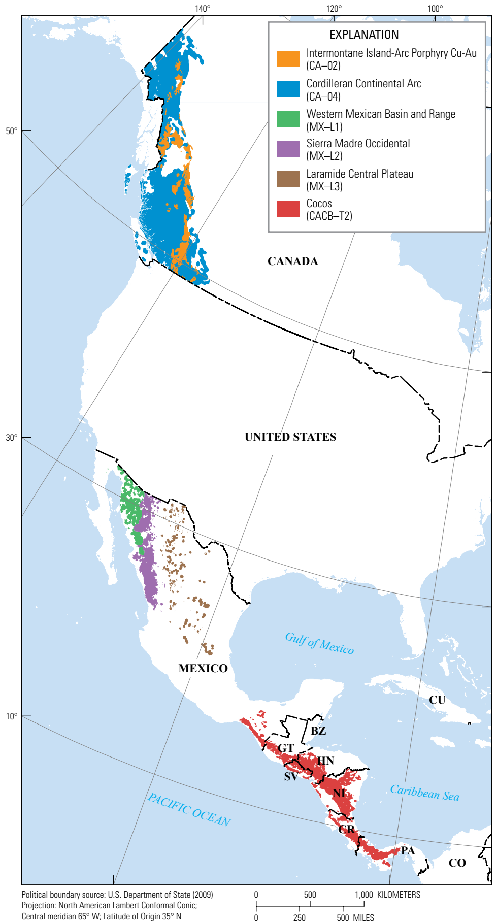
Figure 5. Selected permissive tracts for porphyry copper deposits in North America. Tract identifiers, names, and descriptions are given in table 9. GT, Guatemala; BZ, Belize; SV, El Salvador; HN, Honduras; NI, Nicaragua; CR, Costa Rica; PA, Panama; CO, Columbia; CU, Cuba.
