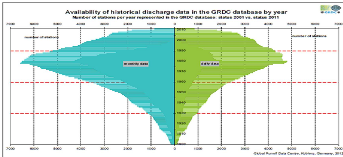
Figure 5: Availability of historical discharge data at GRDC.
