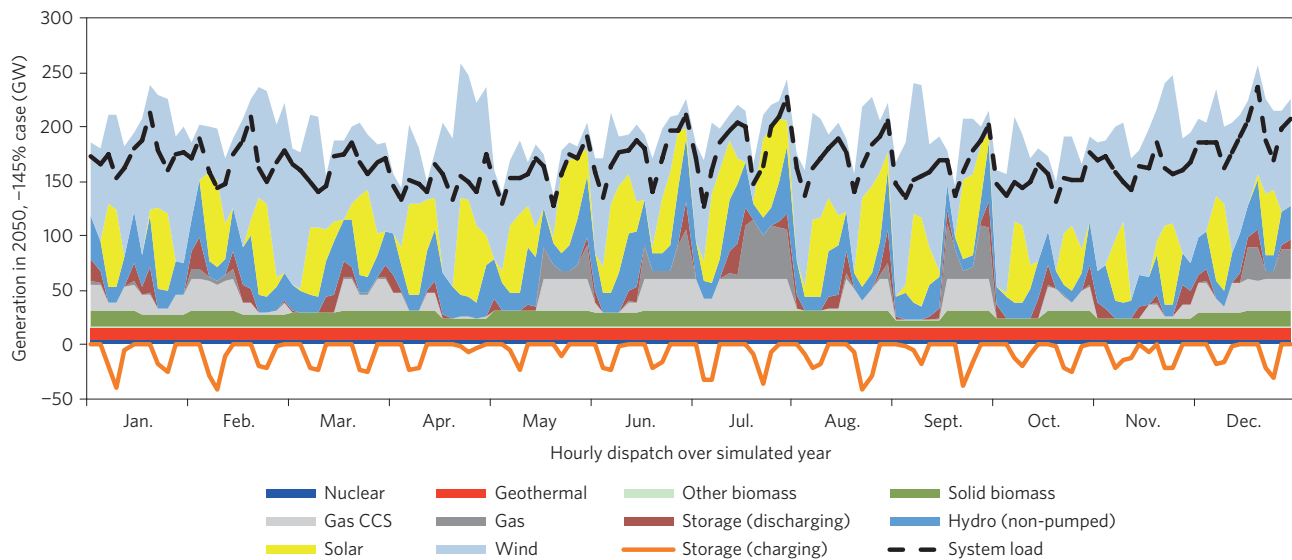
Figure 3 | Hourly dispatch in 2050 in the –145% case. Power system dispatch is shown in sampled hours from two days (peak and median day) each month between January–December. With the exception of BECCS, dispatch is similar between the –86% No Biomass and –145% case (Supplementary Fig. 9). Low-carbon scenarios without BECCS and carbon-negative scenarios with BECCS ultimately result in similar deployment of gas and renewable generation. ‘Other Biomass’ includes both liquid and gaseous biomass supplies.
