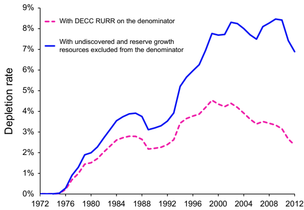
Fig. 1. Historical depletion rates for the UK with different depletion rate denominators.
