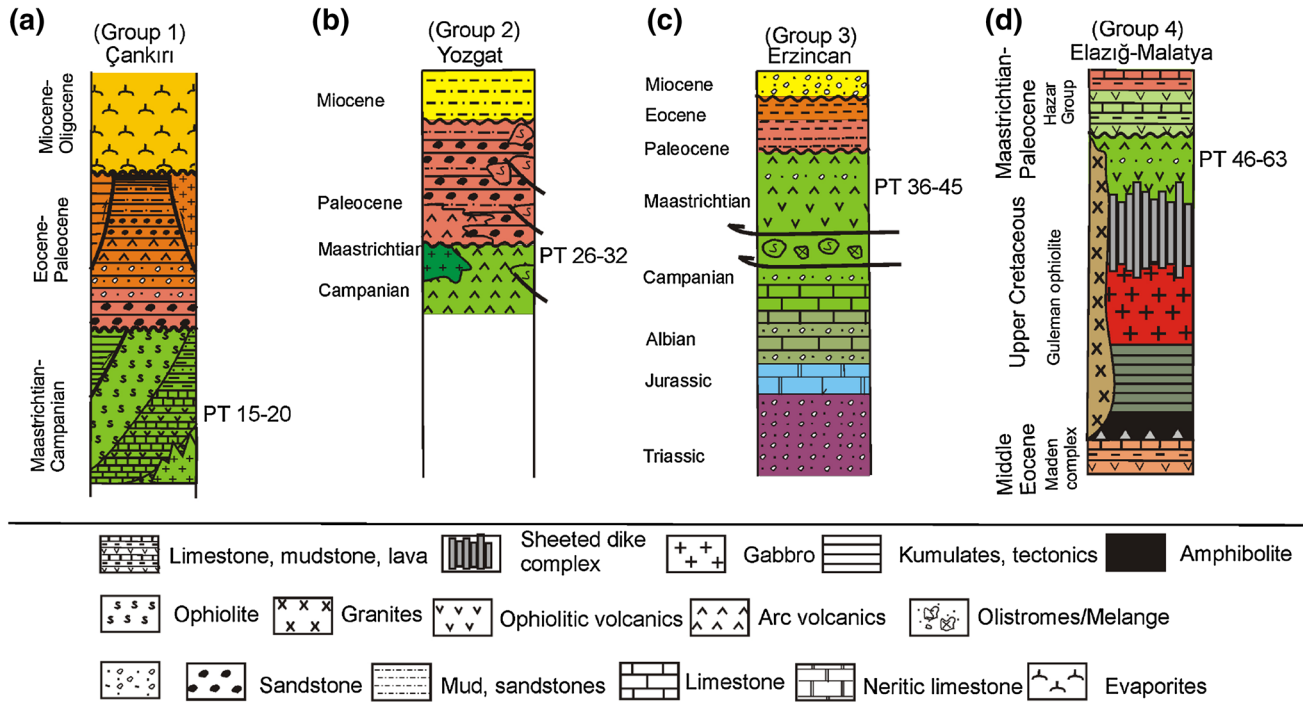
Fig. 3 Generalized stratigraphic columnar sections showing the sampling sites in a Çankırı (Kaymakçı et al. 2009; Tüysüz et al. 1995), b Yozgat (Erdoğan et al. 1996), c Erzincan (Rice et al. 2009) and d Elazığ-Malatya (Parlak et al. 2009)
