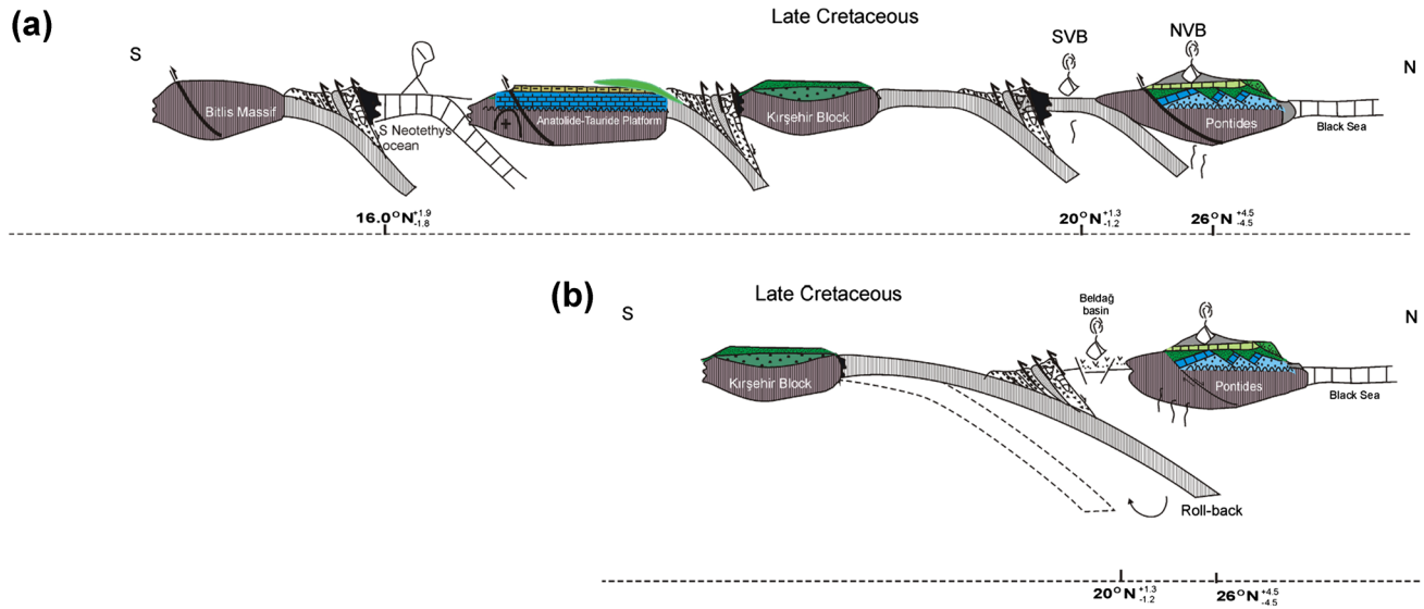
Fig. 10 The paleo(geographic) position of the Pontides and the Southeast Taurides in the Late Cretaceous showing a two subduction zone b slab roll-back process in the Pontides
